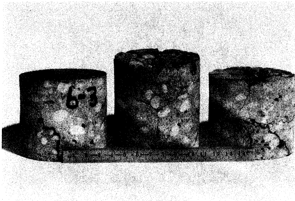
Figure 4. Cores removed from slabs repaired by injection.
