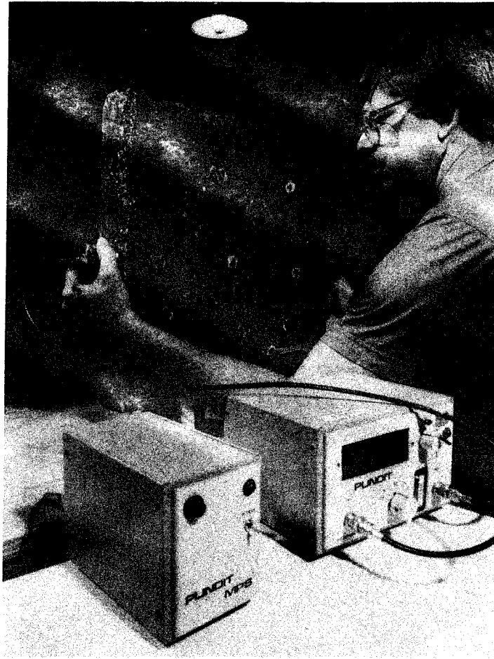
Figure 3. Ultrasonic pulse velocity test.
