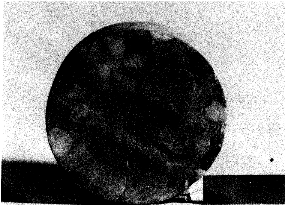
Figure 5. Splitting tensile strength test specimen after failure.
