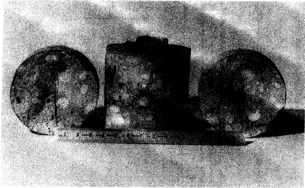
Figure 7. Cores removed from slab repaired by impregnation and injection (darkened areas around cracks indicate polymer impregnated concrete).
