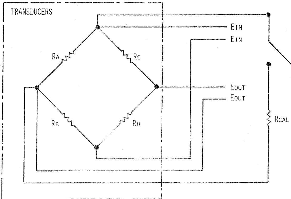
FIGURE B3. STRAIN GAGE TRANSDUCER WITH REMOTE "SHUNT CALIBRATION" CAPABILITY
