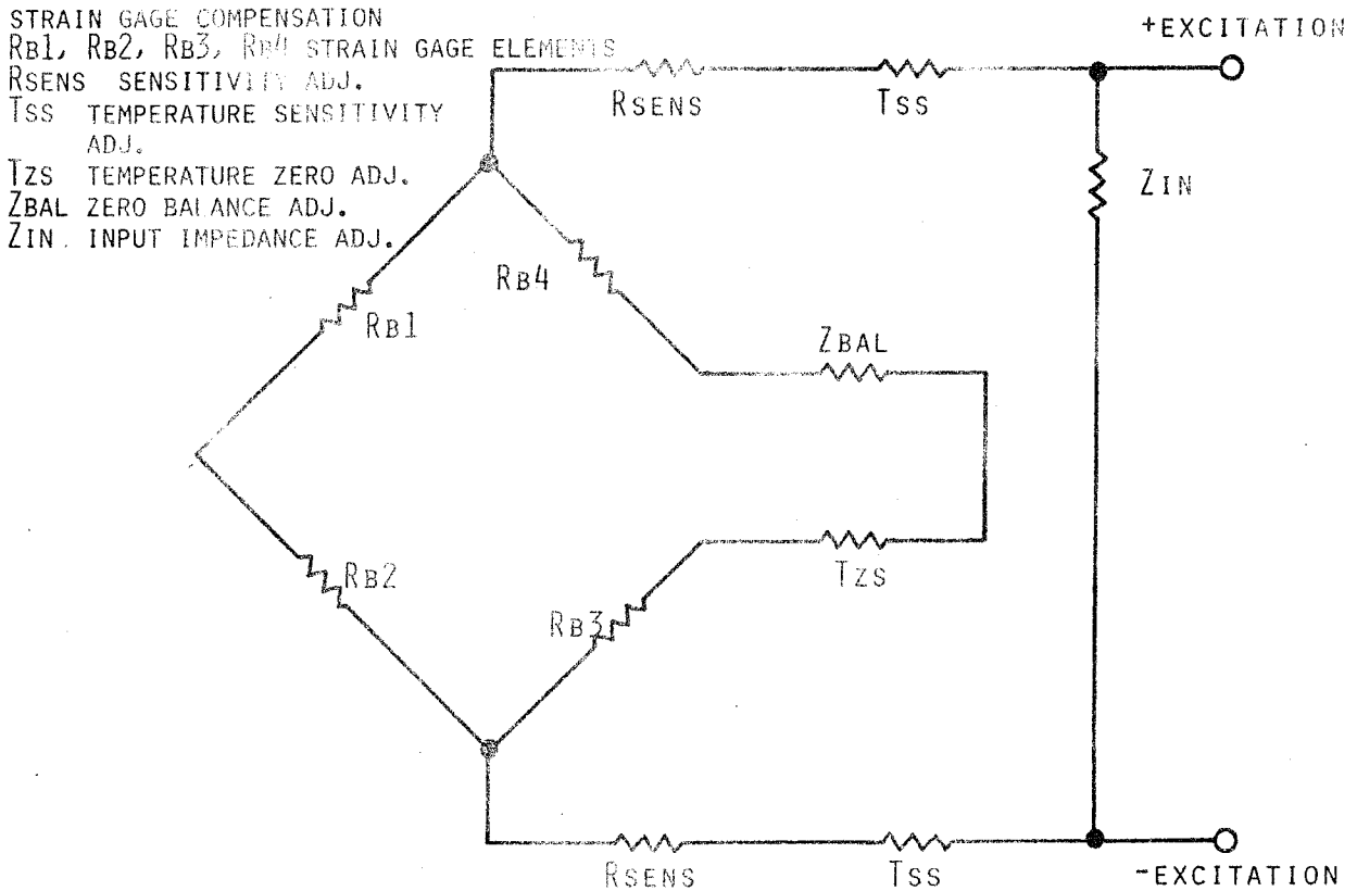
FIGURE B1. STRAIN GAGE COMPENSATION
