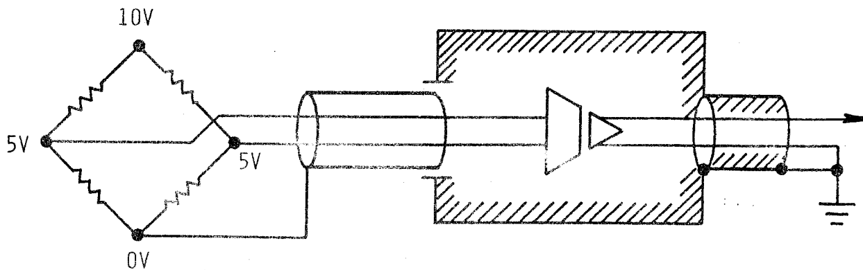
FIGURE 10. EXCITATION VOLTAGE AS A COMMON-MODE SIGNAL
