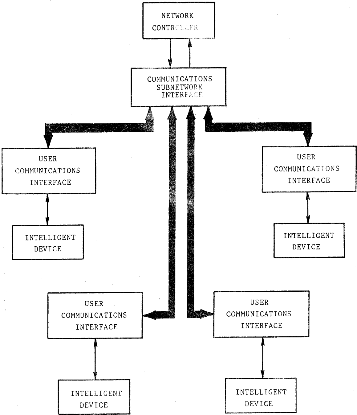
FIGURE 12. STAR CONFIGURATION
