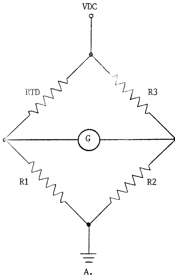
FIGURE 4. THE RTD IN APPLICATION
