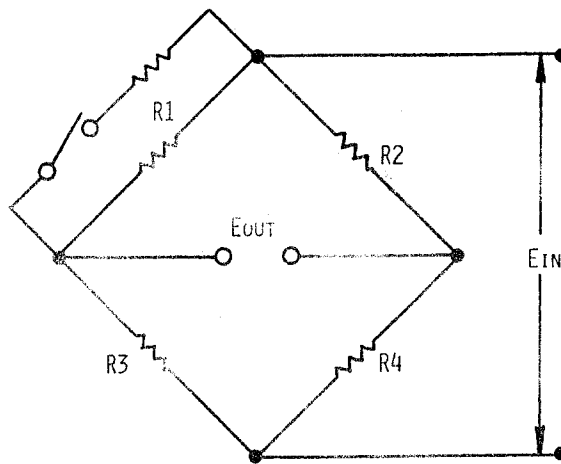
FIGURE 2. WHEATSTONE BRIDGE CIRCUIT
