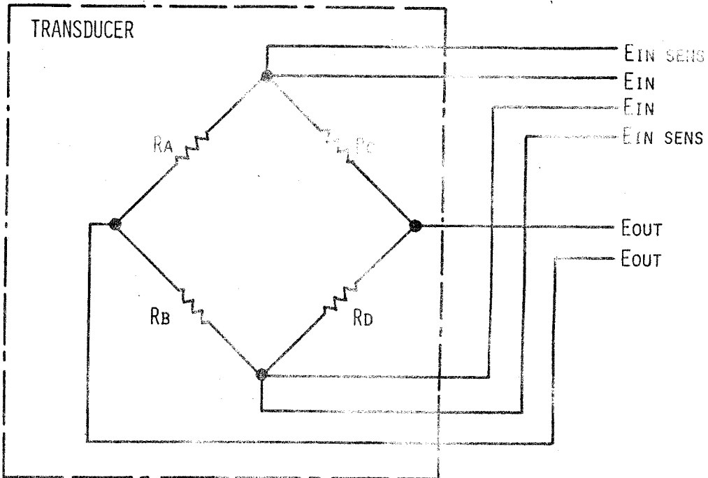
FIGURE B2. STRAIN GAGE TRANSDUCER WITH BRIDGE VOLTAGE SENSING CAPABILITY
