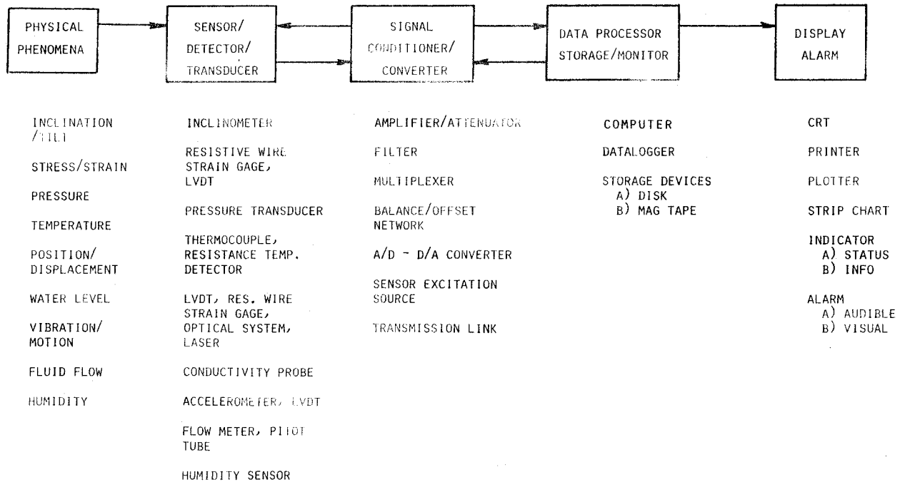
FIGURE 1. TYPICAL AUTOMATED INSTRUMENTATION/DATA ACQUISITION SYSTEM (EXAMPLES ARE LISTED UNDER EACH BLOCK.)
