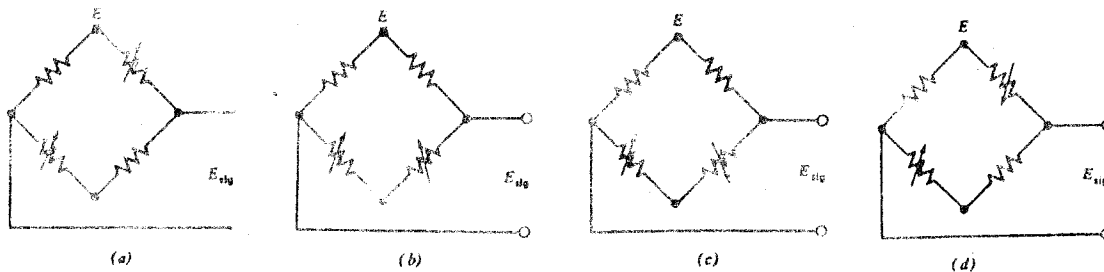
FIGURE B4. VARIOUS TWO-ACTIVE ARM BRIDGE CONFIGURATIONS: (A) SIGNAL ENHANCEMENT; (B) SIGNAL CANCELLATION; (C) SIGNAL ENHANCEMENT; (D) SIGNAL CANCELLATION
