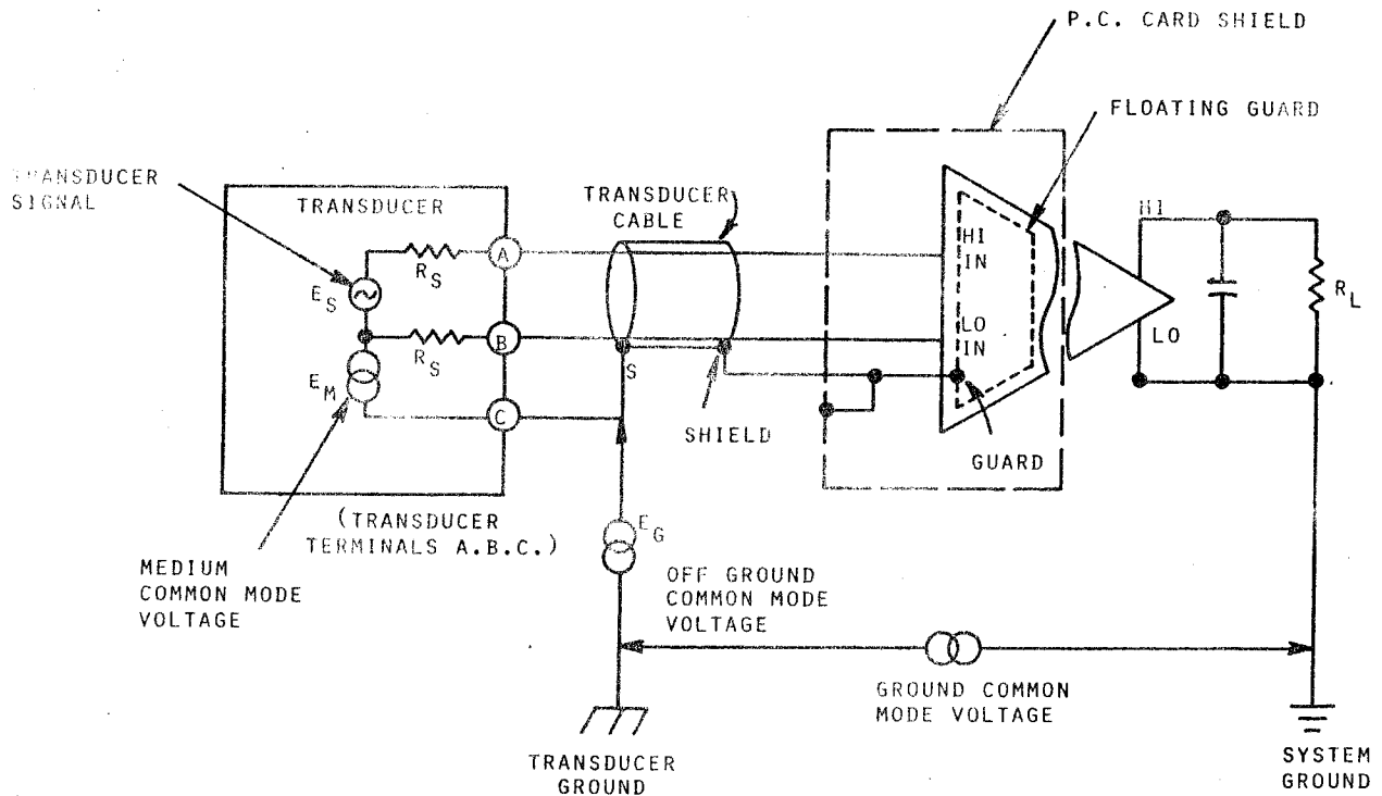
FIGURE 7. TRANSDUCER-AMPLIFIER INTERCONNECTION
