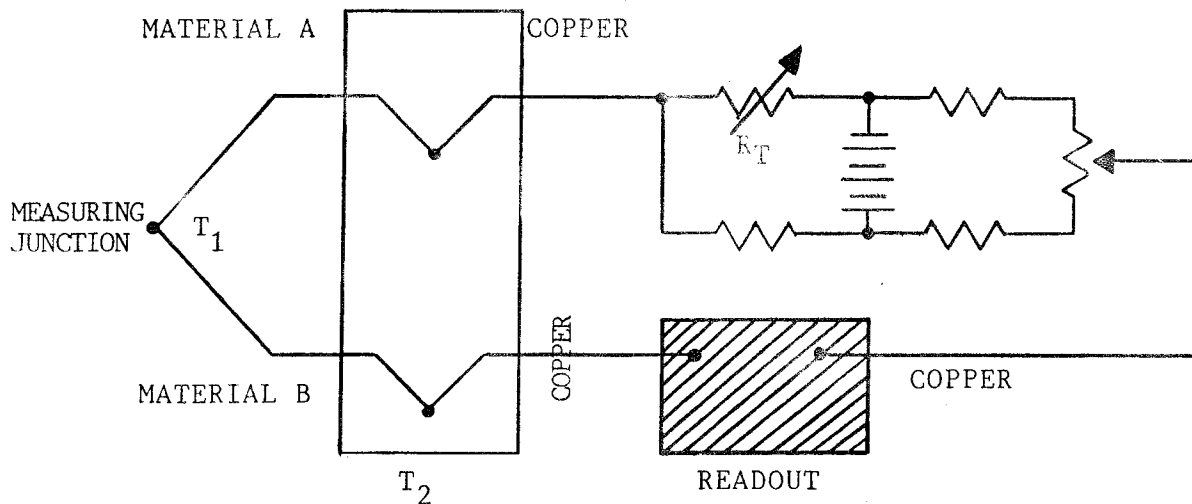
FIGURE 3. THERMOCOUPLE ELECTRICAL REFERENCE JUNCTION
