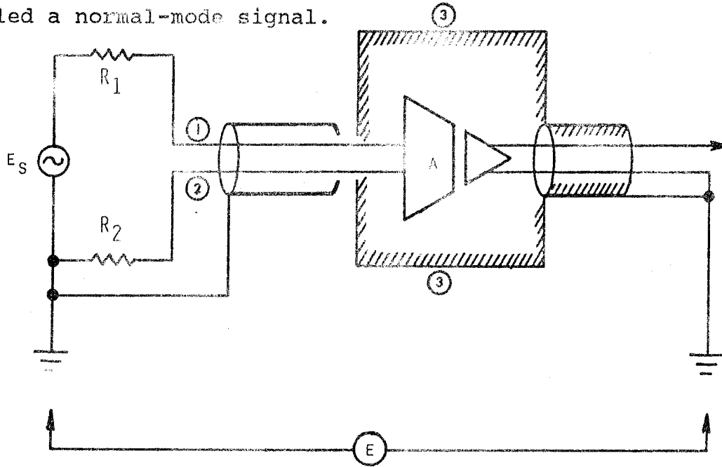
FIGURE 9. A SINGLE AMPLIFIER TO REJECT SIGNAL E
