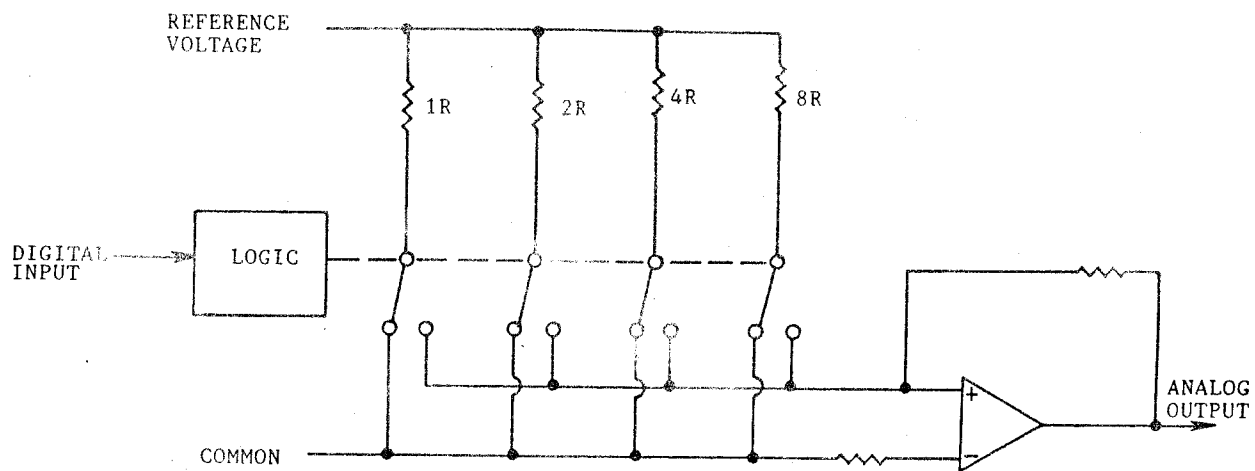
FIGURE 8. TYPICAL DIGITAL-TO-ANALOG NETWORK
