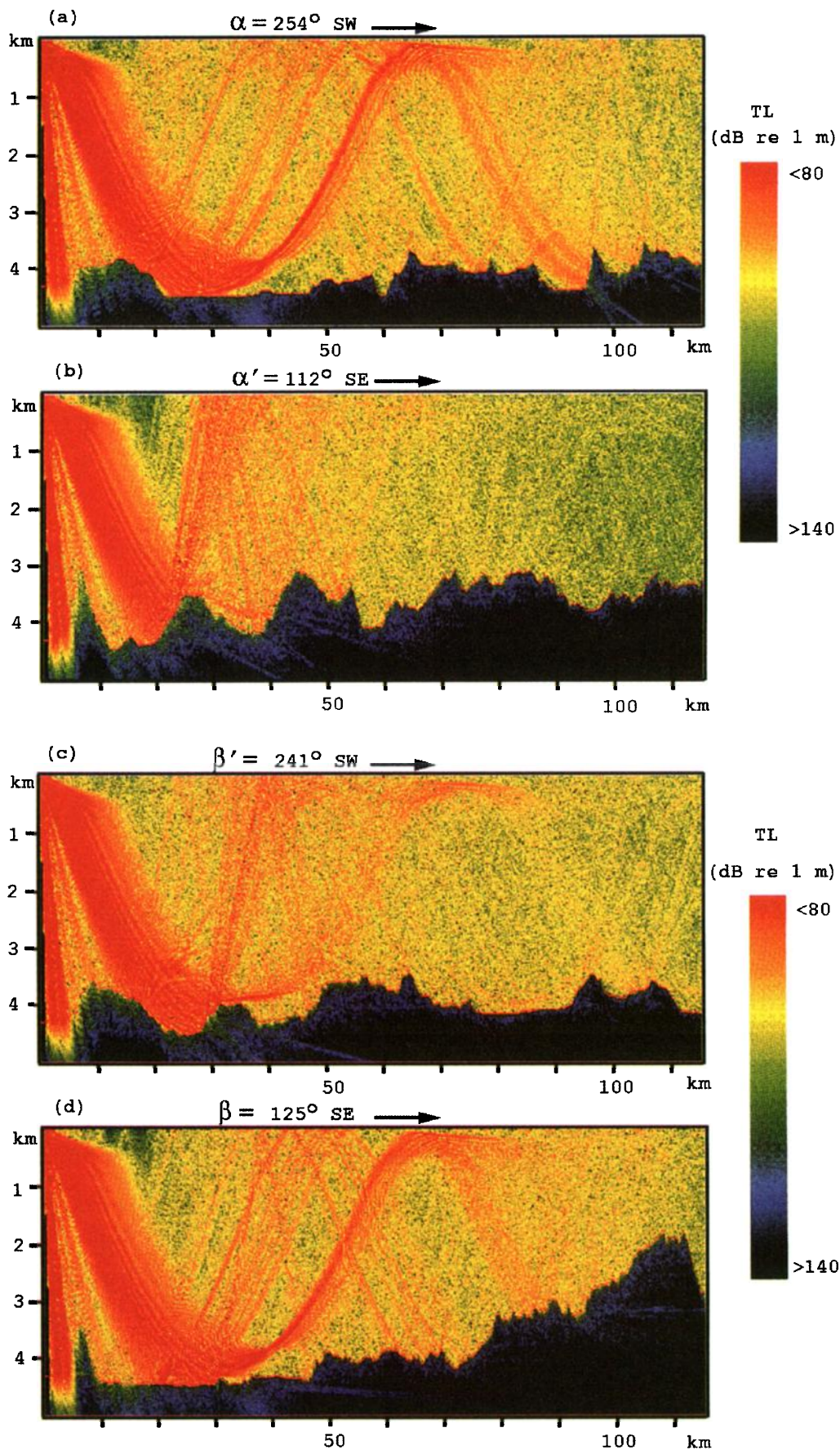
FIG. 6. Transmission loss (TL) for range-dependent cross sections of the ocean along the radials depicted in Fig. 5. In each case, propagation to \frac{1}{2} CZ is partially or fully blocked in the direct path for one member of each symmetric pair, and is clear for the other. (The source is modeled with the wide-angle PE as an untapered ten-element vertical array, shown in Fig. 2, steered to a 6^\circ depression angle.) In general, backfacing scarps are insonified by the source beam while forward-facing scarps are in the acoustic shadow. Stronger backscatter is therefore expected from backfacing scarps.
