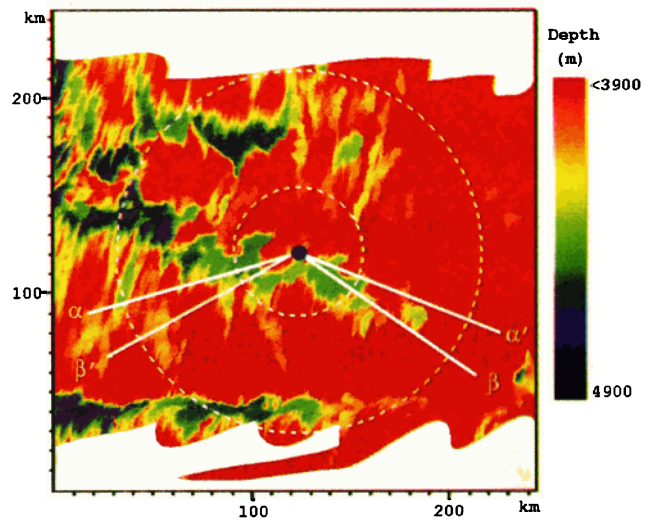
FIG. 5. Positive excess depth with respect to the conjugate depth of the source-array center. The white dotted lines indicate the approximate location of the source-beam vertex at 1\frac{1}{2} CZ ranges from central observation R7E15 which is indicated by a dark dot. The solid white lines indicate radial pairs (\alpha, \alpha') and (\beta, \beta') symmetric about the array axis.
