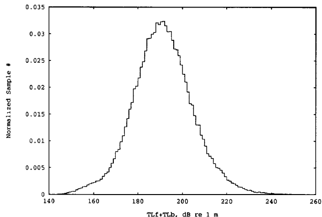
FIG. 11. A histogram of wide area TL_f+TL_b for observation R7E15 with mean level 191 dB re: 1 m, median 191 dB re: 1 m, and standard deviation 14 dB. Two-way TL values corresponding to waterborne sites comprise the lower tail of this distribution.
