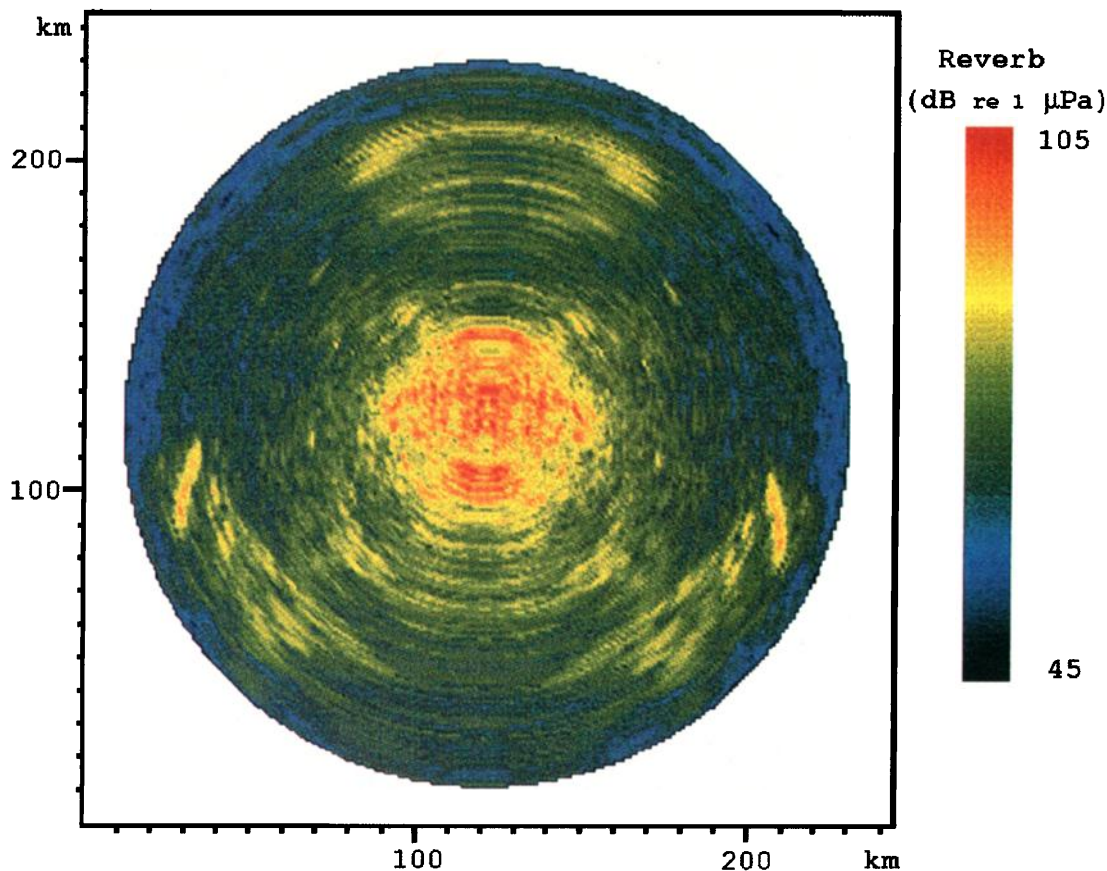
FIG. 7. A reverberation map for observation R7E15. Highest level returns occur within the direct path and at 1\frac{1}{2} CZ range. All returns are mirrored about the array axis, roughly 183^\circ azimuth, due to right-left ambiguity. Poor resolution due to endfire occurs within roughly \pm 30^\circ of the array axis.
