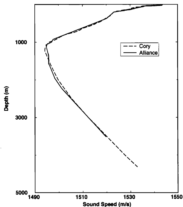
FIG. 1. Sound-speed profiles measured by the RV CORY CHOUDEST via XBT on J201 20:02 Z at 26° 31' N 47° 9' W (near the Easternstar) and the RV ALLIANCE via CTD on J199 18:12 Z at 26° 34' N 47° 59' W (near the Westernstar). The close agreement between the profiles over significant spatial and temporal separations strongly supports the range/time-independent approximation used for the water-column sound-speed structure in this analysis. Archival data are used below 1830-m depth for the XBT.
