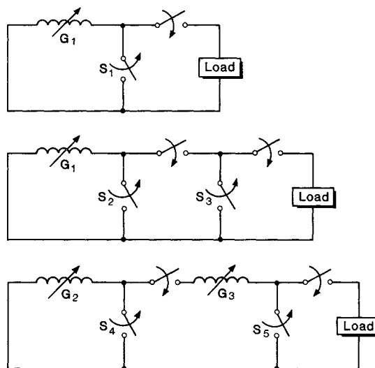
Fig. 1. Exemplary power conditioning circuits.
