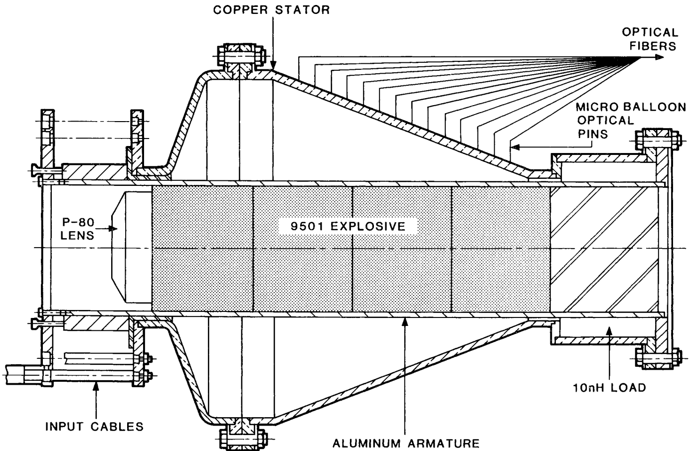
Fig. 2. Simplified drawing of the coaxial generator used in the tests.
