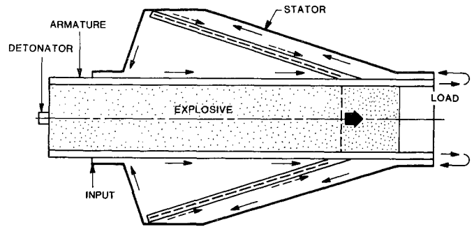
Fig. 1. Operation of the sweeping-wave coaxial generator. The dashed lines represent the positions of the armature and detonation front near the end of the run.
