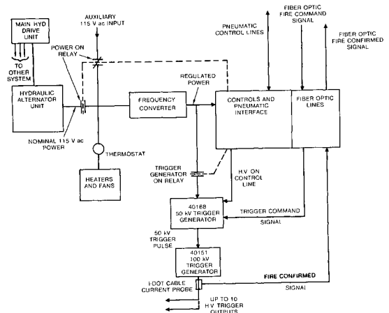
Fig. 2 Block Diagram
