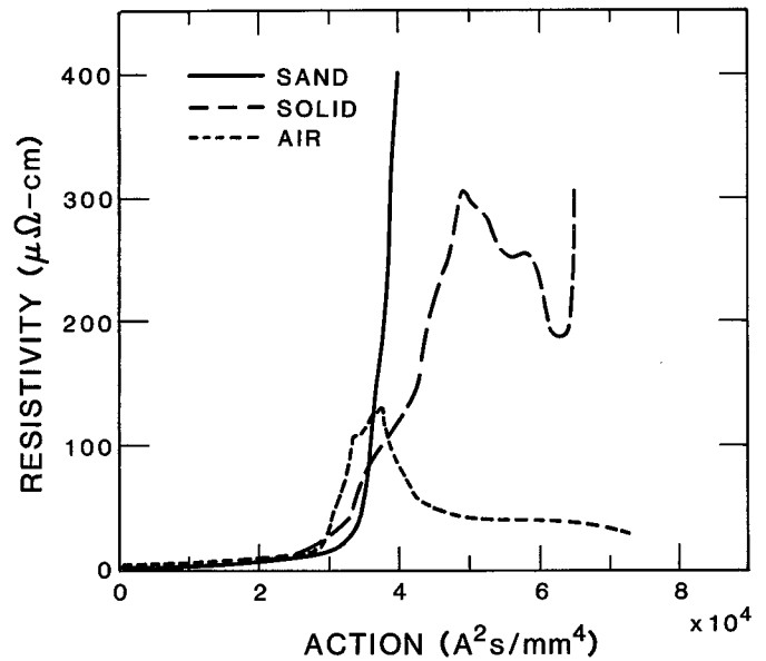
Fig. 5. Effect of Surrounding Material, Aluminum Fuse
