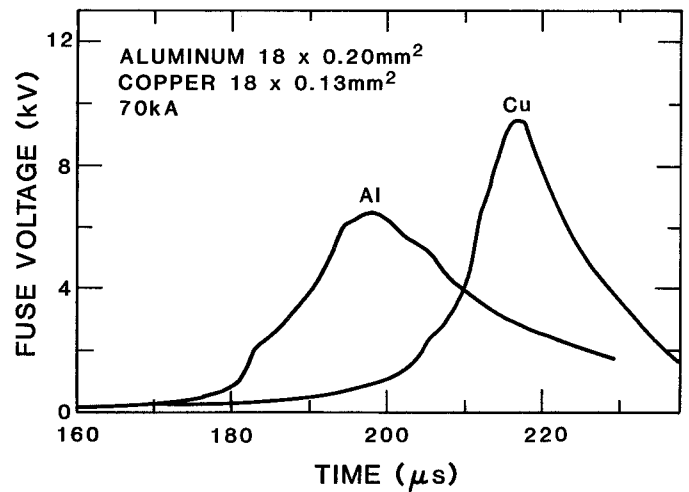
Fig. 10. Comparison of Copper and Aluminum Fuses
