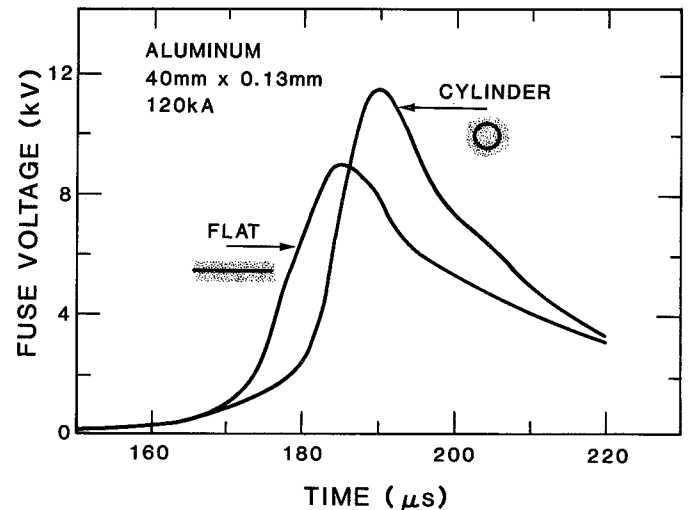
Fig. 6. Effect of Fuse Geometry on Switching
