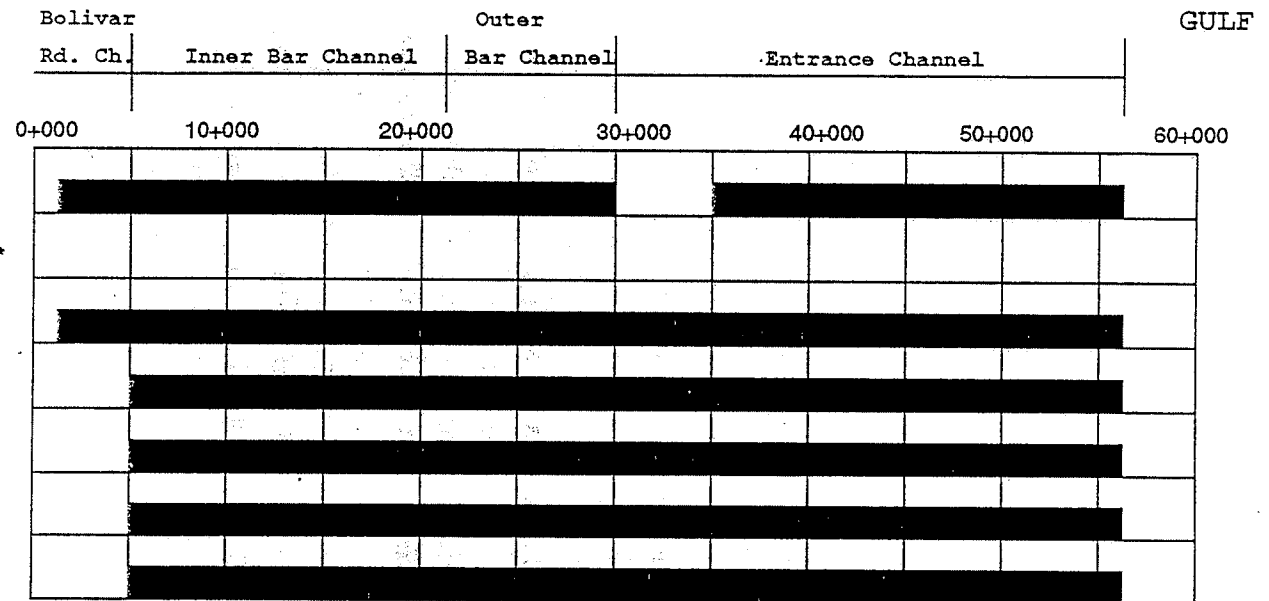
FIGURE 5 MAINTENANCE DREDGING OF THE GALVESTON HARBOR CHANNEL
