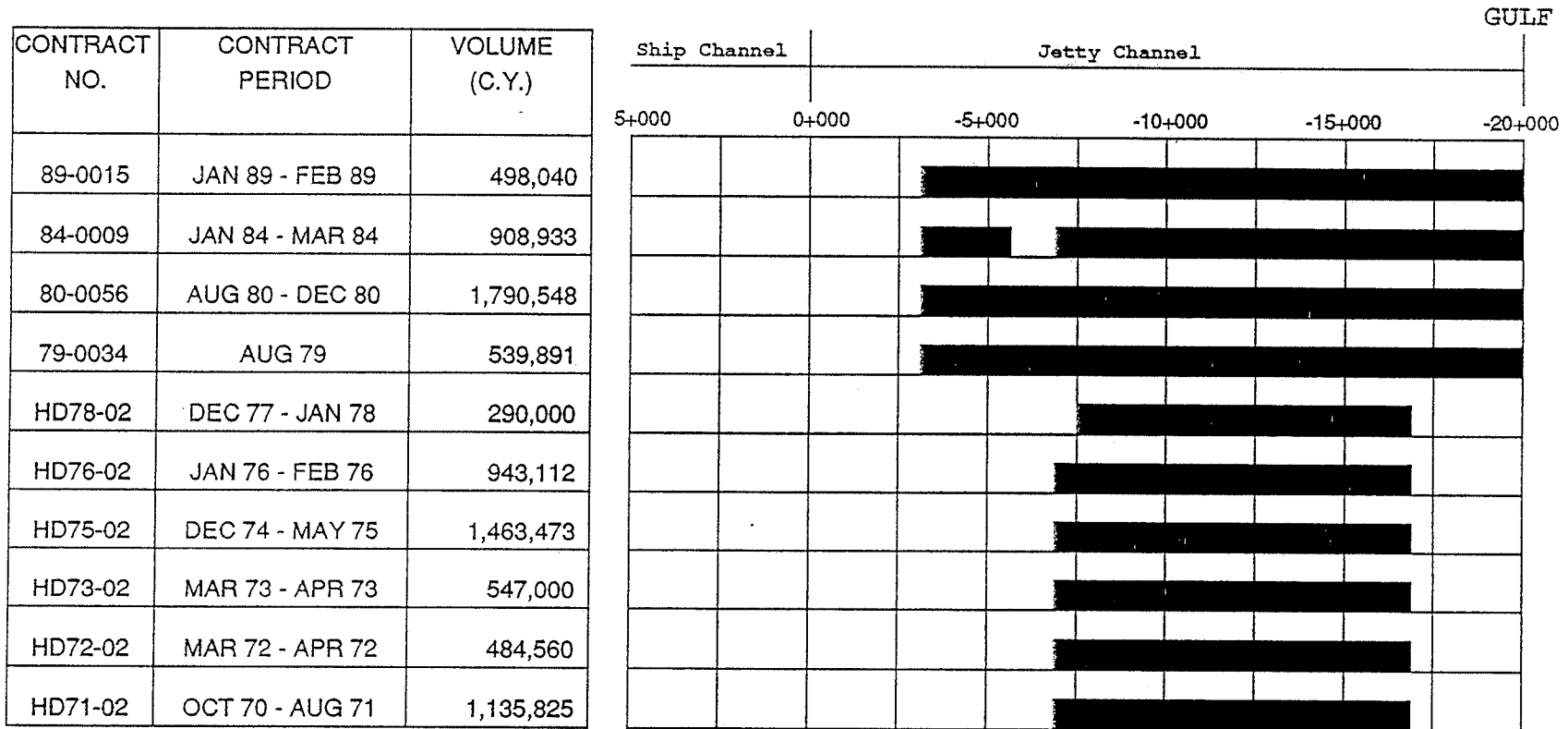
FIGURE 11 MAINTENANCE DREDGING OF THE ENTRANCE OF MATAGORDA SHIP CHANNEL
