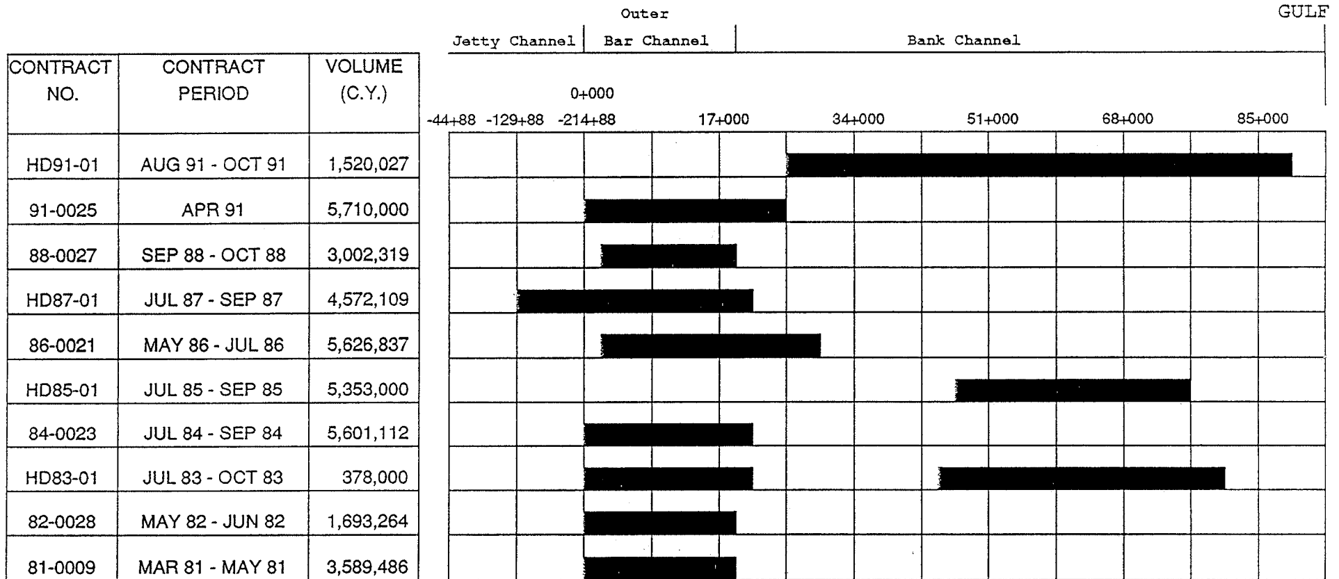
FIGURE 3 MAINTENANCE DREDGING OF THE ENTRANCE OF SABINE-NECHES WATERWAY
