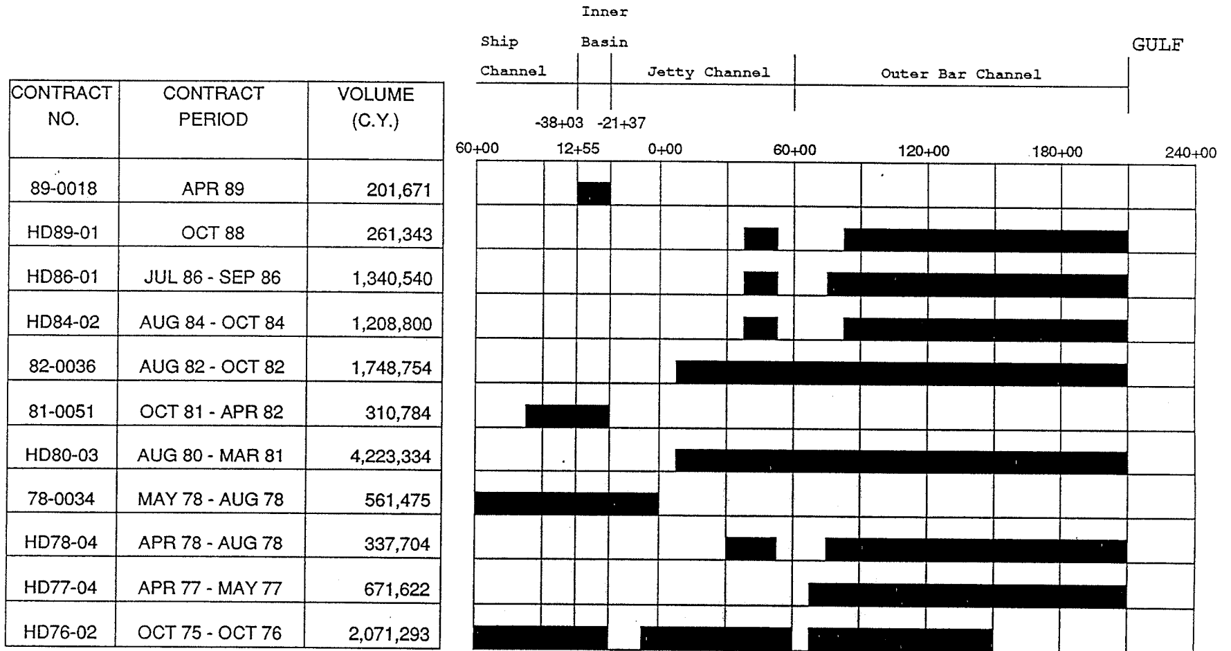
FIGURE 13 MAINTENANCE DREDGING OF THE ENTRANCE OF CORPUS CHRISTI SHIP CHANNEL
