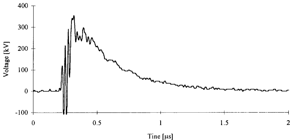
Figure 7. Output Voltage into 5 \Omega from +/- 50 kV Charge of Four Stage Marx
