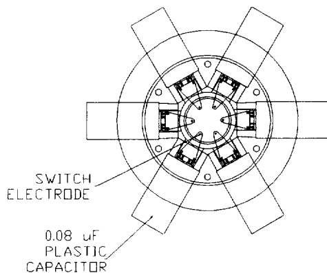
Figure 2a. Axial View of Single Marx Stage
