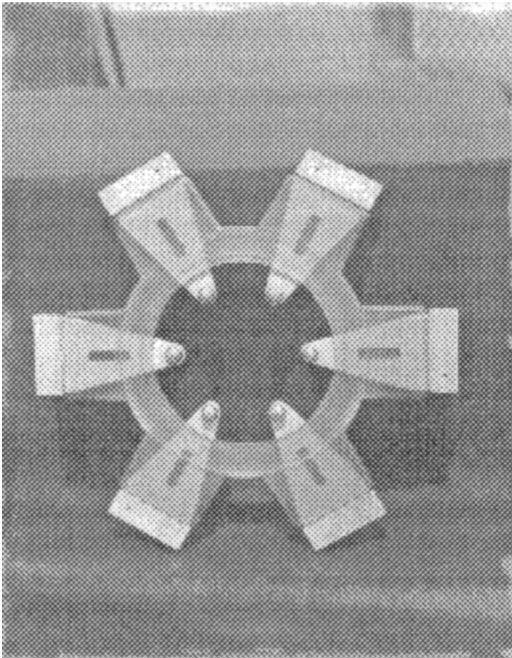
Figure 4. Completed Cast Switch Element
