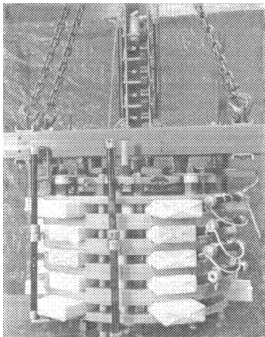
Figure 1. Assembled Four Stage Compact Marx
