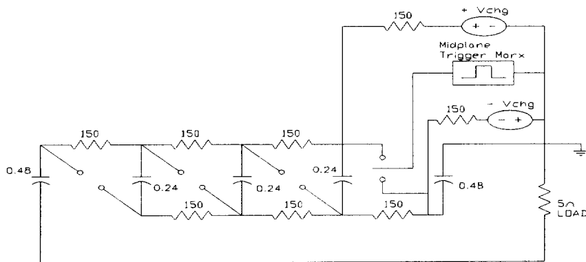
Figure 3 Circuit Diagram of Bipolar Four Stage Marx
