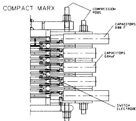
Figure 2b. Radial Cross Section View of Four Stage Marx
