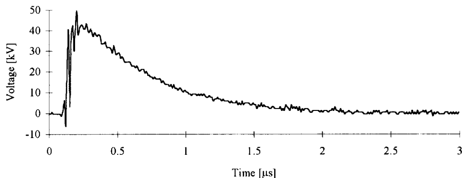
Figure 5. Output Voltage into 5 \Omega from \pm 20 kV Charge of Two Stage Marx
