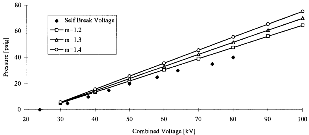
Figure 6. Static breakdown and operating pressures for the Compact Marx.
