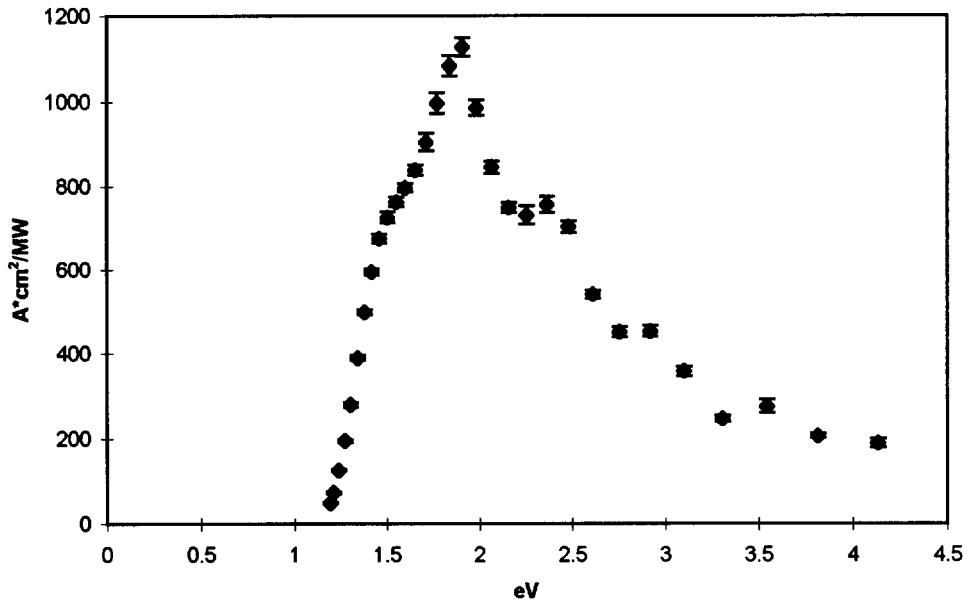
Figure 1. Average response and 1- \sigma error bars for 49 HS-1 silicon diodes.
