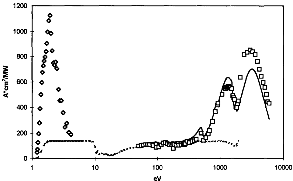
Figure 3. HS-1 silicon diode spectral response . Overlaid curves show two different physical models of behavior.
