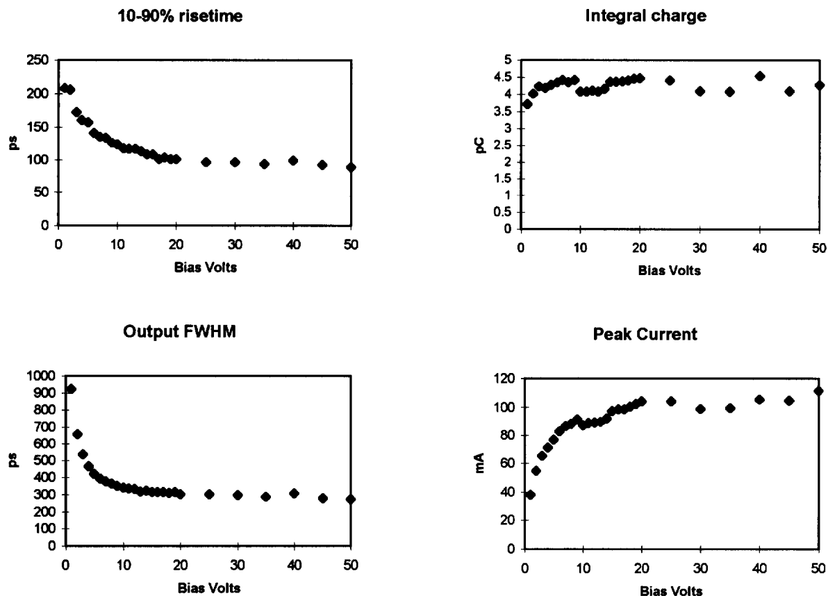
Figure 2. HS-1 silicon diode response as a function of bias voltage for a fast visible laser input pulse.
