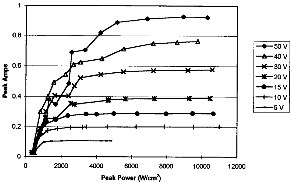
Figure 5. HS-1 silicon diode saturation response as a function of bias voltage.
