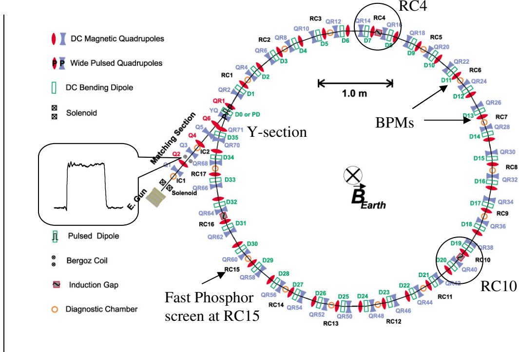
Fig. 3. 22. Lattice optics diagram with the RC4 induction-cell and RC10 wall current monitor circled. An example rectangular beam current profile is shown in the caption. Two of the 14 available BPMs are labeled in the figure as well as the placement of the fast phosphor screen at RC15.
