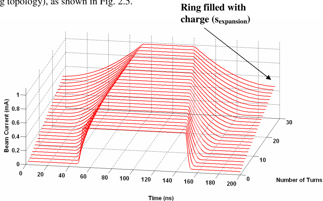
Fig. 2. 5. Analytical beam current calculation of the head and tail evolution, assuming an injected beam length that is longer than \frac{1}{3} the total lap time.
