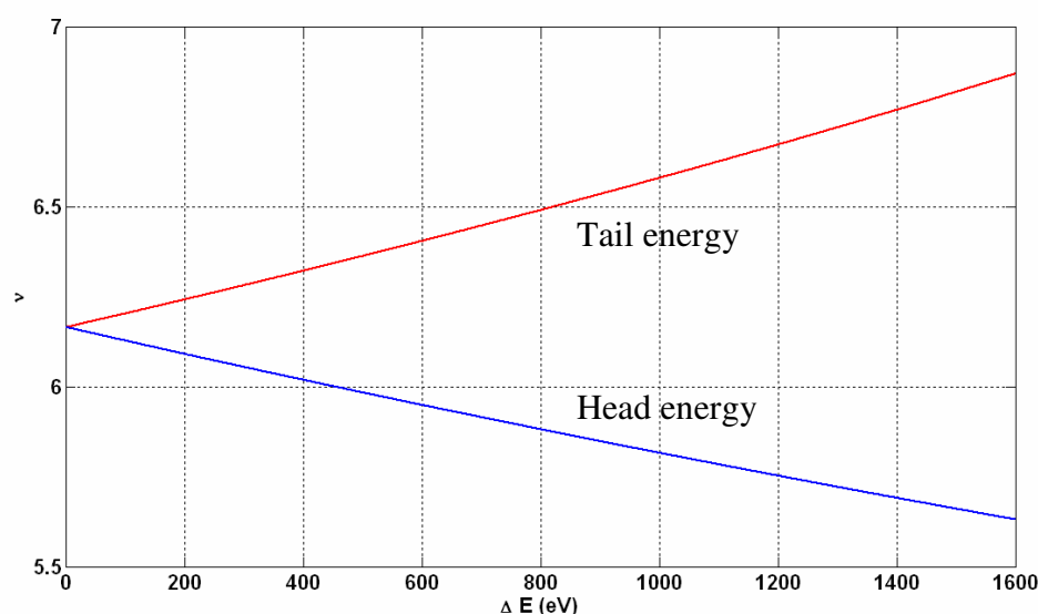
Fig. 2. 11. Tune dependence on peak head and tail energy.
