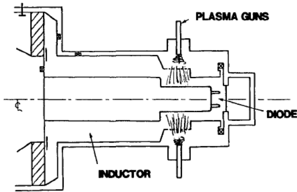
Fig. 1. Schematic of the Gamble II system.
