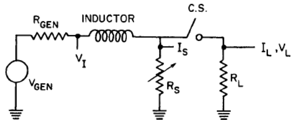
Fig. 3. Simplified circuit model.
