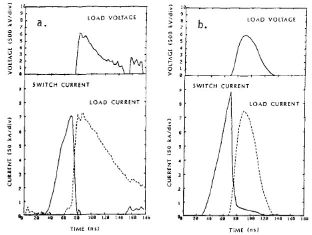
Fig. 2. (a) Gamble II PEOS results, (b) Computer model of Gamble II results.
