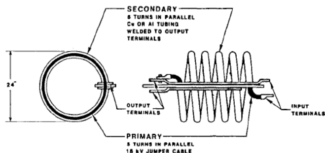
Figure 5. Pulse transformer
