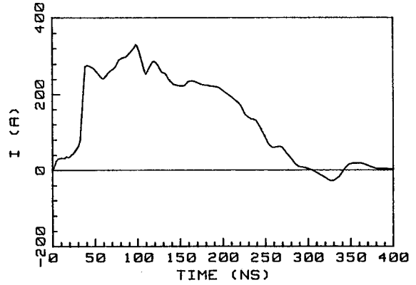
Figure 10. Current response of self-integrating magnetic field loop positioned in AURORA test cell as shown in Fig. 11a.
