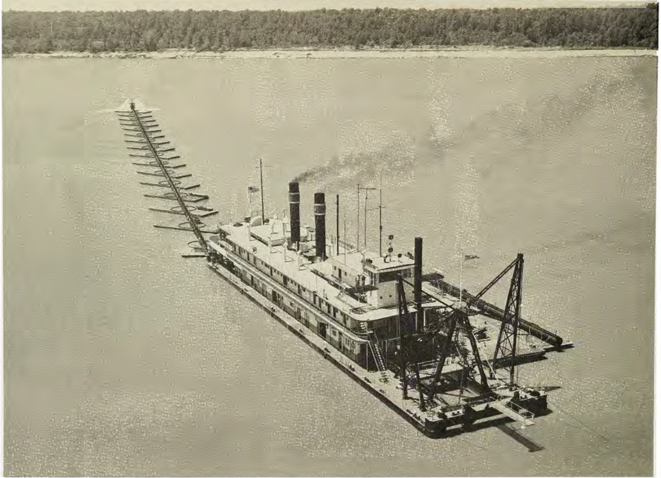
"Ockerson" at work dredging channel.
