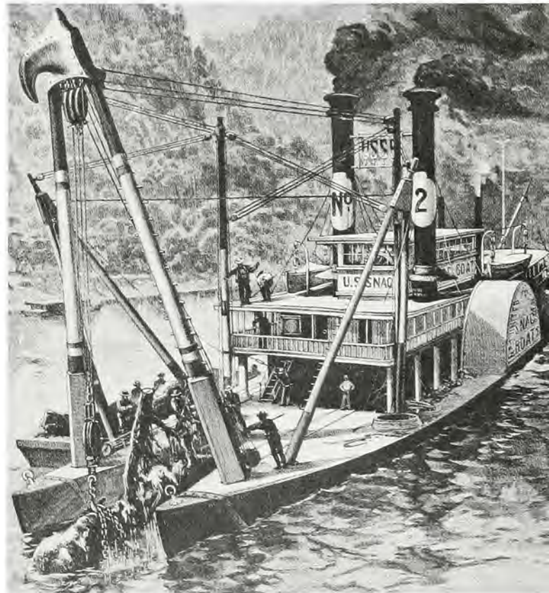
U. S. Snag Boat No. 2 is a slightly enlarged version of Capt. Shreve's original snag boat, the Heliopolis. Harper's Weekly, 1889.
