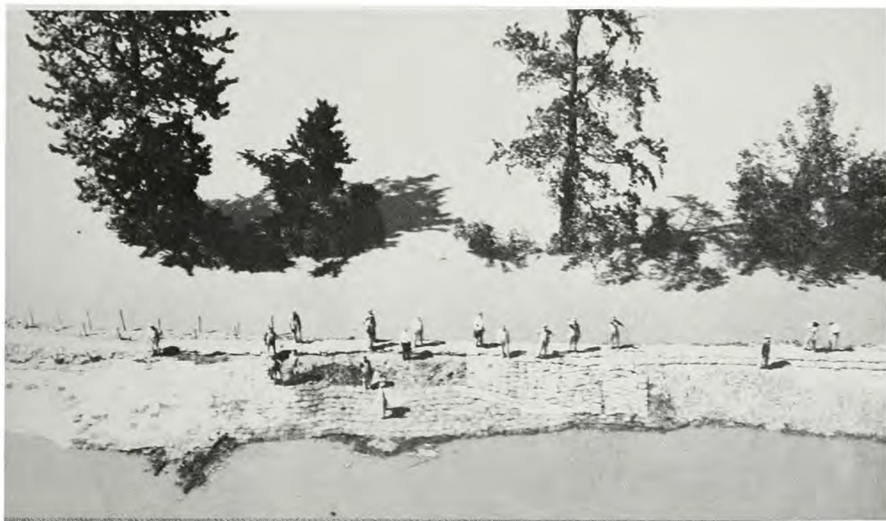
Men at work adding height and protecting the slope of an emergency levee at Booth's Point. May 29, 1943.
