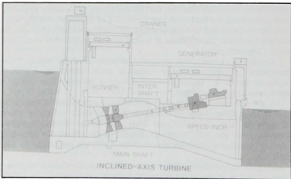
The division's Hydropower Design Branch determined that inclined-axis turbines were more economical than traditional designs.
