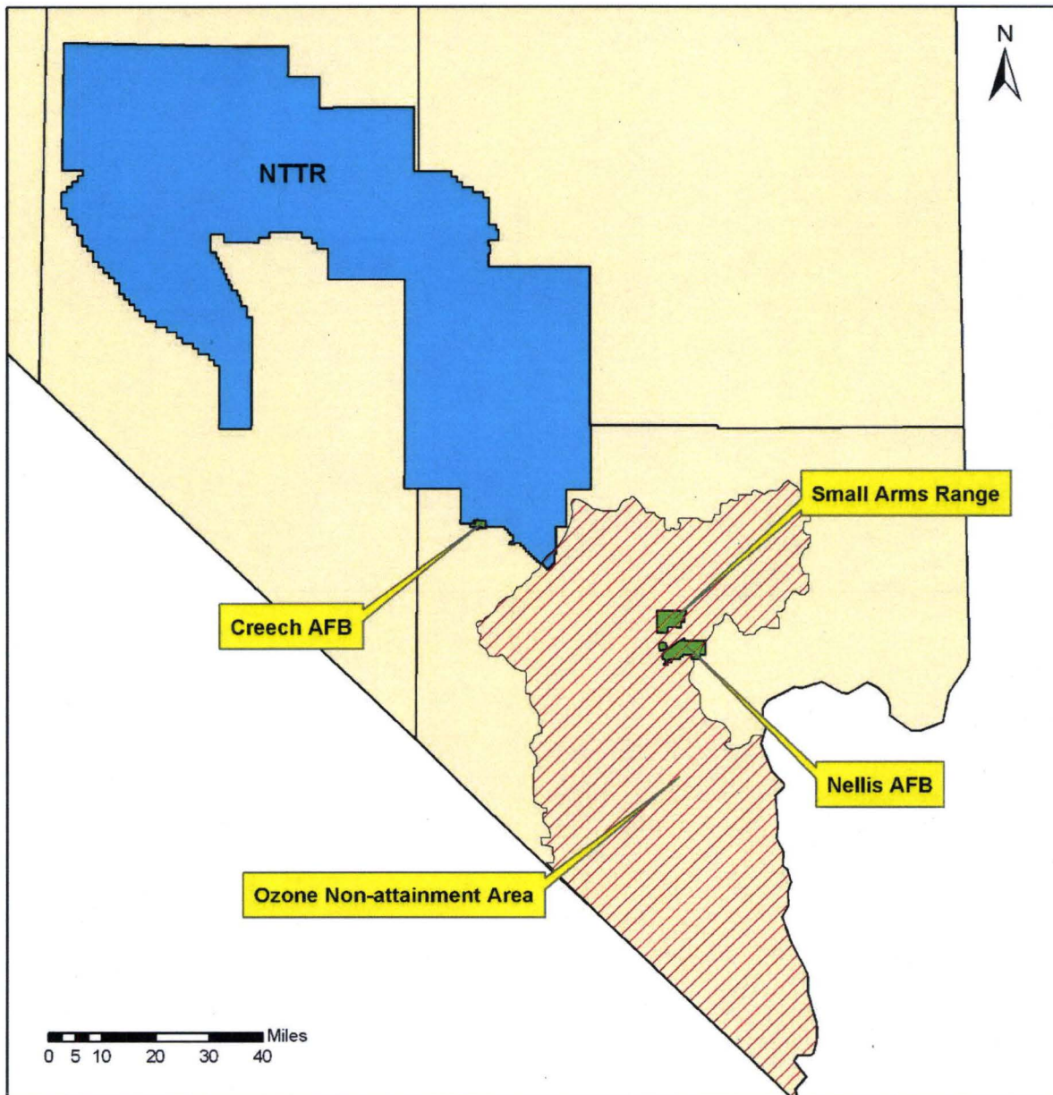
Figure 3.3. Ozone 8-hour non-attainment area at NTTR and NAFB.
