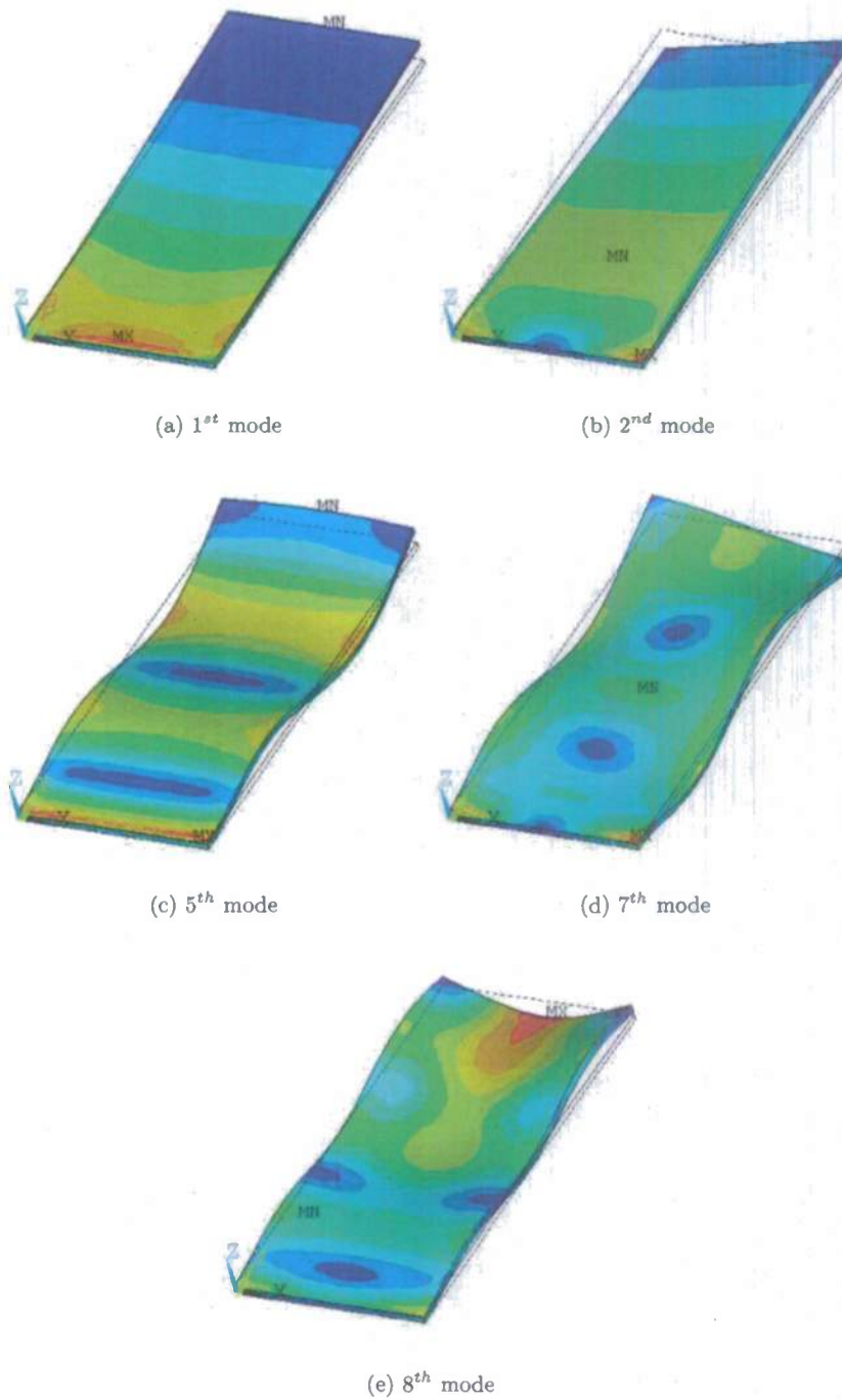
Figure 27: Plate structure: mode shapes and Von Mises modal strain fields.
