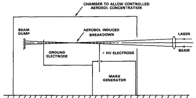
Figure 3. Arrangement for preparing channels in the atmosphere.
