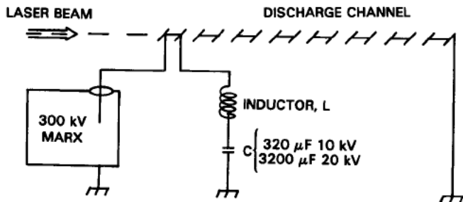
Figure 1. Schematic diagram of the apparatus for producing discharge channels with inductive isolation of the secondary bank.
