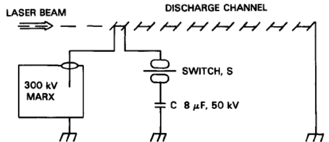
Figure 2. Schematic diagram of the apparatus for producing discharge channels with explosive switch isolation of the secondary bank.
