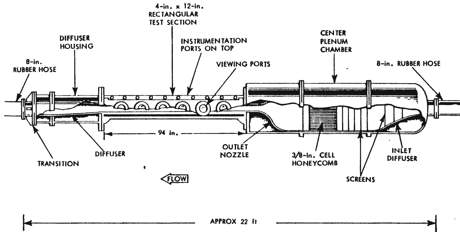
Figure 4 RECTANGULAR TEST SECTION ASSEMBLY
