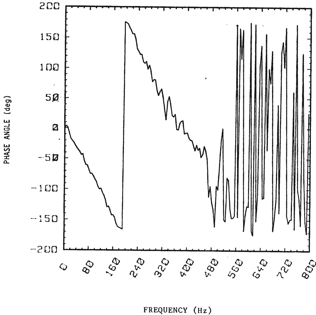
Figure 18a PHASE VELOCITY TRANSFER FUNCTION
