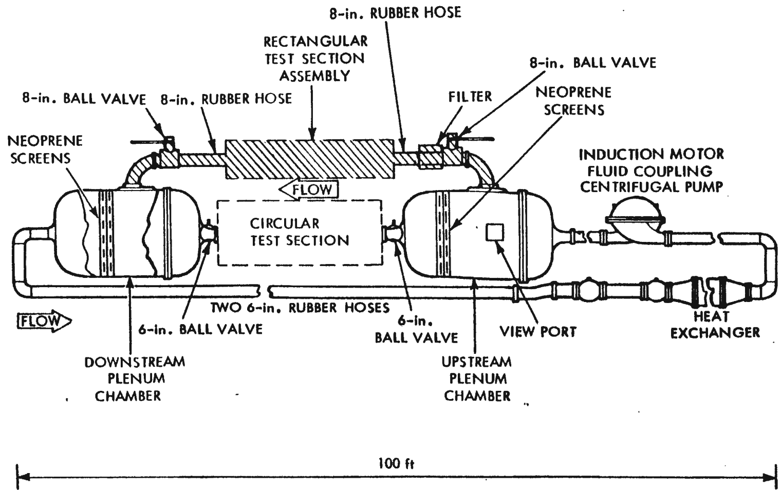
Figure 3 NUSC ACOUSTIC WATER TUNNEL
