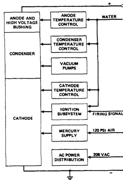
Fig. 2. Block Diagram of LMPVCS System
