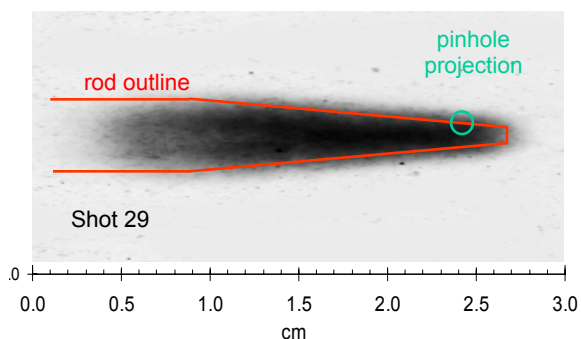
Figure 7. Pinhole camera image of 4-mm-OD anode.
