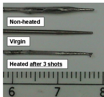
Figure 10. Comparison of non-heated (after one shot), virgin, and heated (after three shots) 1-mm-OD anodes.
