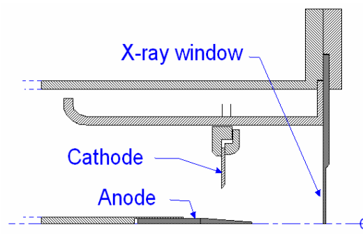
Figure 4. Geometry of the original HRS diode.
