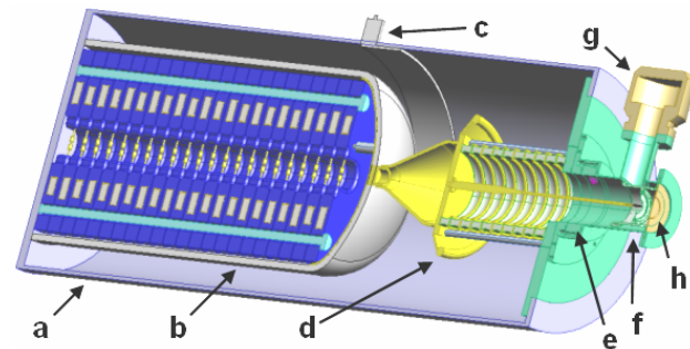
Figure 1. Diagram of the HRS indicating the (a) main body, (b) stacked Marx, (c) voltage monitor, (d) field shaper and stacked-ring insulator, (e) current monitor, (f) cylindrical diode, (g) vacuum pump, and (h) x-ray output window.
