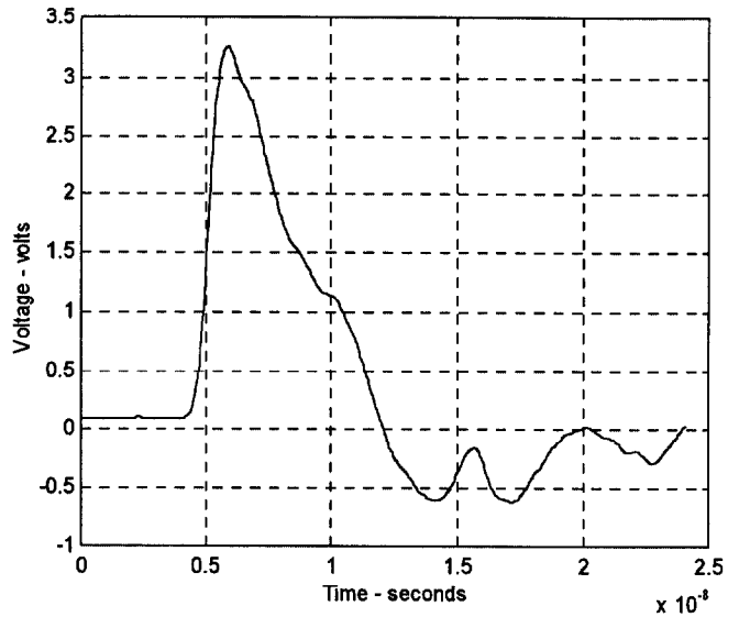
Figure 4. Typical Transmitted Pulse from 1.27-mm Vacuum Gap
