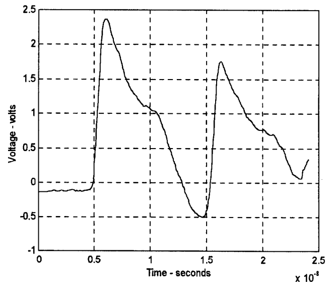
Figure 5. Typical Incident Pulse to 2.45-mm Vacuum Gap
