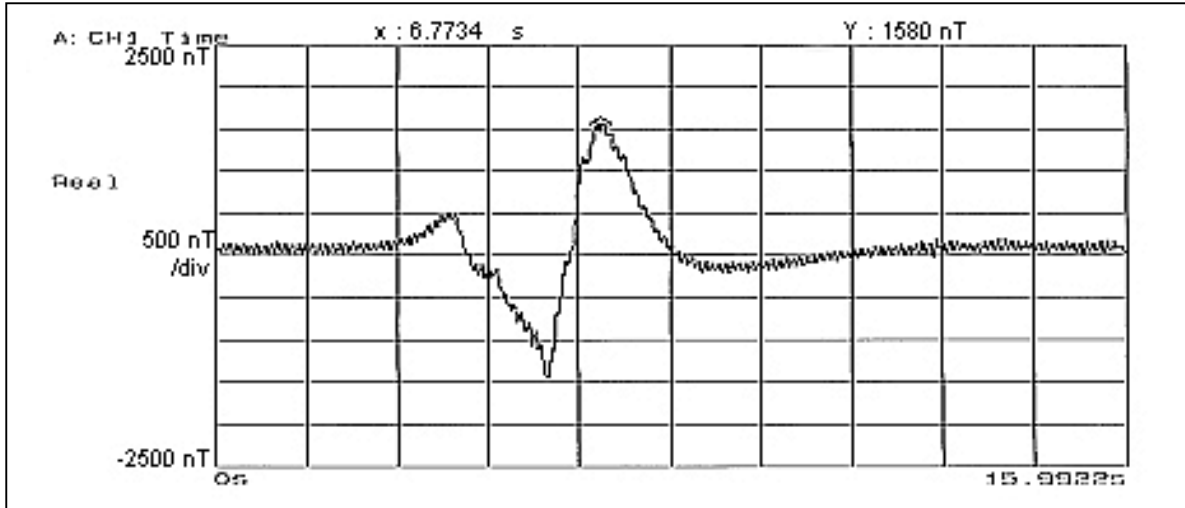
Figure 5-2. Magnetic signature shows the induced and onboard moments.
