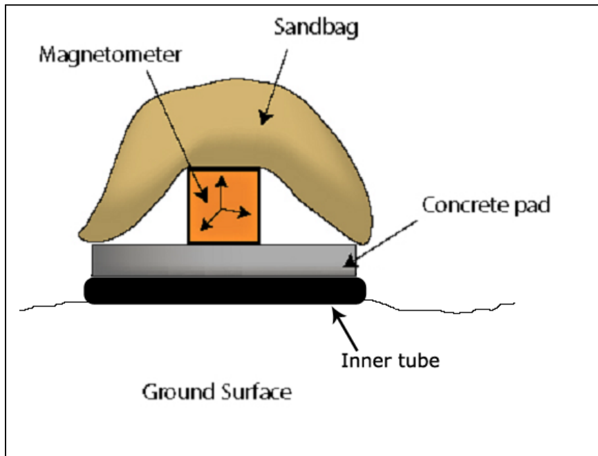
Figure 2-1. Magnetometer placement on the ground surface.
