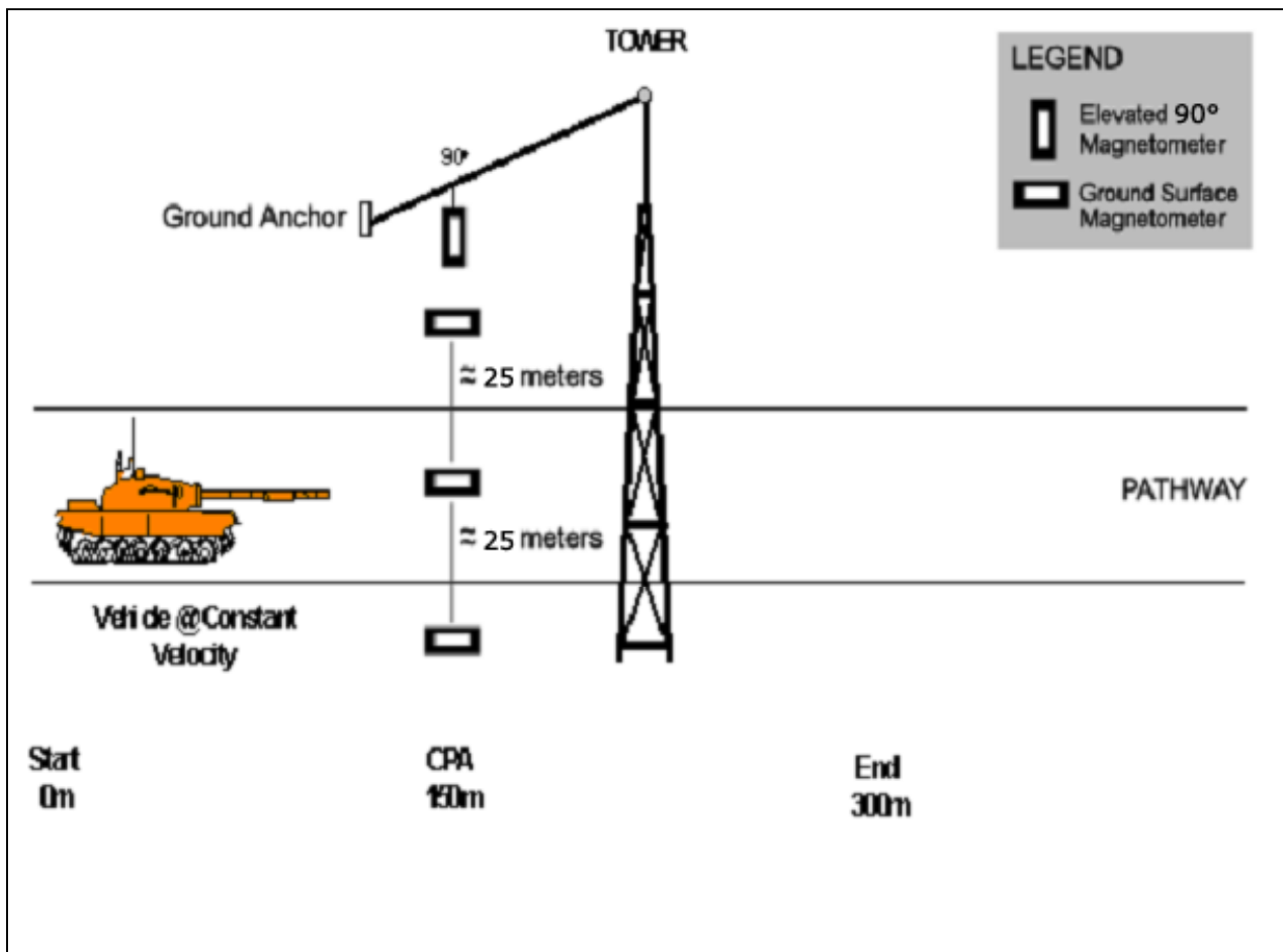
Figure 2-2. Magnetometer scenarios for a vehicular test track.
