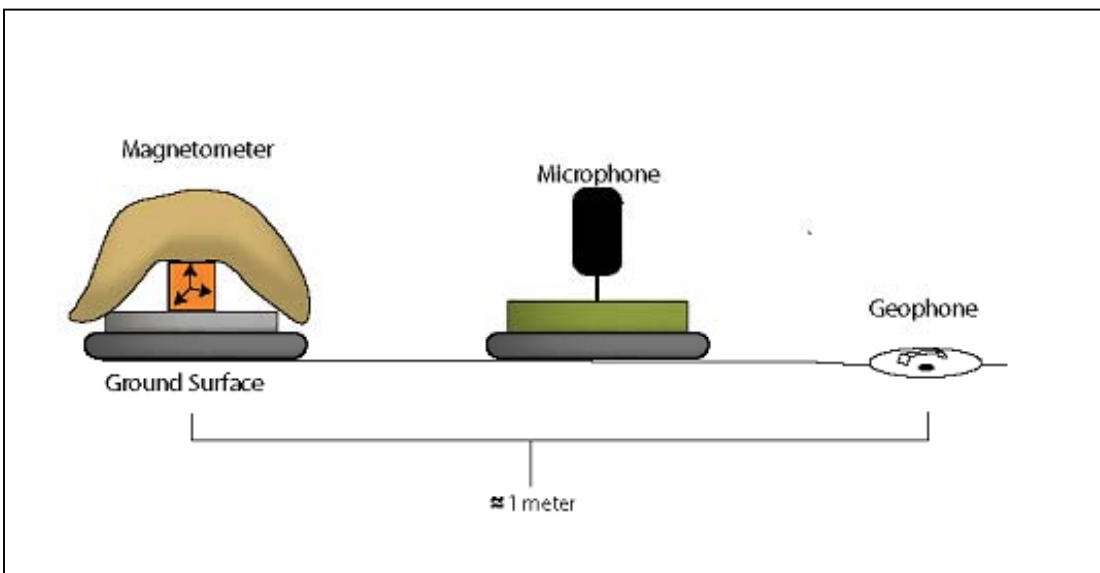
Figure 2-3. Collocation of SAM sensors in the field.
