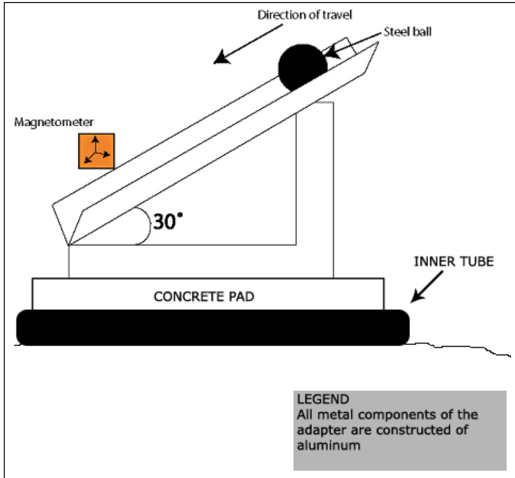
Figure 3-2. Field relative data operational checkout device.
