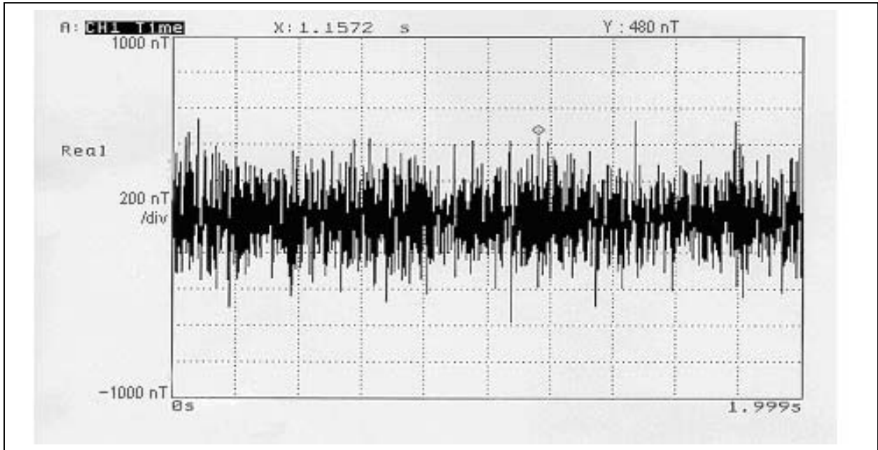
Figure 3-3. Typical magnetic instrument and site ambient noise with the bias nulled out.
