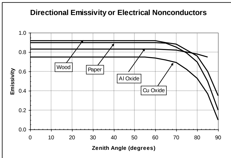
Figure 8-12. Directional emissivity variation for electrical nonconductors.
