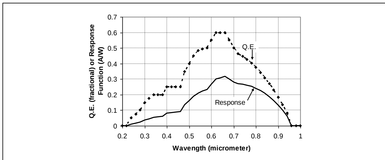
Figure 6-3. Comparison of spectral a Q.E. to a spectral response function.
