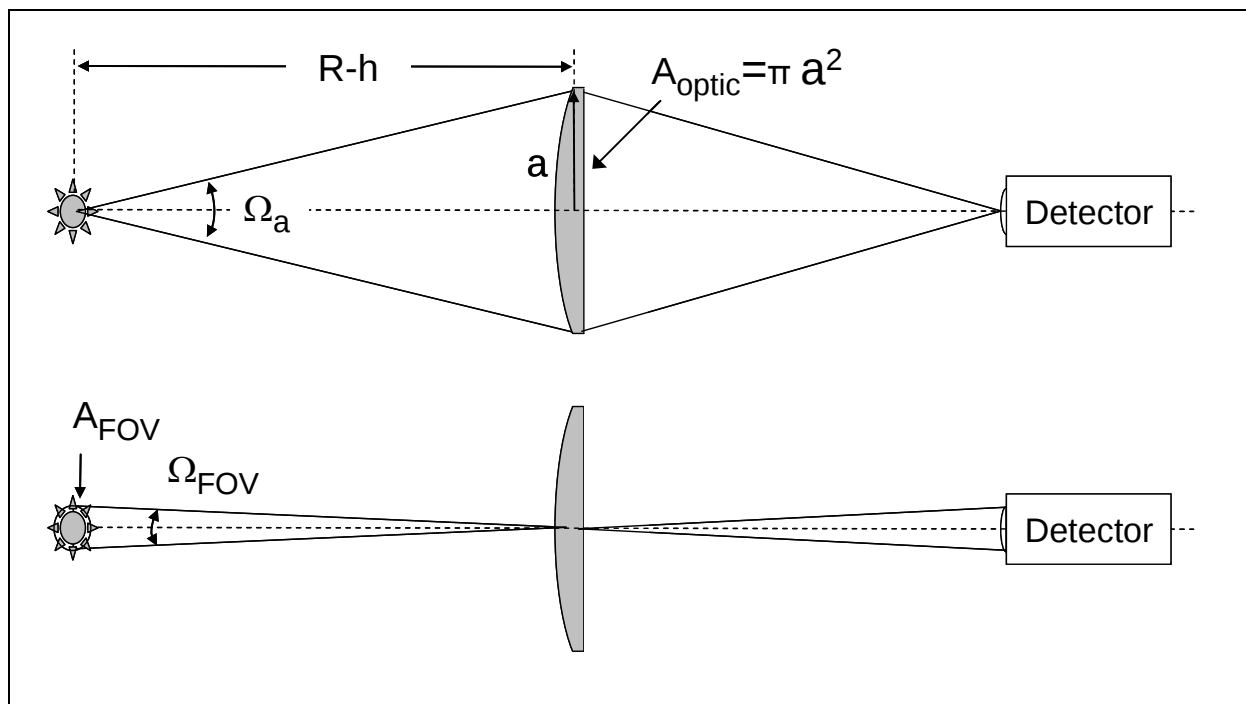
Figure C-2. Illustration of the use of an approximation to the solid angle related to the sensor optical parameters.
