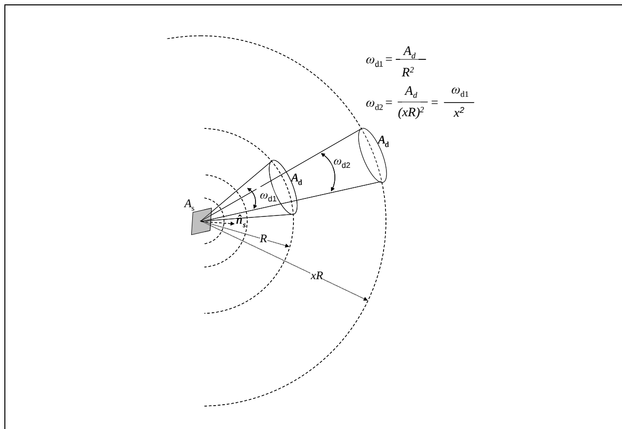
Figure 2-8. Range-squared effect for a point source or an infinitesimal area of a larger source.
