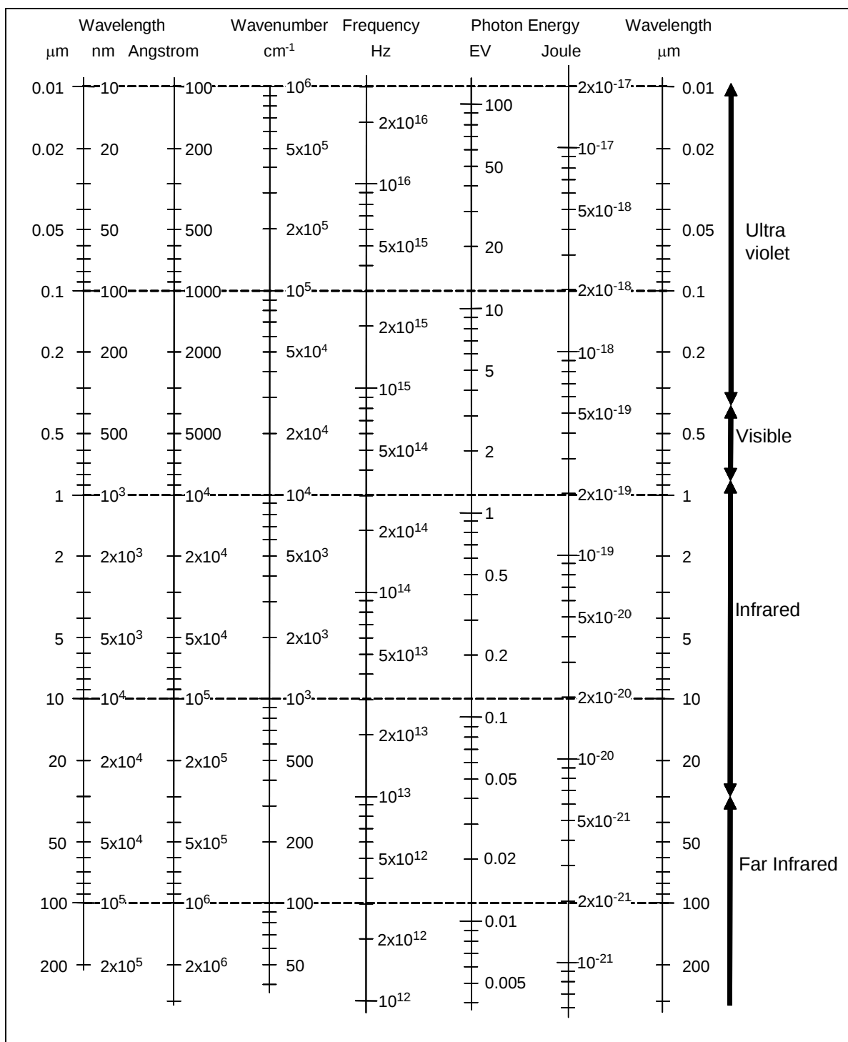
Figure 2-2. Nomograph for conversion between radiometric quantities.
