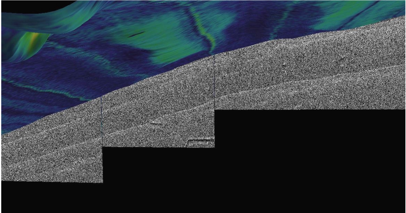
Figure2. Huntce seismic profile as seen in interactive exploration of 3-D scene viewed from below the surface. Surface is seafloor bathymetry with acoustic backscatter (light color represents high backscatter) draped on it.
