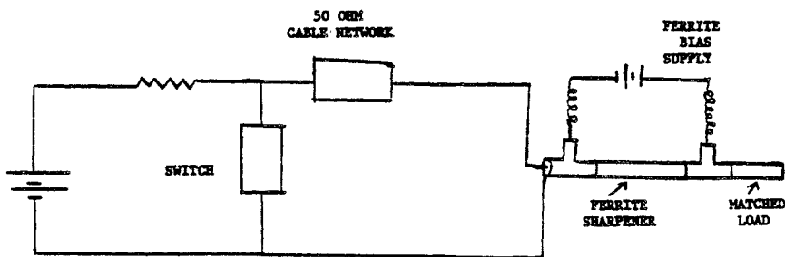
Fig. 5. Experimental Test Circuit for Ferrite Pulse Sharpener.
