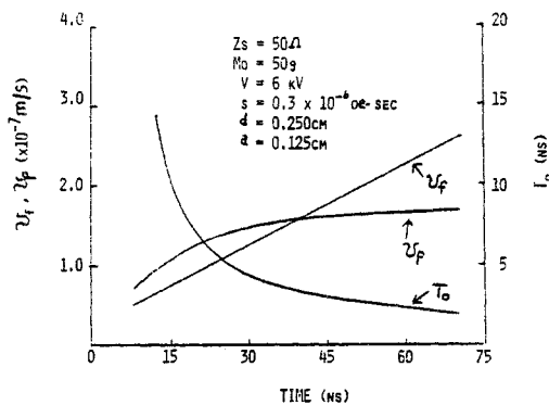
Fig. 4. Variation of Spin Saturation Front Velocity ( v_f ), Phase Velocity ( v_p ), and Switching Time ( T_o ) as Function of Time for 70 ns Ramp Risettime.
