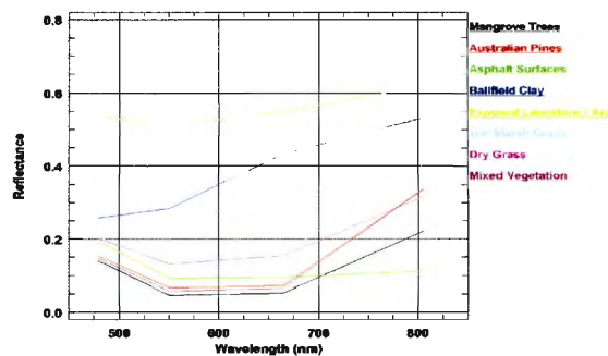
Figure 3. Spectral Signatures of Materials
