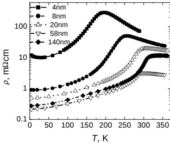
Figure 5. Specific resistance vs. temperature dependence for La_{0.70}Sr_{0.3}MnO_3 films with different thickness prepared on NdGaO_3 substrate
