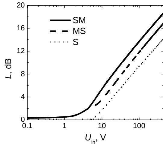
Figure 4. Attenuation ( L ) vs. input voltage ( U_{in} ) for superconducting limiter (dotted line), HSM limiter with magnetic switch connected before (dashed) and after (solid) superconducting strip.
