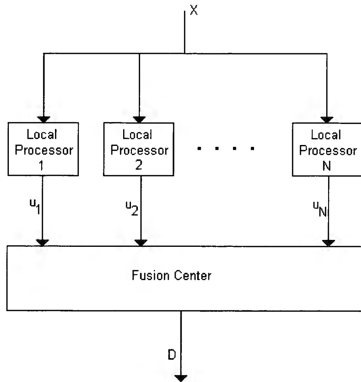
Figure 2. N -Processor Redundant Fusion Network
