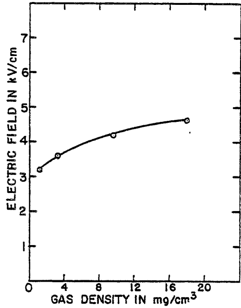
Figure 3. Peak electric field as a function of gas density for foils exploded in 50% \text{O}_2 50% \text{N}_2 .
