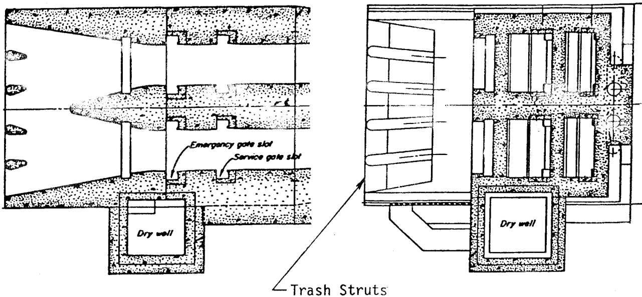
SECTIONAL PLAN AT ELEVATION 1262.00
