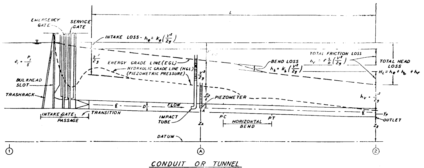
Figure 4. Pressure flow definition sketch.
