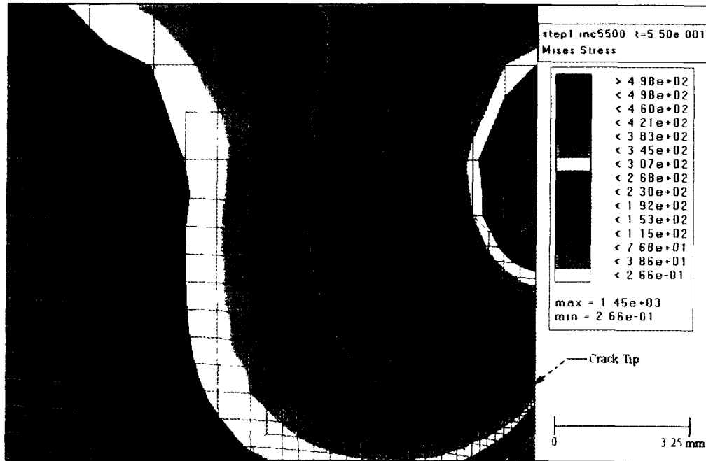
Figure 4.9: von Mises Stress Contours in NS-304SS-12 Specimen (c) D_L/B = 0.04928
