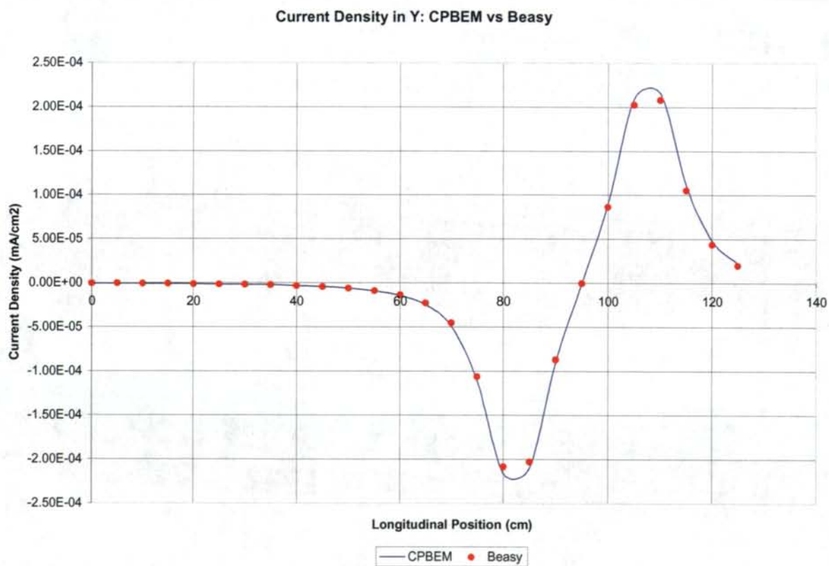
Figure 5.7: Comparison of CPBEM/BEASY Y Current Densities
