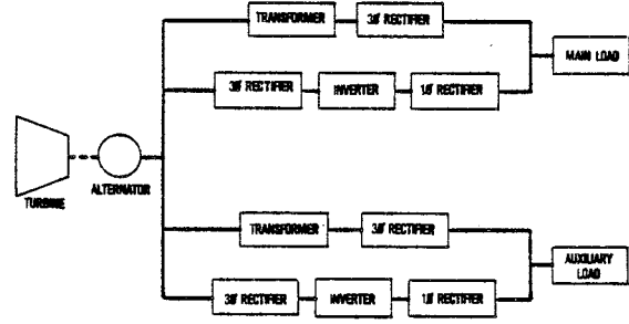
Fig. 3 Systems Using Turbine/Alternator Sources
