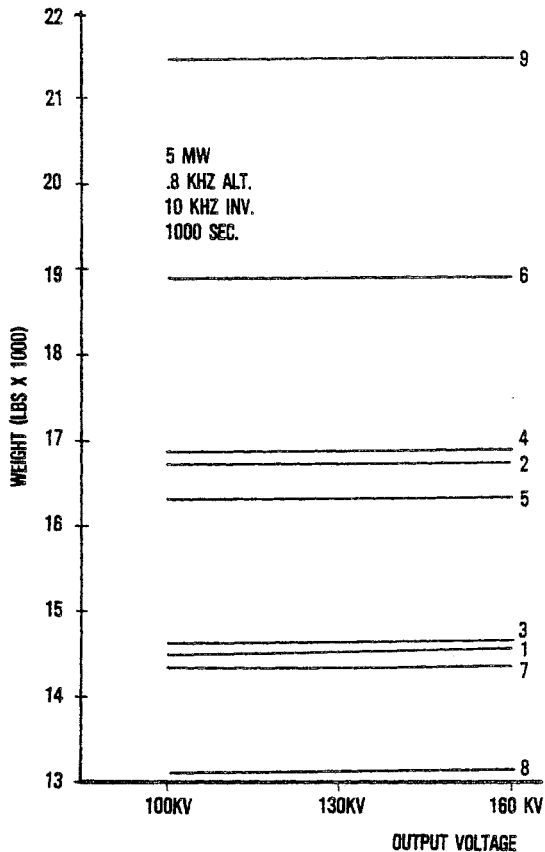
Fig. 7 System Weight as a Function of Output Voltage
