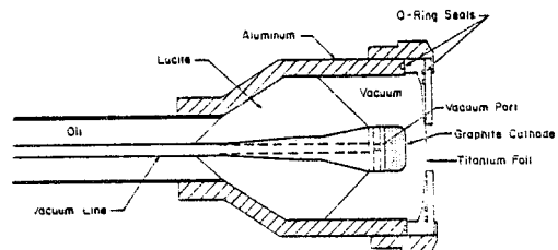
Figure 3: The Diode
