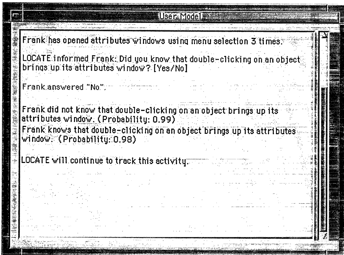
Figure 5. Example Information Placed in LOCATE's User Model Following a User's Answer to the Question in the Help Window Shown in Figure 4
