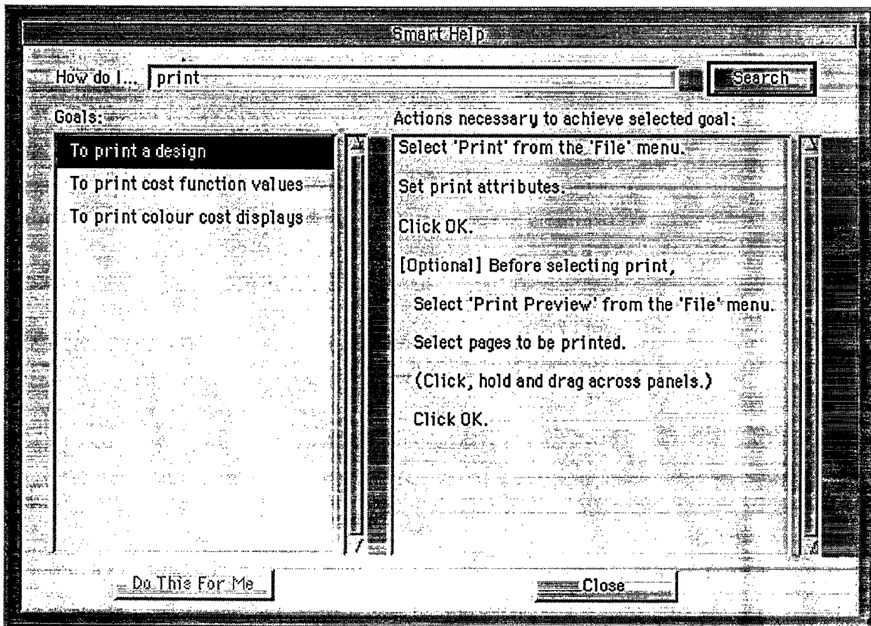
Figure 6. Example of LOCATE's Smart Help Window
