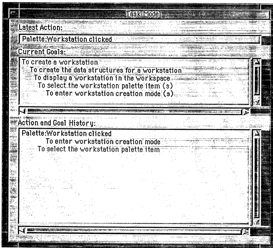
Figure 1. LOCATE's Task Model Window
