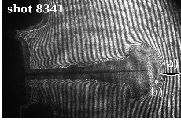
Figure 5: Reconstructed interferogram and superposed rod shadow. Hydrodynamic expansion of tip correspond to t = 110 ns from x-ray onset. a) Region ( r = 0, 3 \text{ mm} \leq z \leq 10 \text{ mm} ) where integrated line density of Figure 7 was computed, b) Location where data of Figure 6 was collected.
