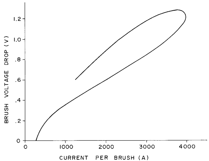
Fig. 5. Results of Brush Testing Shot.
