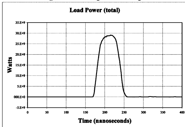
Figure 10. Total load power.
