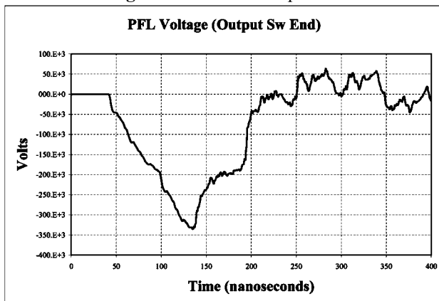
Figure 11. PFL Voltage (Output Switch End)
