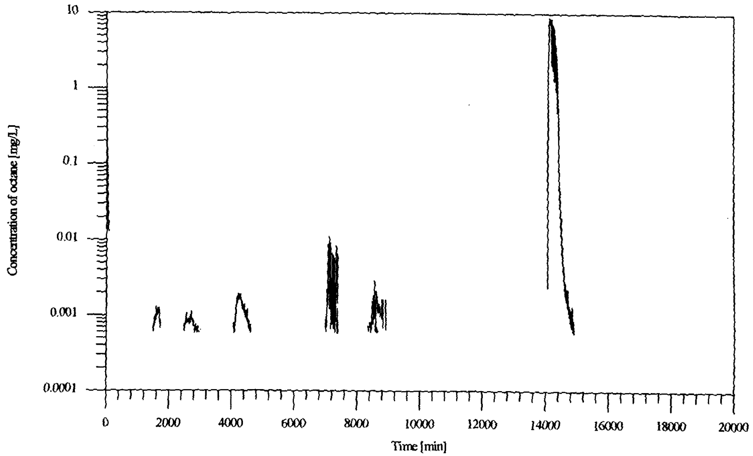
Figure 4.21: Octane concentration in the outlet air of the physical model vs. time for Q_{air} = 10 \text{ L/min} both steady and pulsed injection and Mf \approx 35.14 \text{ g.} out of air flow field wet medium experiment. Draining of the physical model occurred at 14012 min
