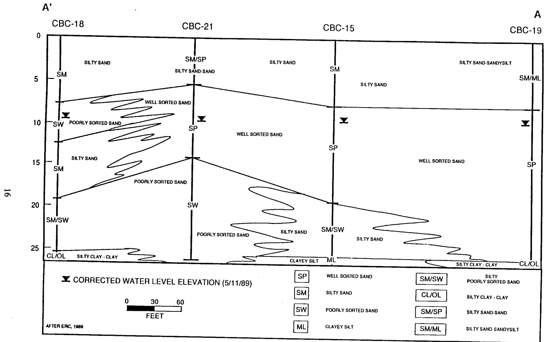
Figure 7. Cross Section A-A' Showing Site Lithology and Depth to Groundwater at the Naval Exchange Gasoline Station, Port Hueneme (PRC and JMM, 1991)
