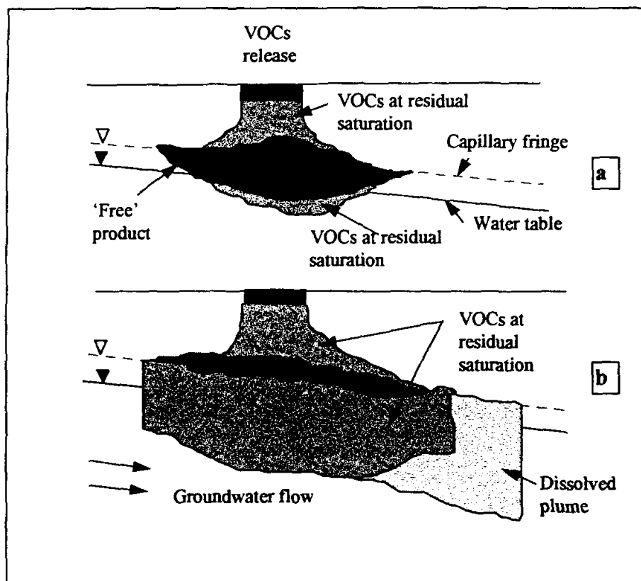
Figure 1.1: Conceptual picture of fate of organic LNAPL liquids after their release. (a) liquid seeps downwards and reaches the groundwater table where it pools and spreads laterally; (b) effect of groundwater movement and groundwater table rise on liquid distribution in subsurface.
