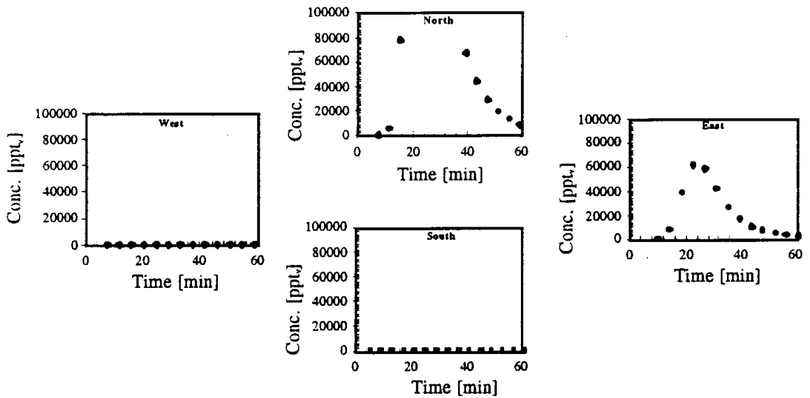
Figure SF-2. Directional soil vapor extraction well response to 1.0 mL injection of SF 6 into MP-2 (4-ft below ground surface); vapor extraction system only; flow per well 8 - 10 ft 3 /min (9/7/96).
