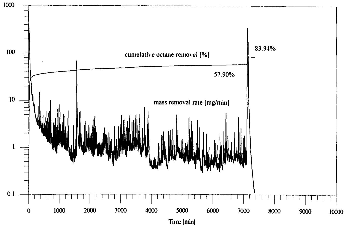
Figure 5.11: Mass removal rate and cumulative octane removal vs. time for Q_{air} = 10 L/min steady injection and M^f = 35.14 g., final wet medium experiment. Draining of the physical model occurred at 7105 min.
