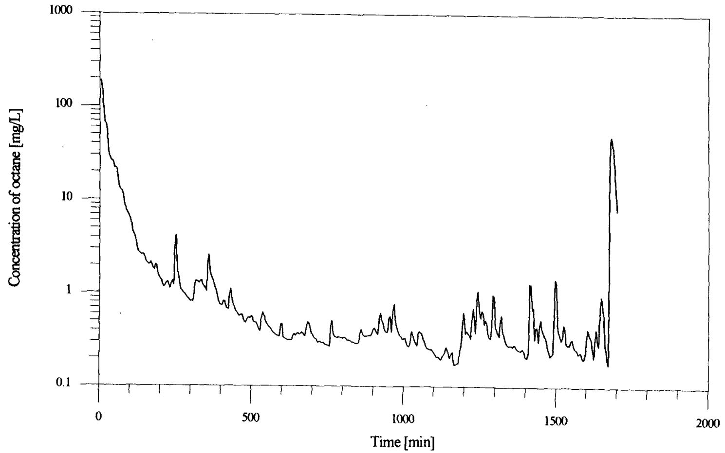
Figure 4.3: Octane concentration in the outlet air of the physical model vs. time for Q_{air} = 11 L/min steady injection and M = 7.03 g., preliminary wet medium experiment.
