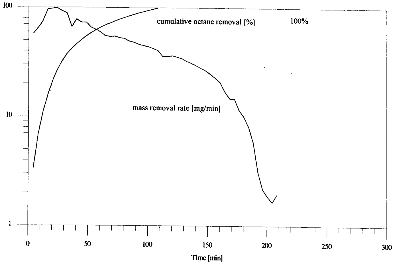
Figure 5.1: Mass removal rate and cumulative octane removal vs. time for Q_{air} = 11 L/min steady injection and M^* = 7.03 g., preliminary dry medium experiment.
