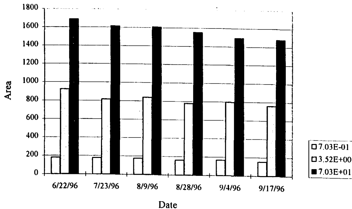
Figure 3.4: Result of standard run for octane on different dates. The sensitivity of the gas chromatograph was set at "low". Octane concentration for standard run were 7.03E-01, 3.52E+00 & 7.03E+01 mg/L-air.
