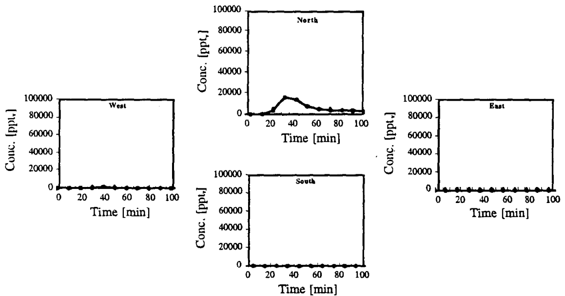
Figure SF-12. Directional soil vapor extraction well response to 0.5 mL injection of SF 6 into MP-6 (8-ft below ground surface); vapor extraction system with air injection; flow per extraction well ≈8 ft 3 /min; injection well flow 5 ft 3 /min (10/28/96).
