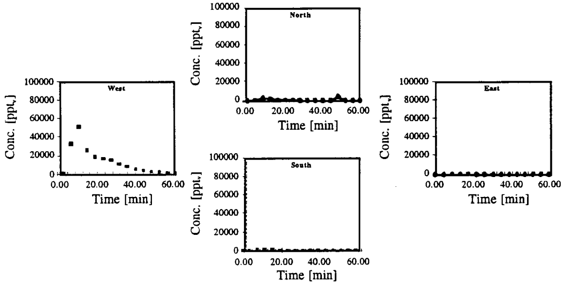
Figure SF-1. Directional soil vapor extraction well response to 0.5 mL injection of SF 6 into MP-1 (4-ft below ground surface); vapor extraction system only; flow per well 8 - 10 ft 3 /min (9/7/96).
