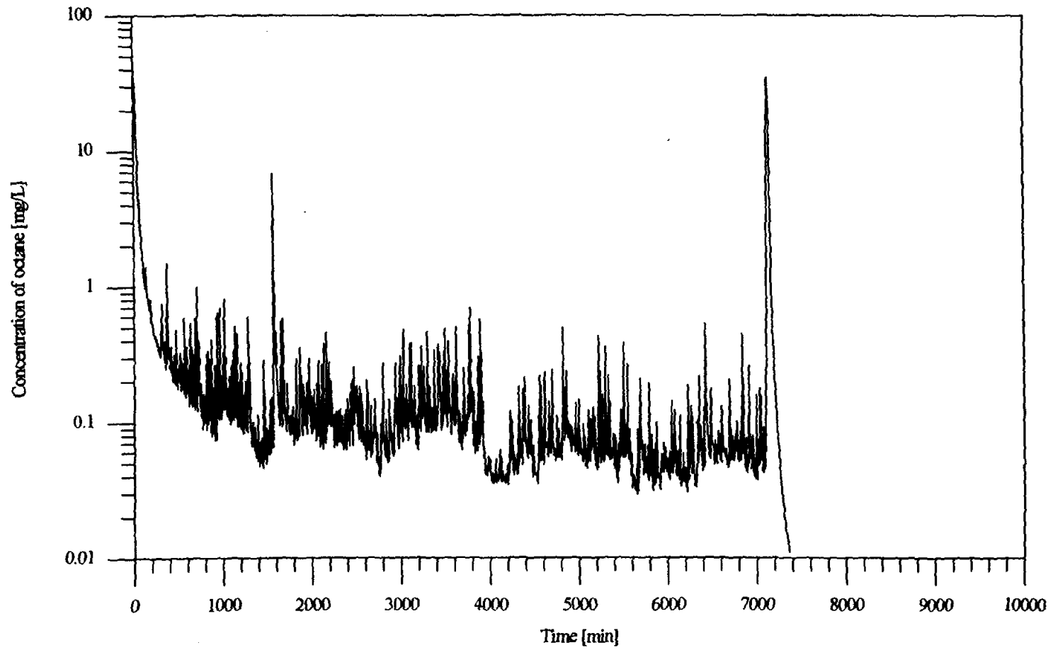
Figure 4.12: Octane concentration in the outlet air of the physical model vs. time for Q_{air} = 10 \text{ L/min} steady injection and M^0 = 35.14 \text{ g.} final wet medium experiment. Draining of the physical model occurred at 7105 min
