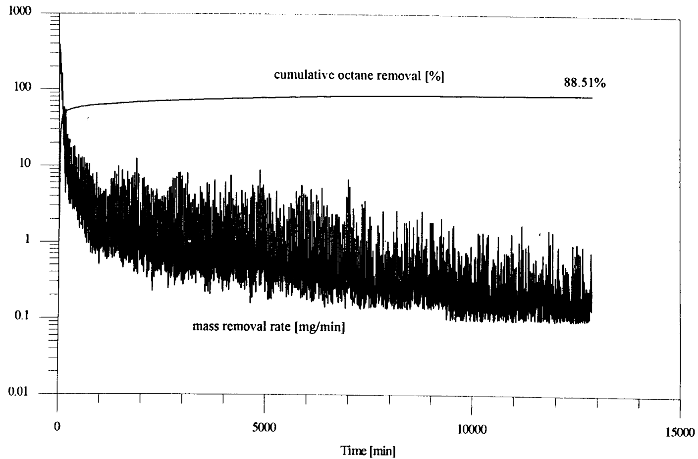
Figure 5.14: Mass removal rate and cumulative octane removal vs. time for Q_{air} = 10 L/min pulsed injection and M^f = 35.14 g., intermediate wet medium experiment.
