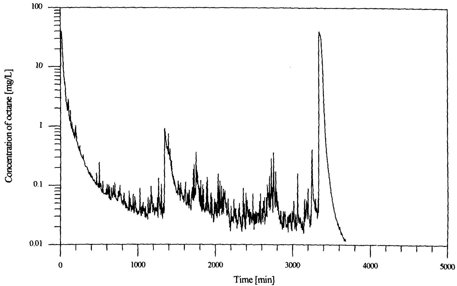
Figure 4.13: Octane concentration in the outlet air of the physical model vs. time for Q_{air} = 10 L/min steady injection and M^f = 35.14 g., final wet medium experiment. Draining of the physical model occurred at 3335 min
