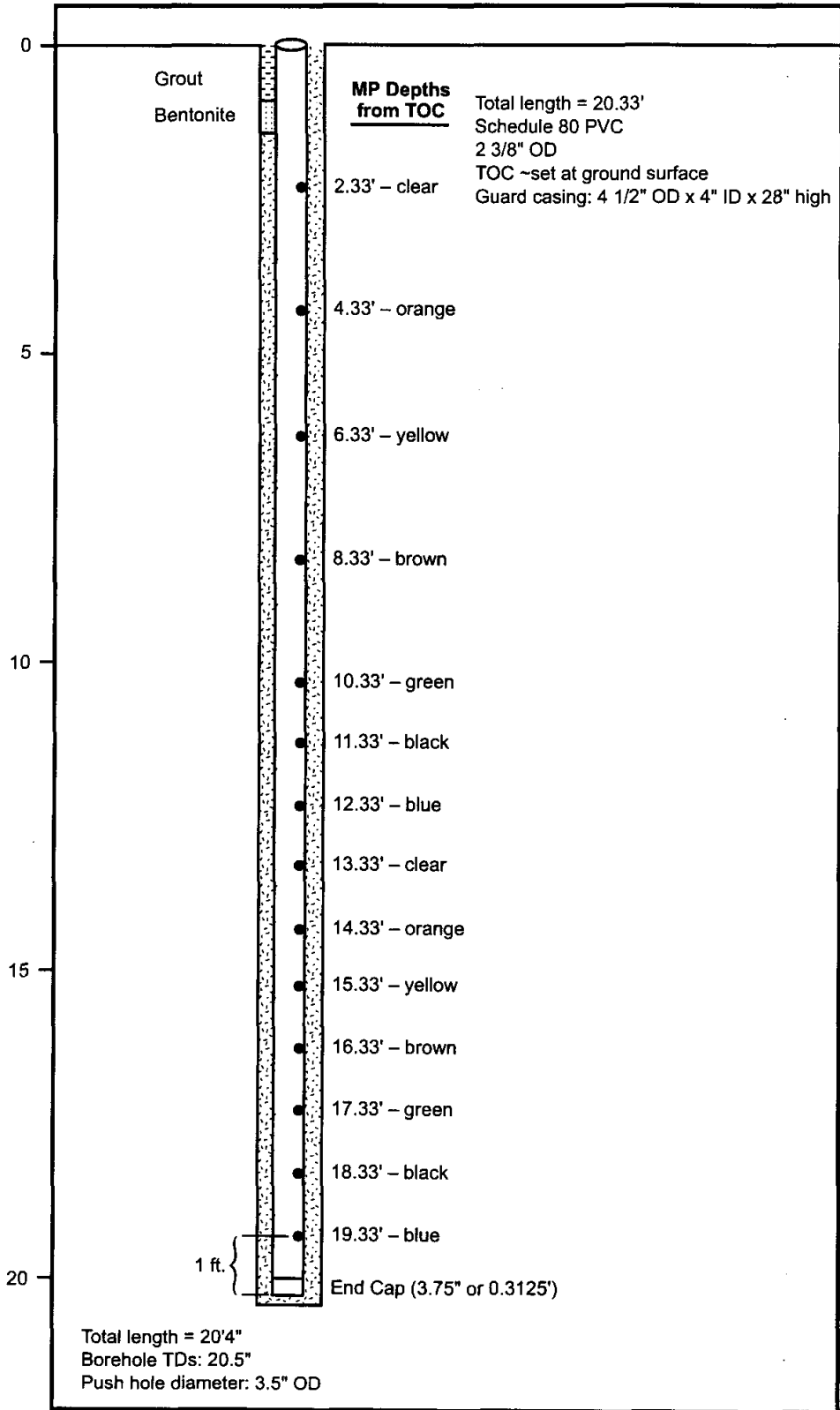
Figure 19. Schematic Diagram Showing a Cross Section of a Typical Multi-Level Sampler
