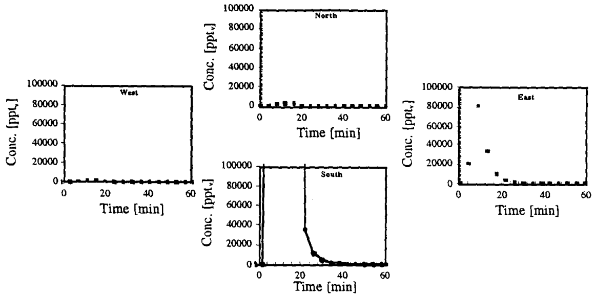
Figure SF-3. Directional soil vapor extraction well response to 0.5 mL injection of SF 6 into MP-3 (4-ft below ground surface); vapor extraction system only; flow per well 8 - 10 ft 3 /min (9/7/96).
