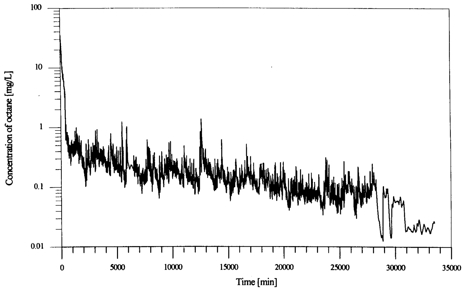
Figure 4.5: Octane concentration in the outlet air of the physical model vs. time for Q_{air} = 1.25 L/min steady injection and M = 35.14 g., intermediate wet medium experiment.
