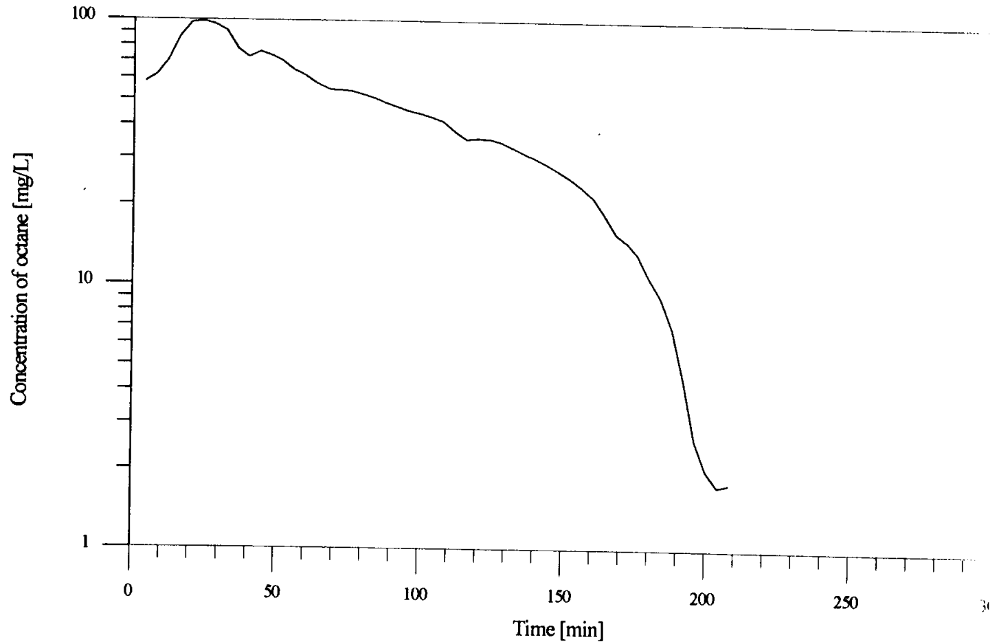
Figure 4.1: Octane concentration in the outlet air of the physical model vs. time for Q_{air} = 11 L/min steady injection and M = 7.03 g., preliminary dry medium experiment.
