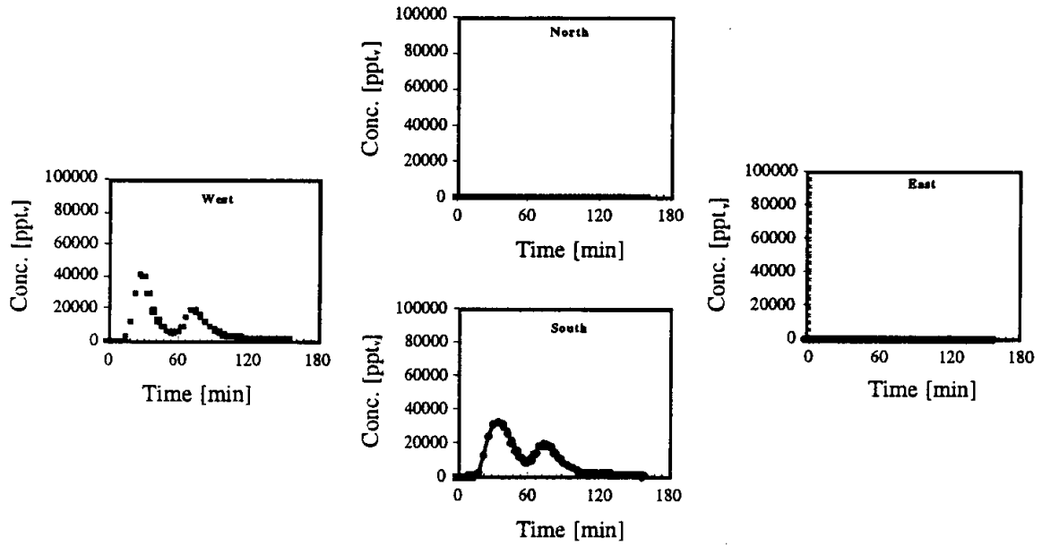
Figure SF-5. Directional soil vapor extraction well response to 0.5 mL injection of SF 6 into MP-5 (4-ft below ground surface); vapor extraction system only; flow per well 8 - 10 ft 3 /min (9/8/96).
