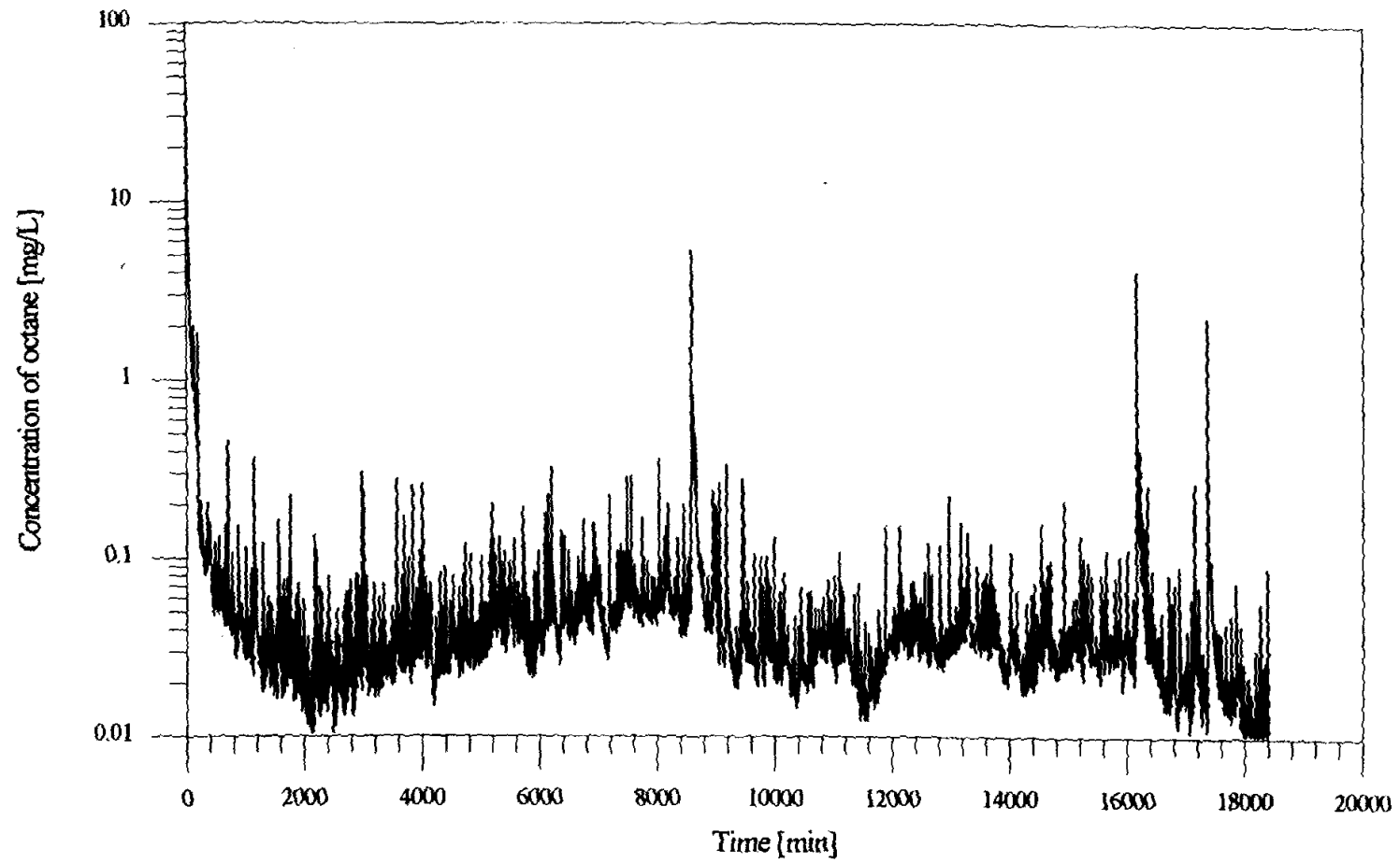
Figure 4.7: Octane concentration in the outlet air of the physical model vs. time for Q_{air} = 10 L/min steady injection and M^f = 35.14 g., intermediate wet medium experiment.
