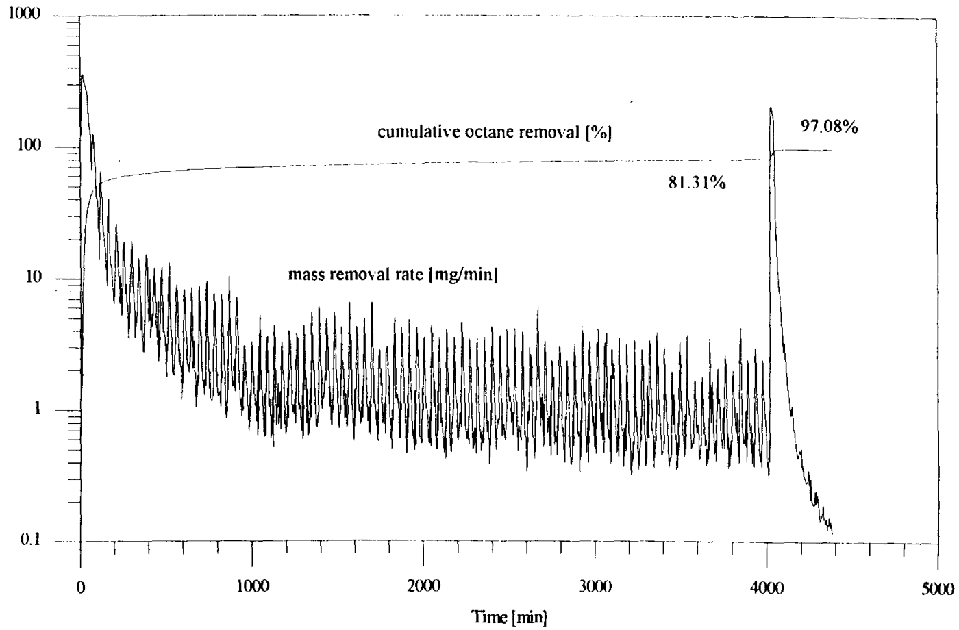
Figure 5.16: Mass removal rate and cumulative octane removal vs. time for Q_{air} = 10 L/min pulsed injection and M^l = 35.14 g., final wet medium experiment. Draining of the physical model occurred at 4016 min.
