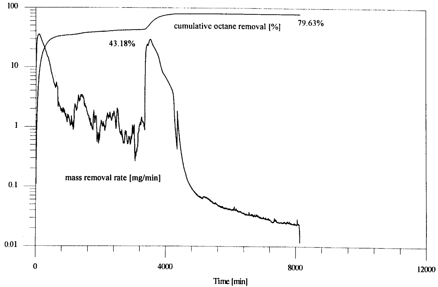
Figure 5.8: Mass removal rate and cumulative octane removal vs. time for Q_{air} = 1.25 L/min steady injection and \Lambda P = 35.14 g., final wet medium experiment. Draining of the physical model occurred at 3347 min
