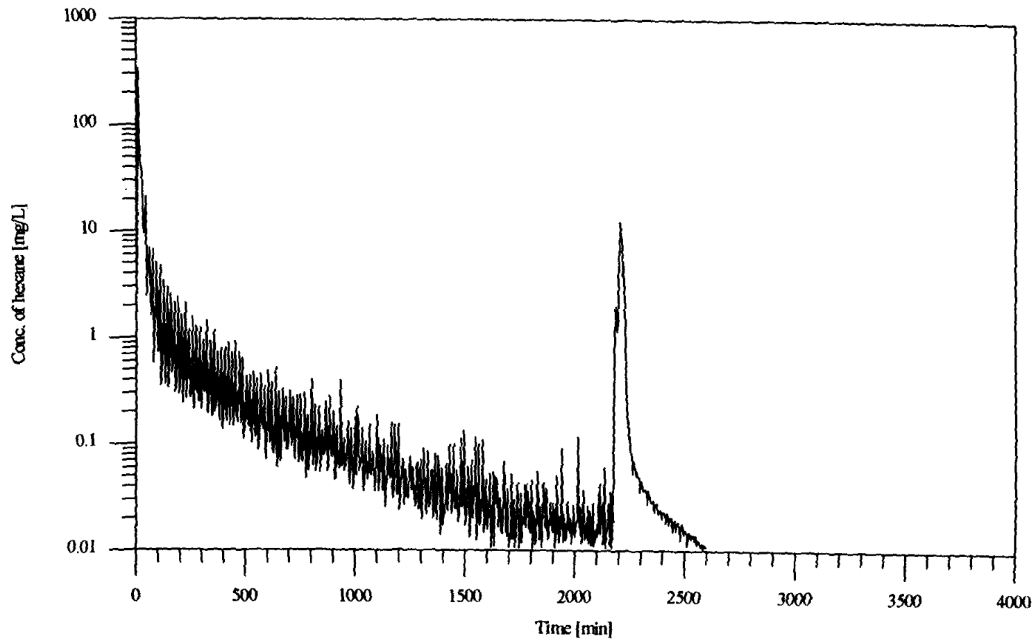
Figure 4.20: Hexane concentration in the outlet air of the physical model vs. time for Q_{air} = 10 L/min pulsed injection and M = 33 g., final wet medium experiment. Draining of the physical model occurred at 2174 min
