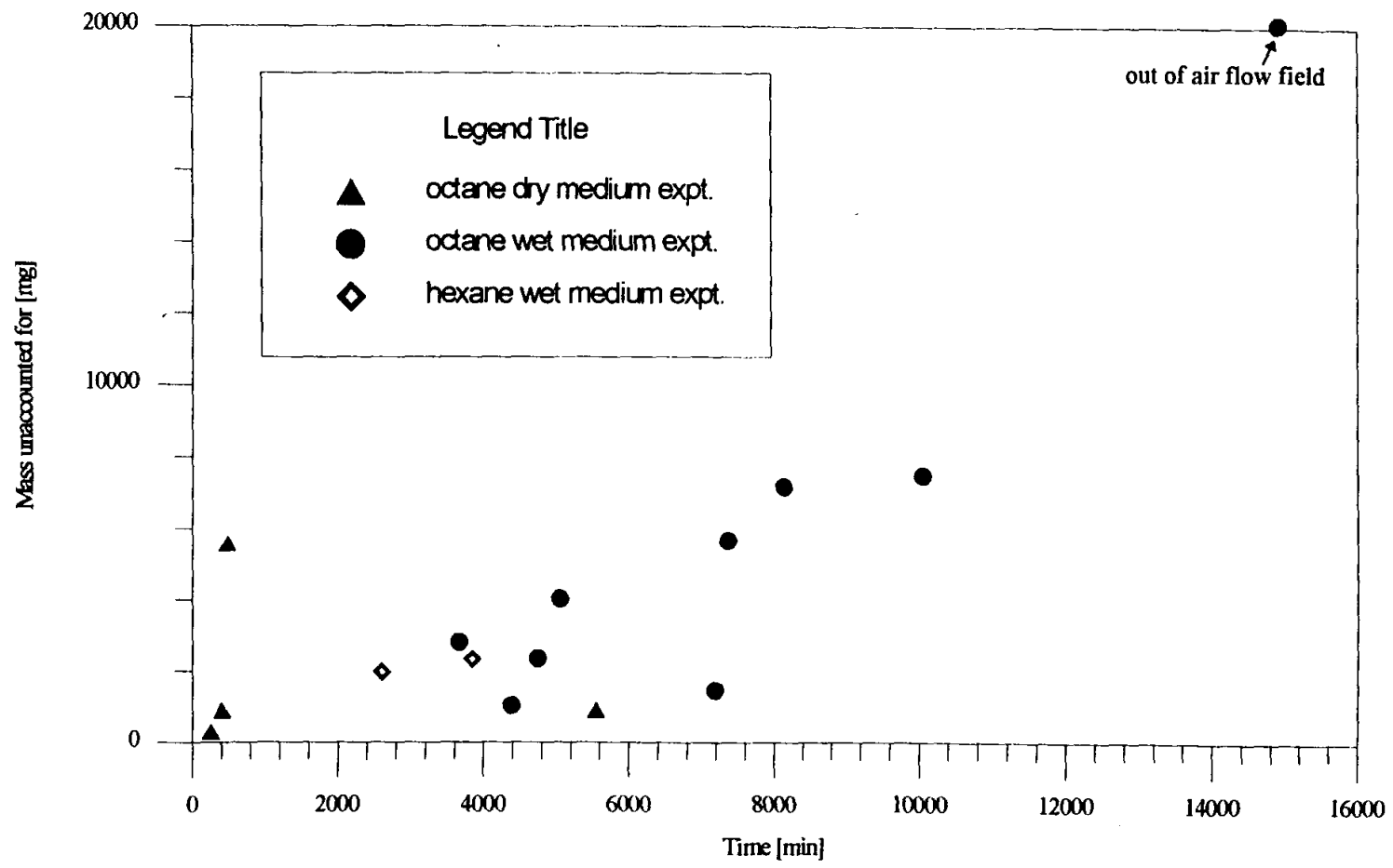
Figure 5.23: Mass unaccounted for in the final mass balance vs. time.
