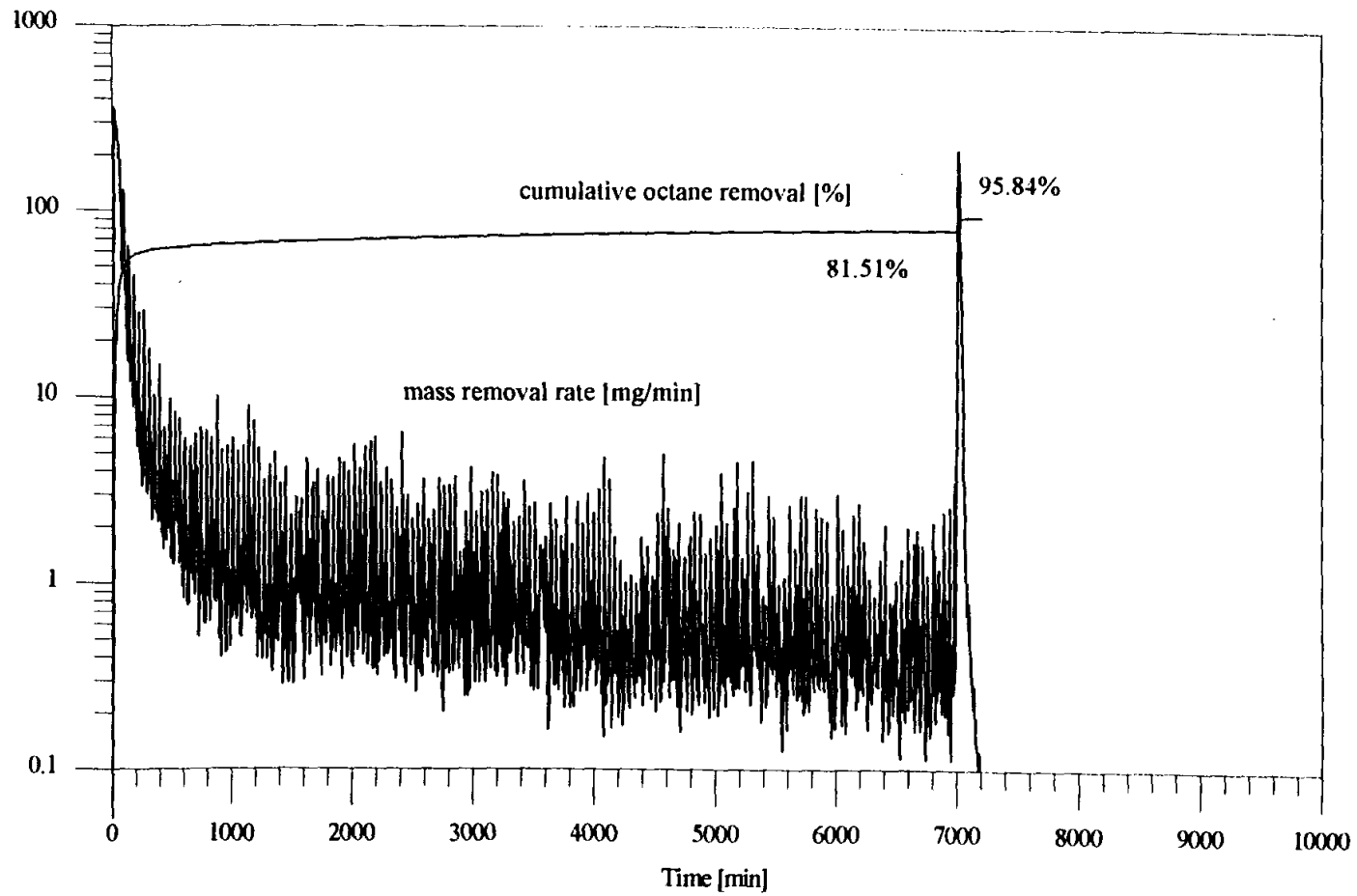
Figure 5.15: Mass removal rate and cumulative octane removal vs. time for Q_{air} = 10 L/min pulsed injection and M^0 = 35.14 g., final wet medium experiment. Draining of the physical model occurred at 6983 min.
