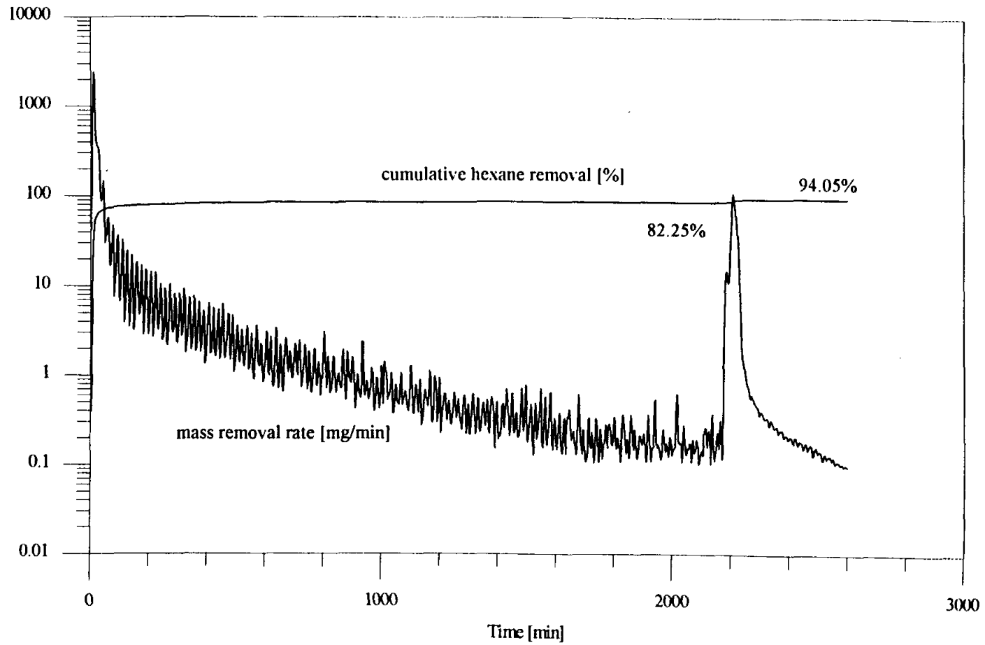
Figure 5.22: Mass removal rate and cumulative hexane removal vs. time for Q_{air} = 10 L/min pulsed injection and M^p = 33 g., final wet medium experiment. Draining of the physical model occurred at 2174 min.
