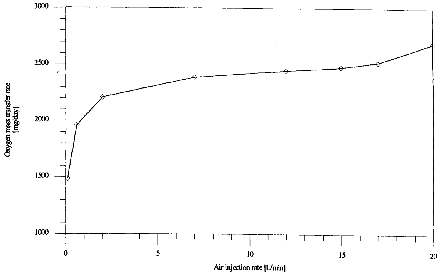
Figure A5: Oxygen Mass Transfer Rate vs. Air Injection Rate for constant water flowrate (270 cm 3 /min) and variable air injection for a layered system.
