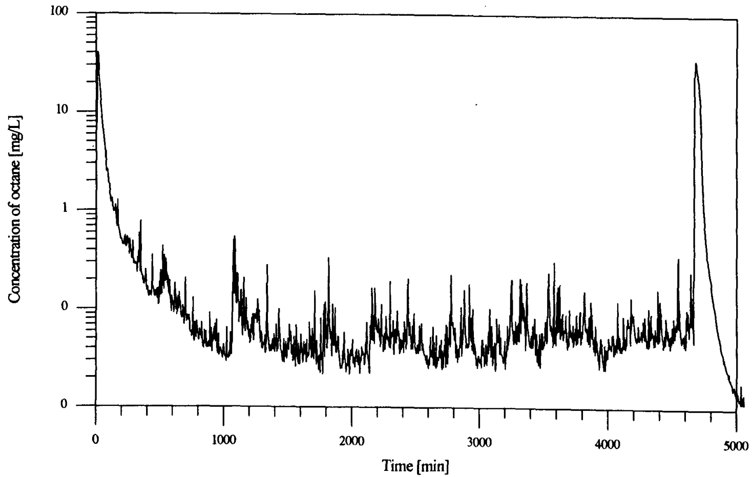
Figure 4.14: Octane concentration in the outlet air of the physical model vs. time for Q_{air} = 10 L/min steady injection and M^f = 35.14 g., final wet medium experiment. Draining of the physical model occurred at 4664 min
