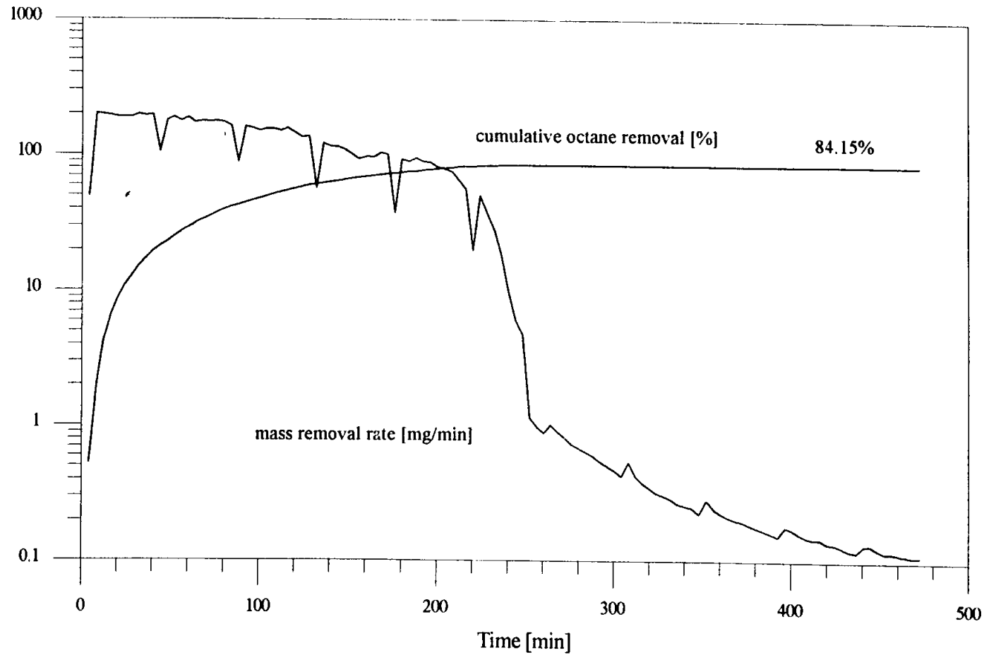
Figure 5.5: Mass removal rate and cumulative octane removal vs. time for Q_{air} = 10 L/min pulsed injection and M^* = 35.14 g., intermediate dry medium experiment.
