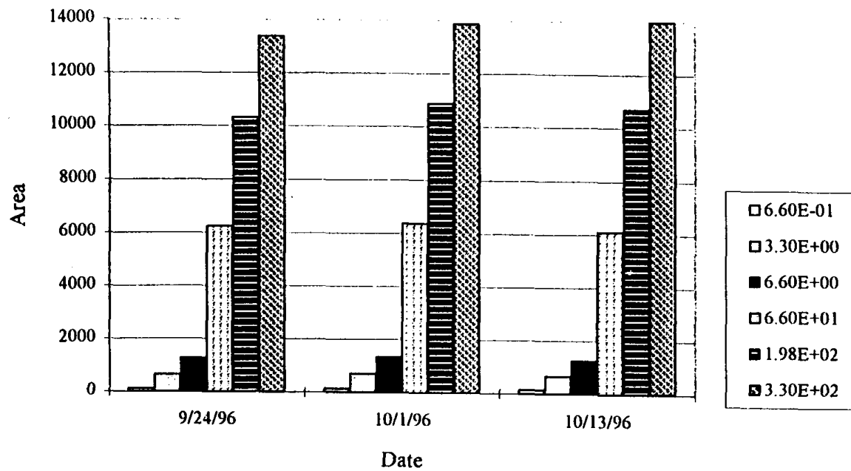
Figure 3.6: Result of standard run for hexane on different dates. The sensitivity of the gas chromatograph was set at "low". Hexane concentration for standard run were 6.6E-01, 3.30, 6.60, 6.6E+01, 1.98E+02 & 3.30E+02 mg/L-air.
