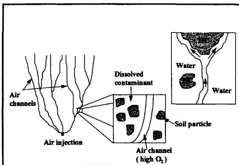
Figure 2.1: Conceptual model of processes occurring during in situ air sparging (after Rutherford 1995).
