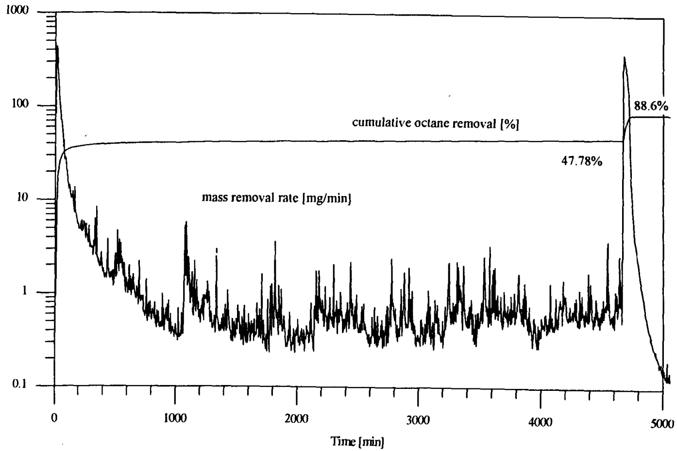
Figure 5.13: Mass removal rate and cumulative octane removal vs. time for Q_{air} = 10 L/min steady injection and M = 35.14 g., final wet medium experiment. Draining of the physical model occurred at 4664 min.
