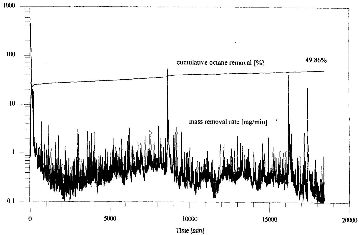
Figure 5.10: Mass removal rate and cumulative octane removal vs. time for Q_{air} = 10 L/min steady injection and M^p = 35.14 g., intermediate wet medium experiment.
