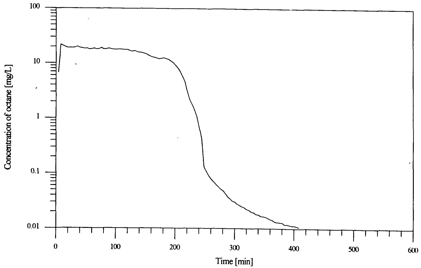
Figure 4.6: Octane concentration in the outlet air of the physical model vs. time for Q_{air} = 10 L/min steady injection and M^p = 35.14 g., intermediate dry medium experiment.
