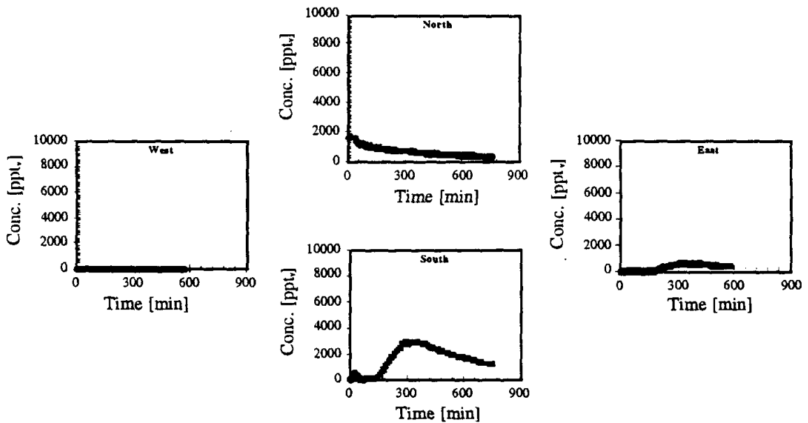
Figure SF-8. Directional soil vapor extraction well response to 0.5 mL injection of SF 6 into MP-9 (4-ft below ground surface); vapor extraction system only; flow per well 8 - 10 ft 3 /min (9/8/96).
