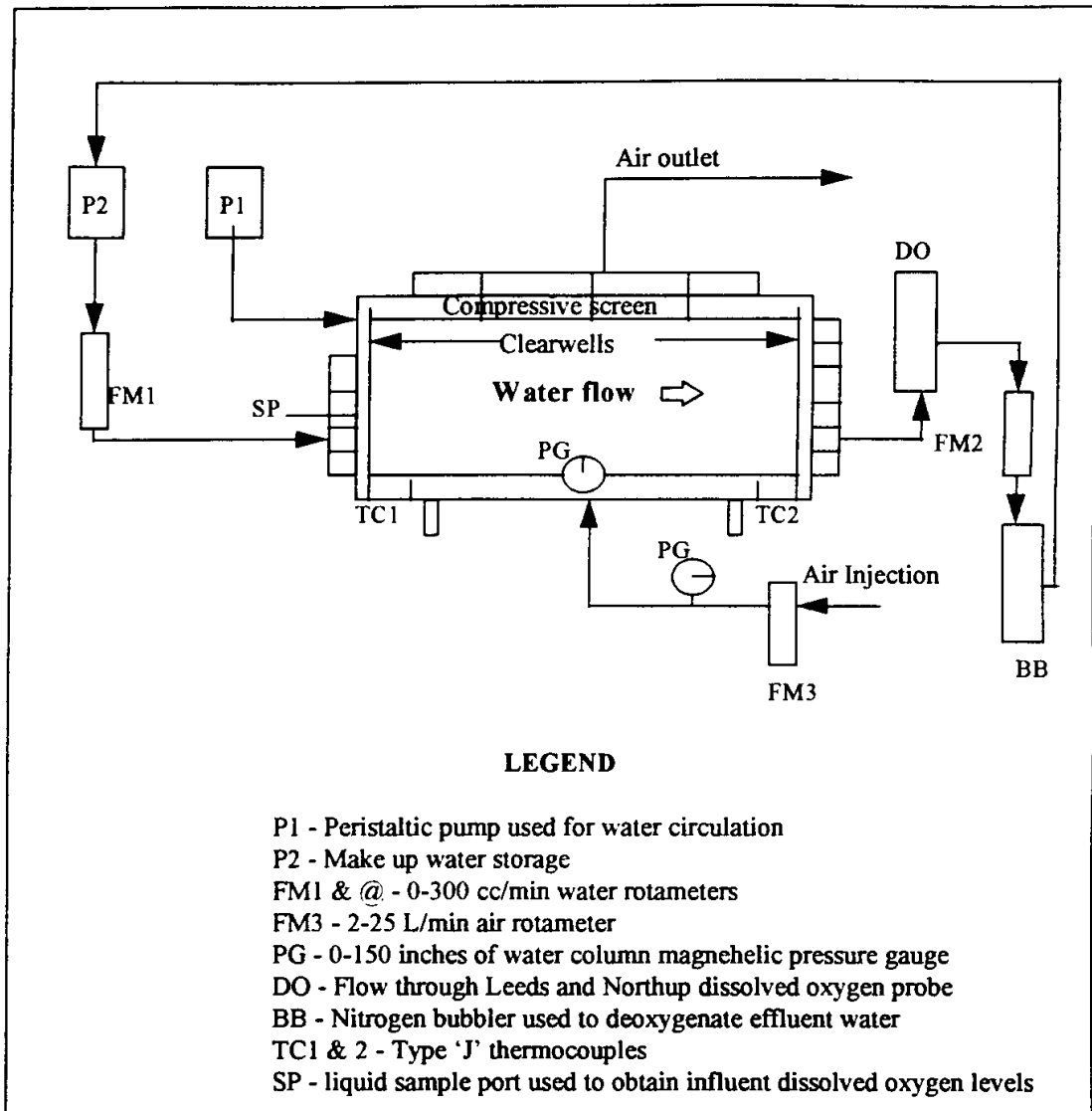
Figure A2. Experimental flow loop.
