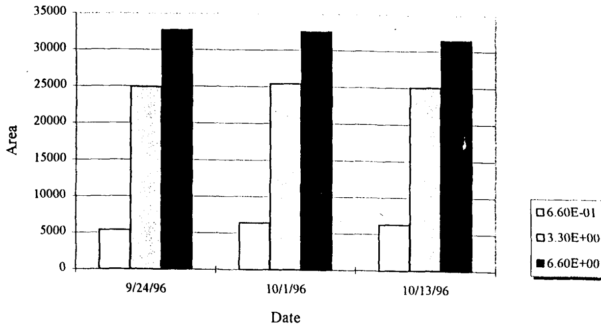
Figure 3.5: Result of standard run for hexane on different dates. The sensitivity of the gas chromatograph was set at "high". Hexane concentration for standard run were 0.66, 3.30- & 6.60 mg/L-air.
