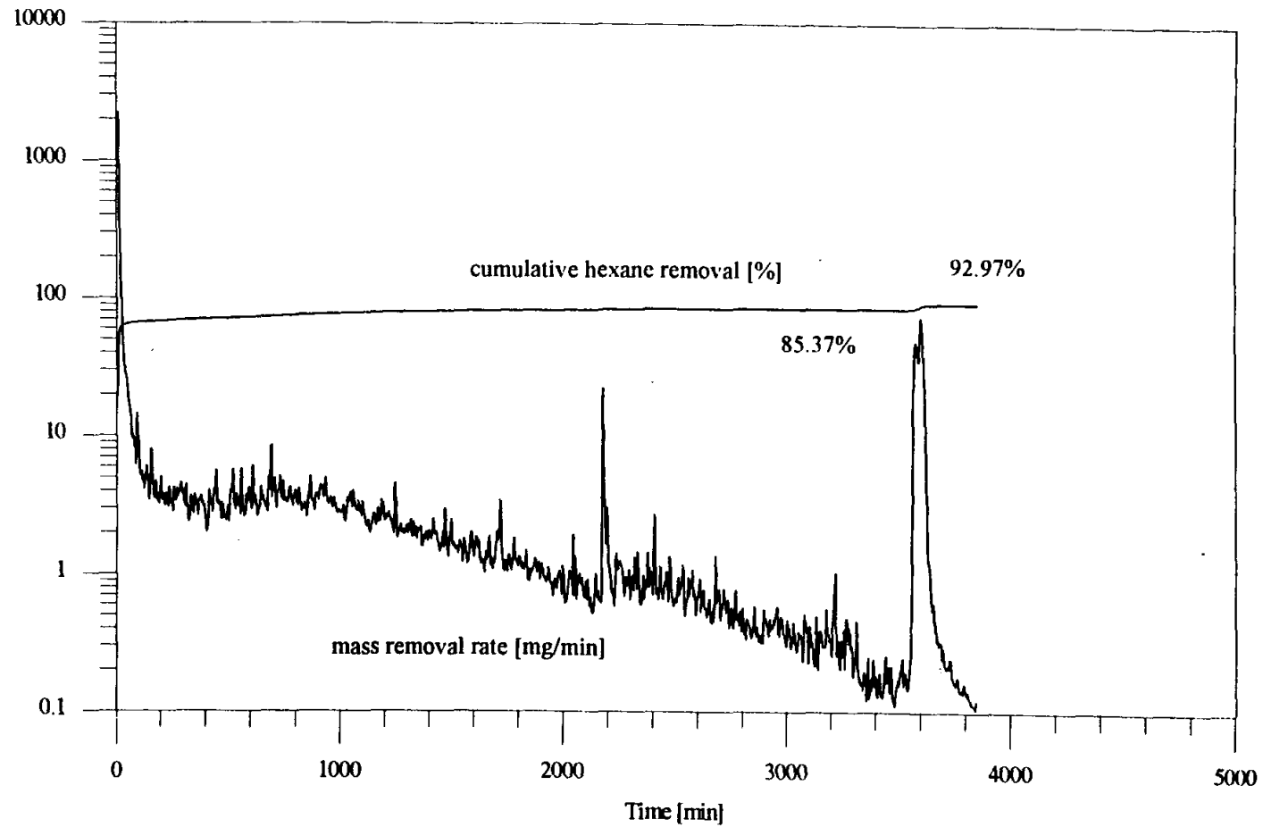
Figure 5.21: Mass removal rate and cumulative hexane removal vs. time for Q_{air} = 10 L/min steady injection and M = 33 g., final wet medium experiment. Draining of the physical model occurred at 3556 min.
