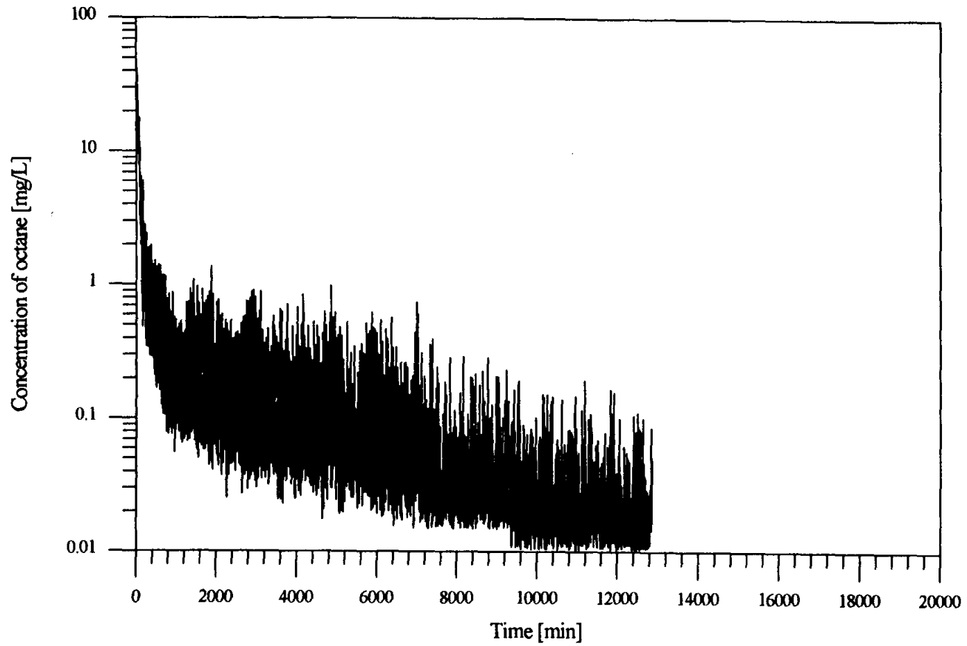
Figure 4.9: Octane concentration in the outlet air of the physical model vs. time for Q_{air} = 10 L/min pulsed injection and M^p = 35.14 g., intermediate wet medium experiment.
