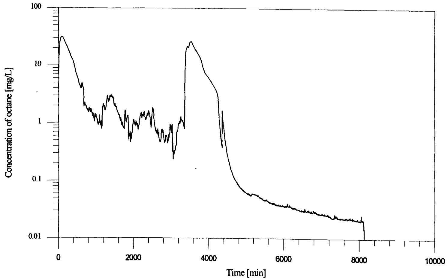
Figure 4.10: Octane concentration in the outlet air of the physical model vs. time for Q_{air} = 1.25 L/min steady injection and M^0 = 35.14 g., final wet medium experiment. Draining of the physical model occurred at 3347 min.
