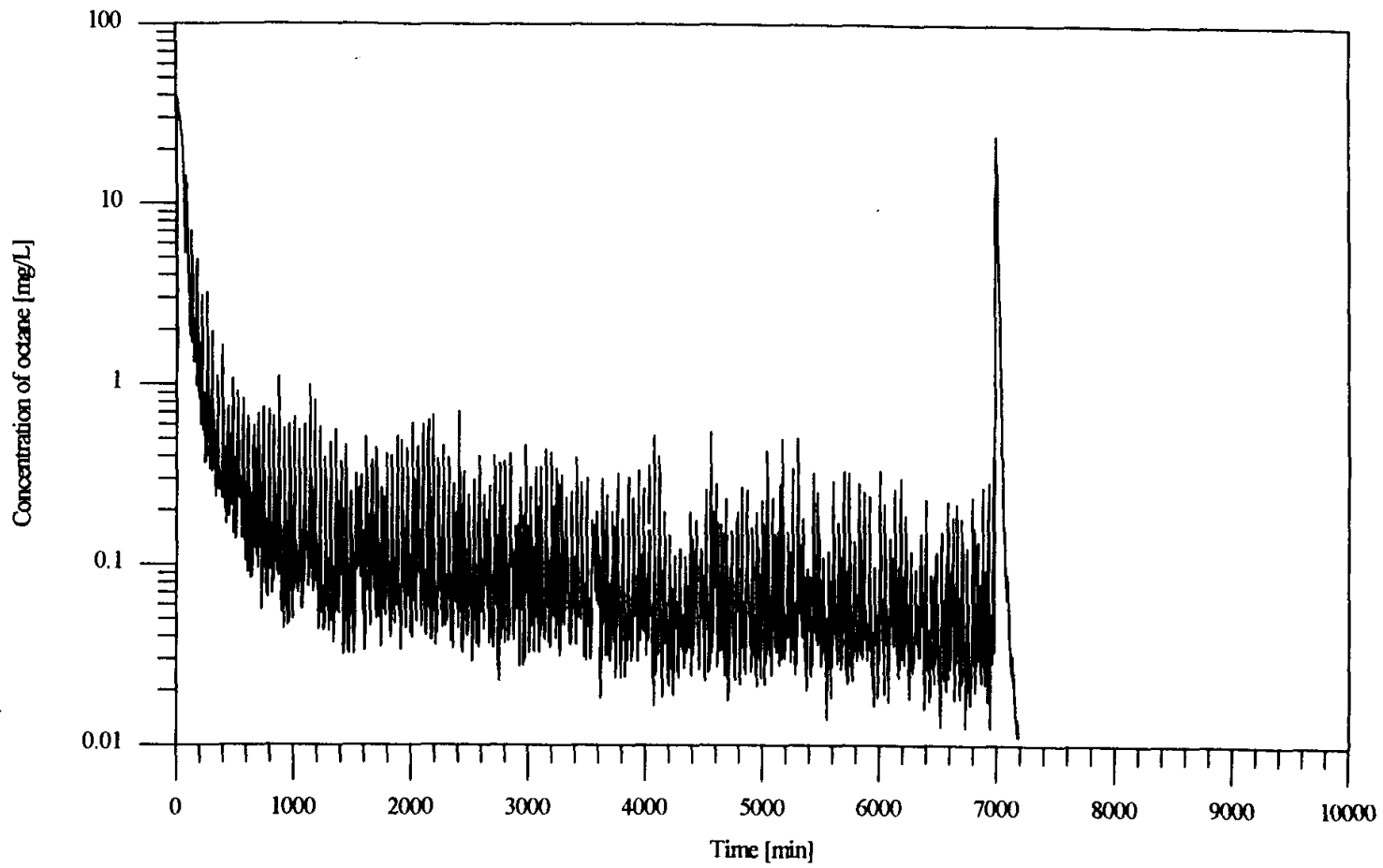
Figure 4.15: Octane concentration in the outlet air of the physical model vs. time for Q_{air} = 10 L/min pulsed injection and M^f = 35.14 g., final wet medium experiment. Draining of the physical model occurred at 6983 min
