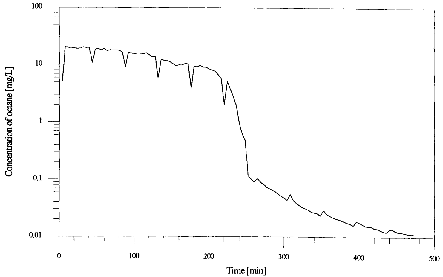
Figure 4.8: Octane concentration in the outlet air of the physical model vs. time for Q_{air} = 10 L/min pulsed injection and M^{\#} = 35.14 g., intermediate dry medium experiment.
