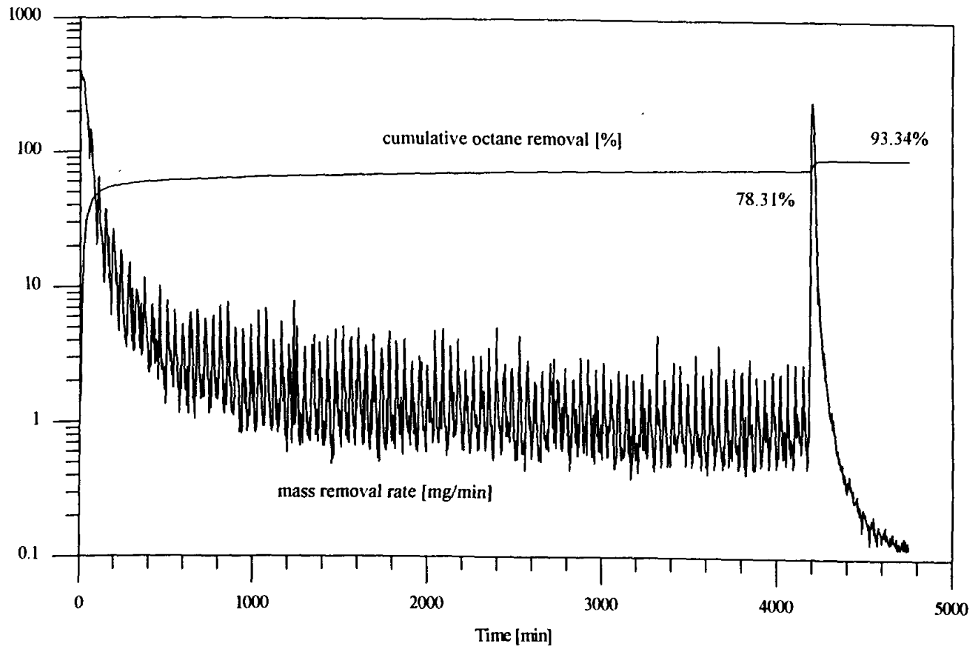
Figure 5.17: Mass removal rate and cumulative octane removal vs. time for Q_{air} = 10 L/min pulsed injection and M^P = 35.14 g., final wet medium experiment. Draining of the physical model occurred at 4184 min.
