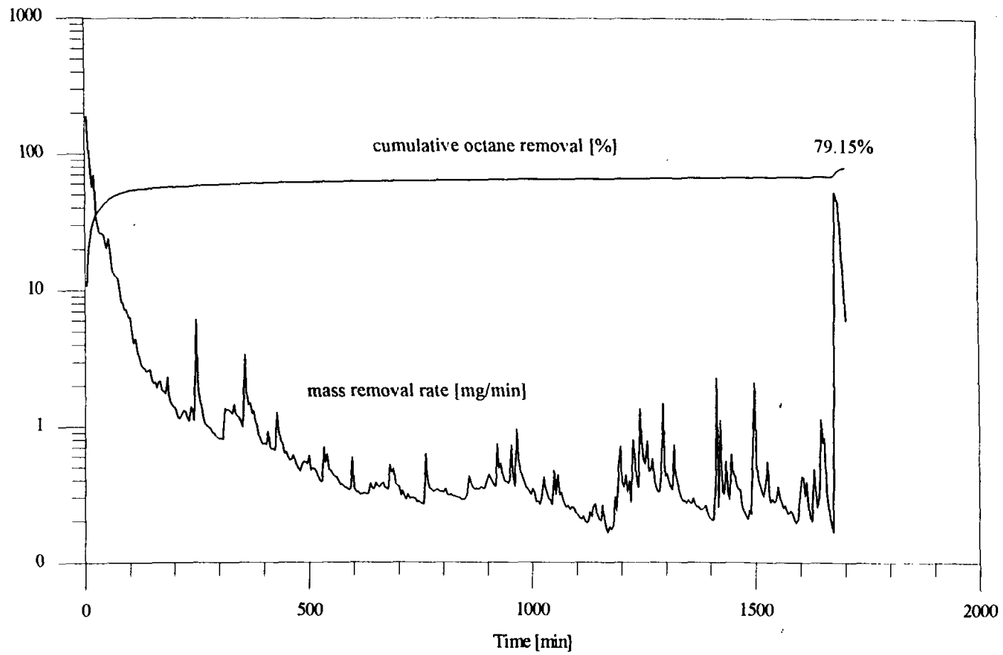
Figure 5.6: Mass removal rate and cumulative octane removal vs. time for Q_{air} = 11 L/min steady injection and M^p = 7.03 g., preliminary wet medium experiment.
