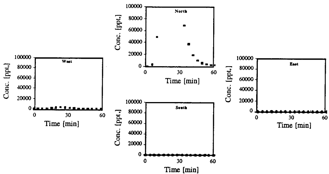
Figure SF-6. Directional soil vapor extraction well response to 0.5 mL injection of SF 6 into MP-6 (4-ft below ground surface); vapor extraction system only; flow per well 8 - 10 ft 3 /min (9/8/96).
