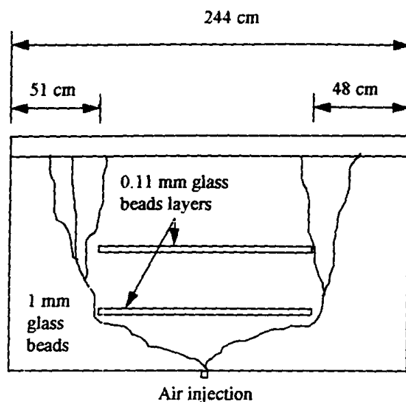
Figure A1: Layered setting for the physical model shown with typical air flow field.
