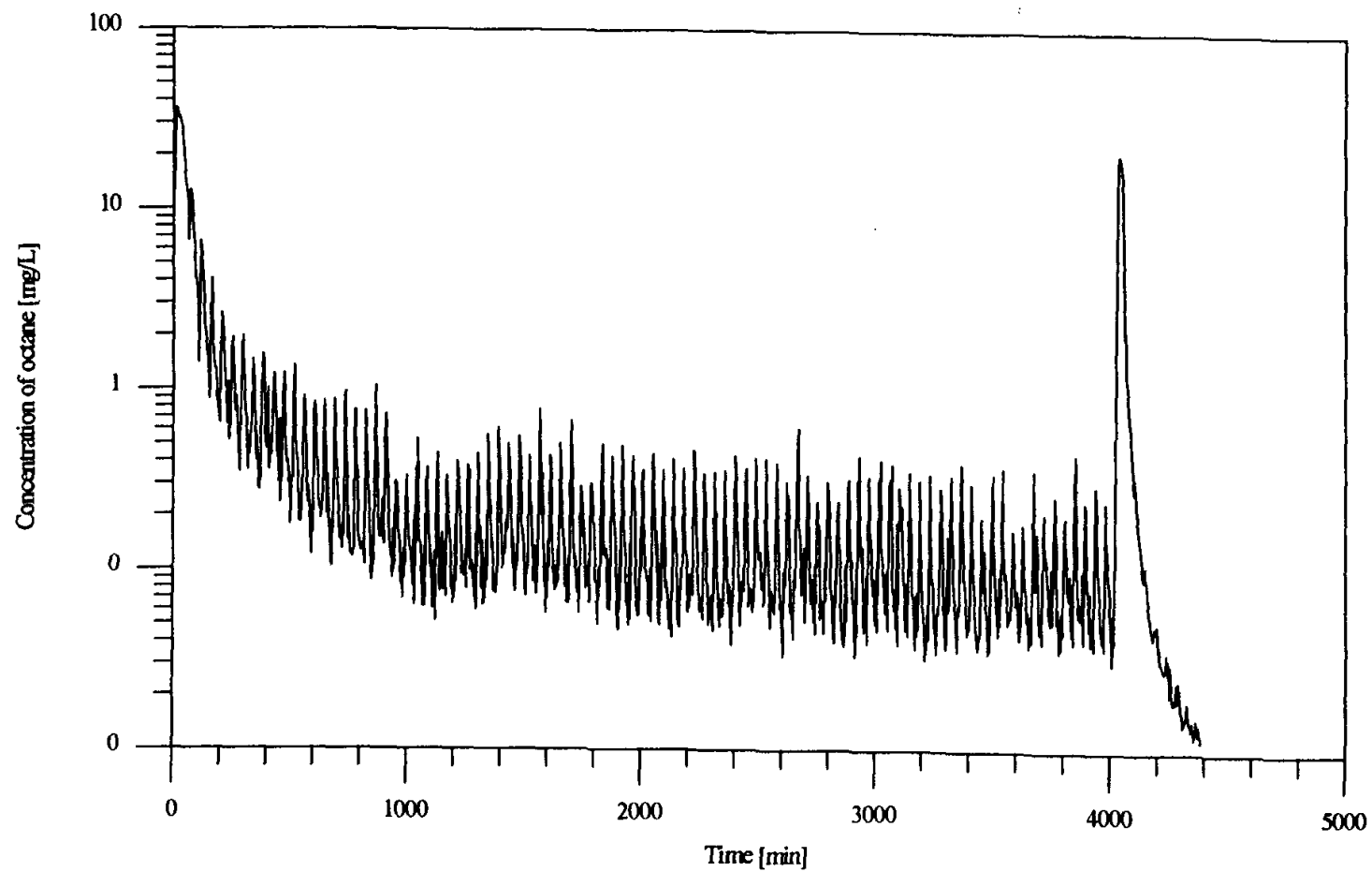
Figure 4.16: Octane concentration in the outlet air of the physical model vs. time for Q_{air} = 10 \text{ L/min} pulsed injection and M^f = 35.14 \text{ g.} , final wet medium experiment. Draining of the physical model occurred at 4016 min
