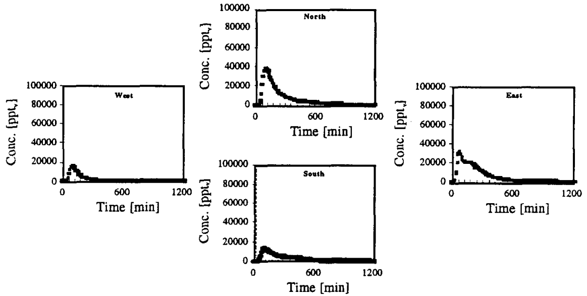
Figure SF-9. Directional soil vapor extraction well response to 0.5 mL injection of SF 6 into the air injection well; flow per extraction well ≈8 ft 3 /min; injection well flow 5 ft 3 /min (10/26 - 10/28/96).
