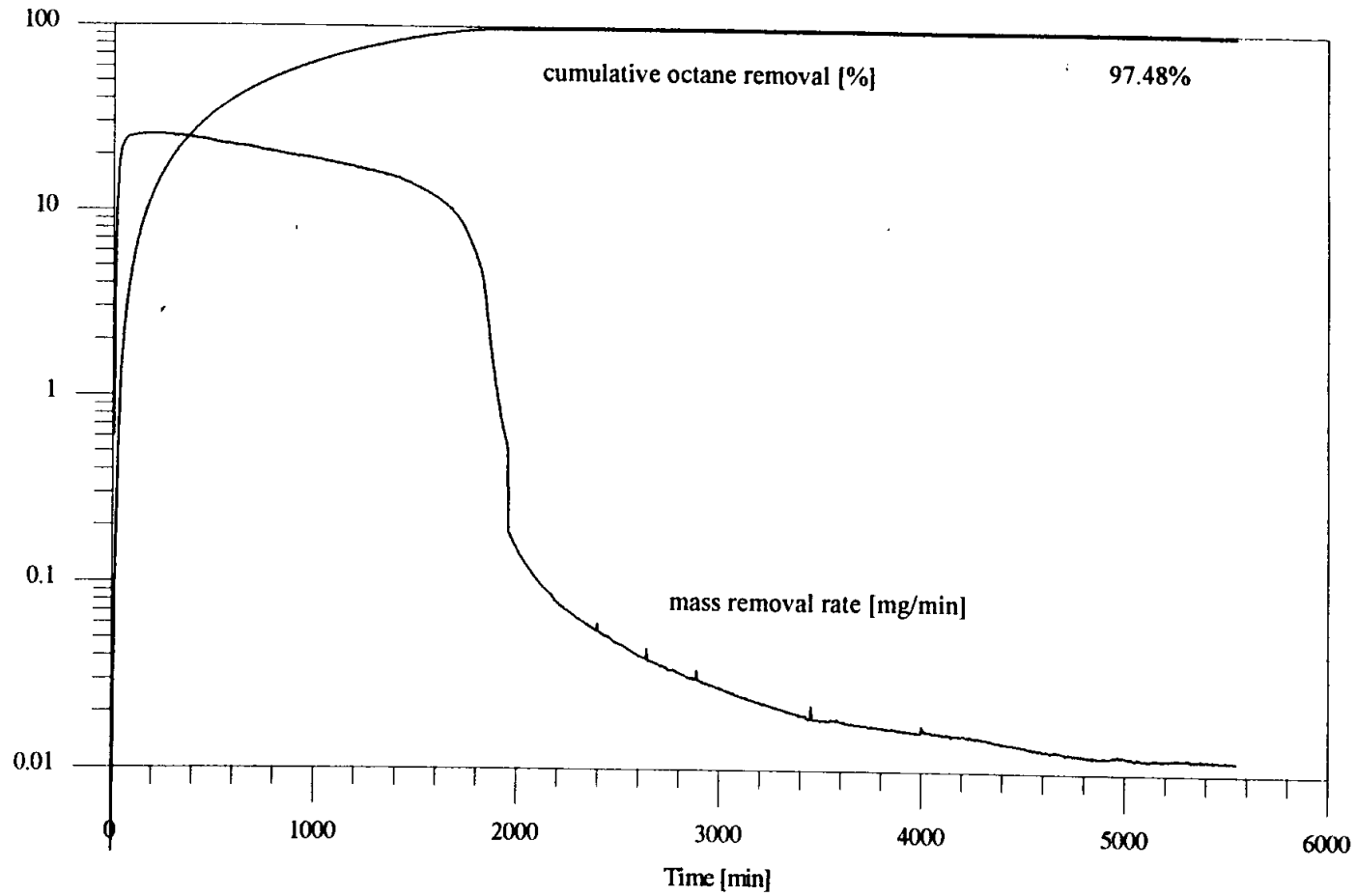
Figure 5.3: Mass removal rate and cumulative octane removal vs. time for Q_{air} = 1.25 L/min steady injection and M^f = 35.14 g., intermediate dry medium experiment.
