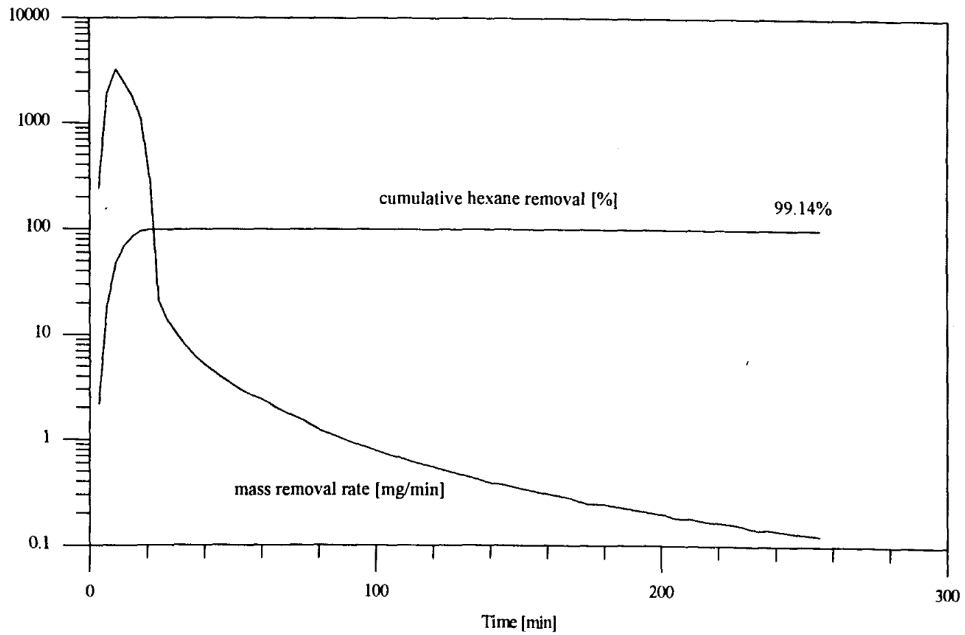
Figure 5.20: Mass removal rate and cumulative hexane removal vs. time for Q_{air} = 10 L/min steady injection and M^p = 33 g., intermediate dry medium experiment.
