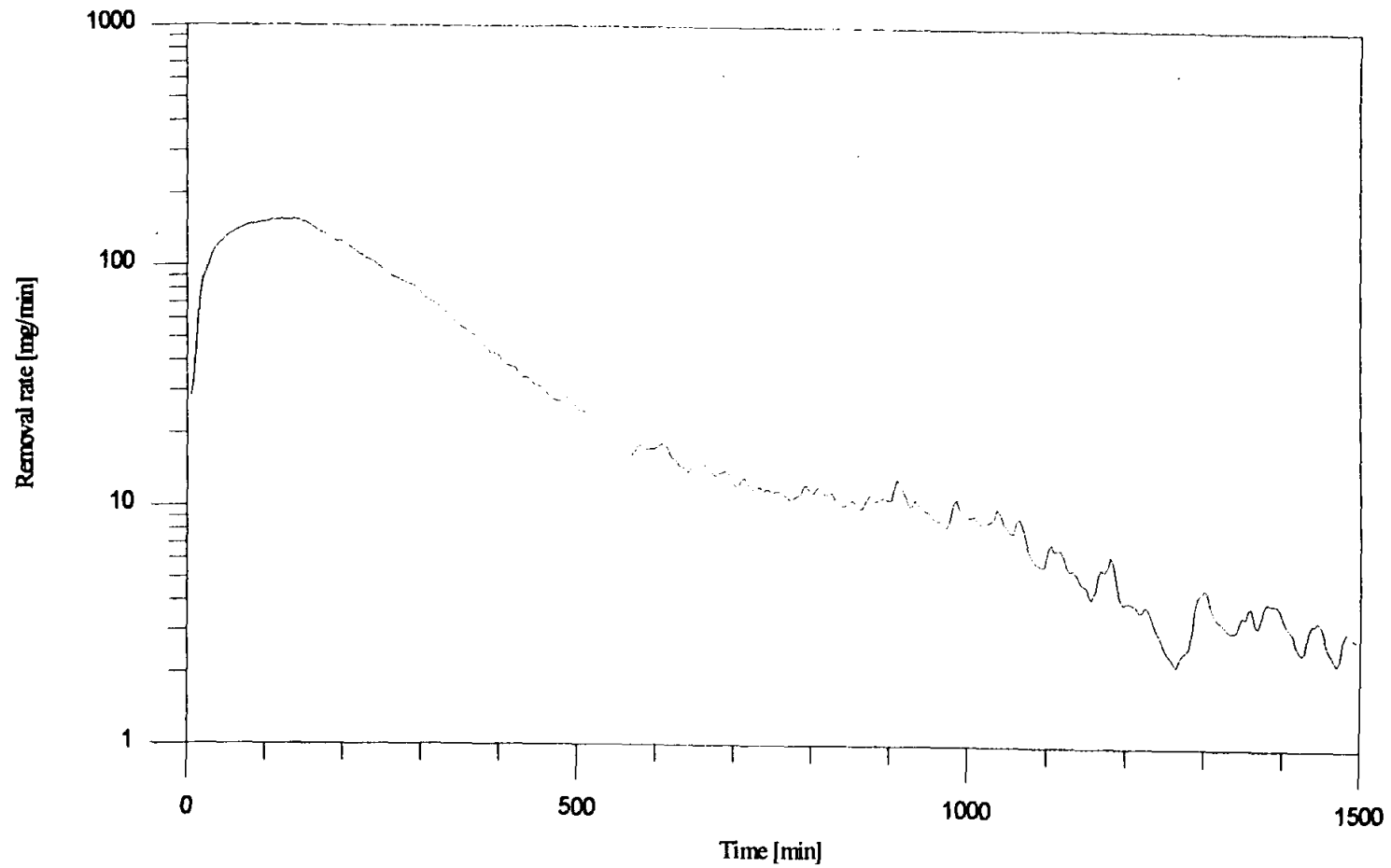
Figure 5.18: A close look at the short term removal rate of octane vs. time for Q_{air} = 1.25 L/min steady injection and M^0 = 35.14 g.
