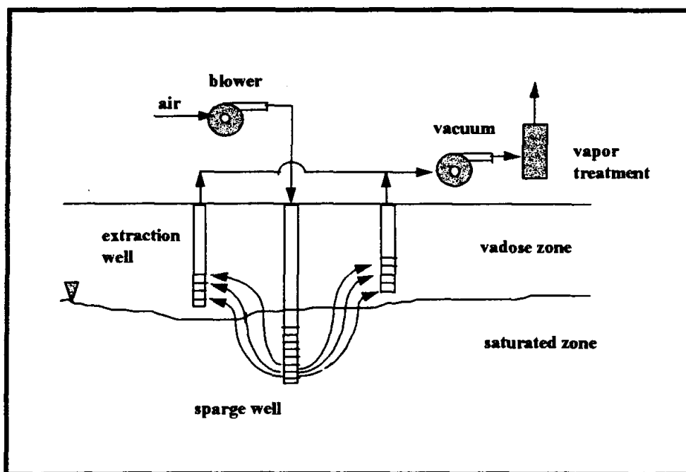
Figure 1.2: Schematic of an air sparging system.
