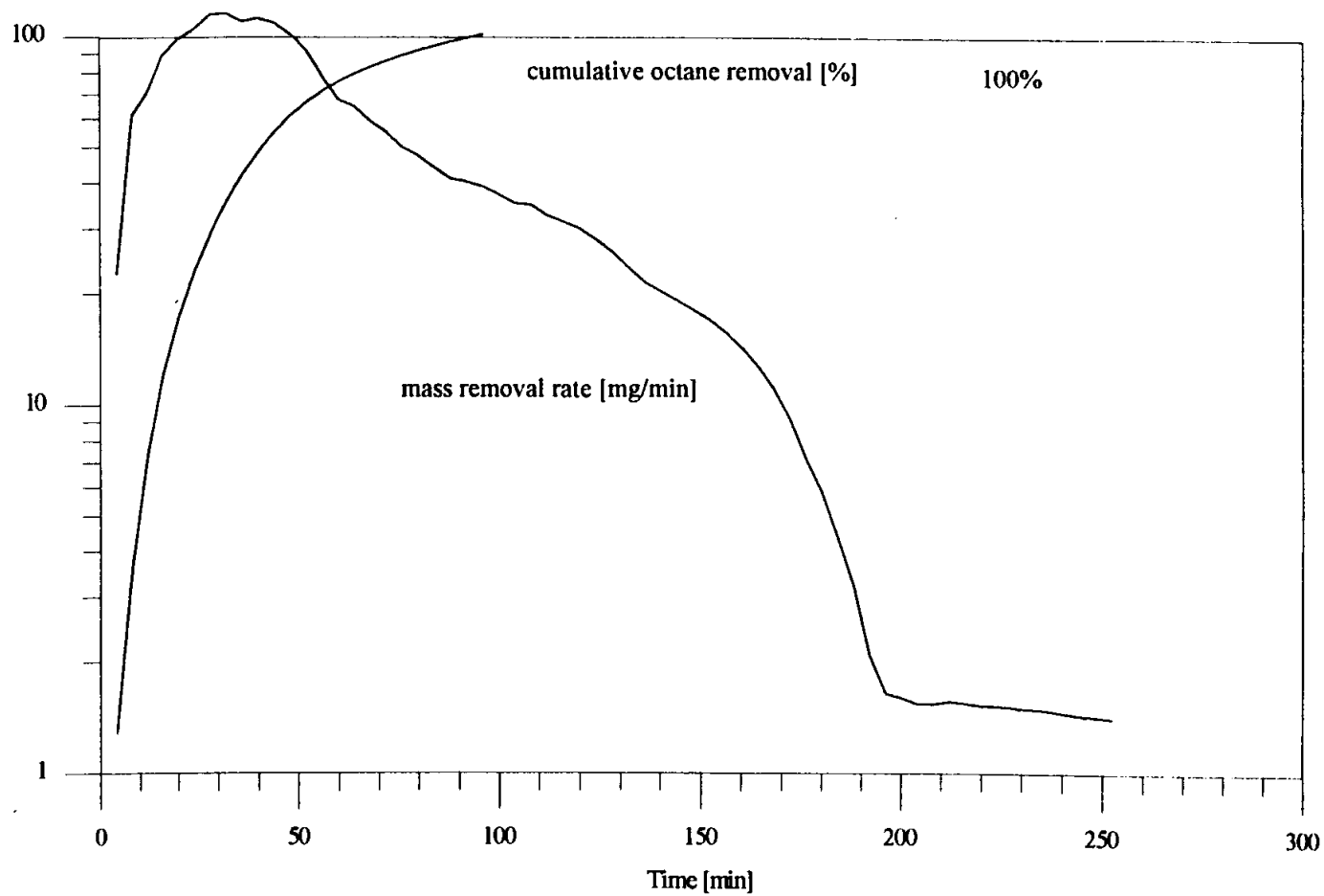
Figure 5.2: Mass removal rate and cumulative octane removal vs. time for Q_{air} = 11 L/min steady injection and M^0 = 7.03 g., preliminary dry medium experiment.
