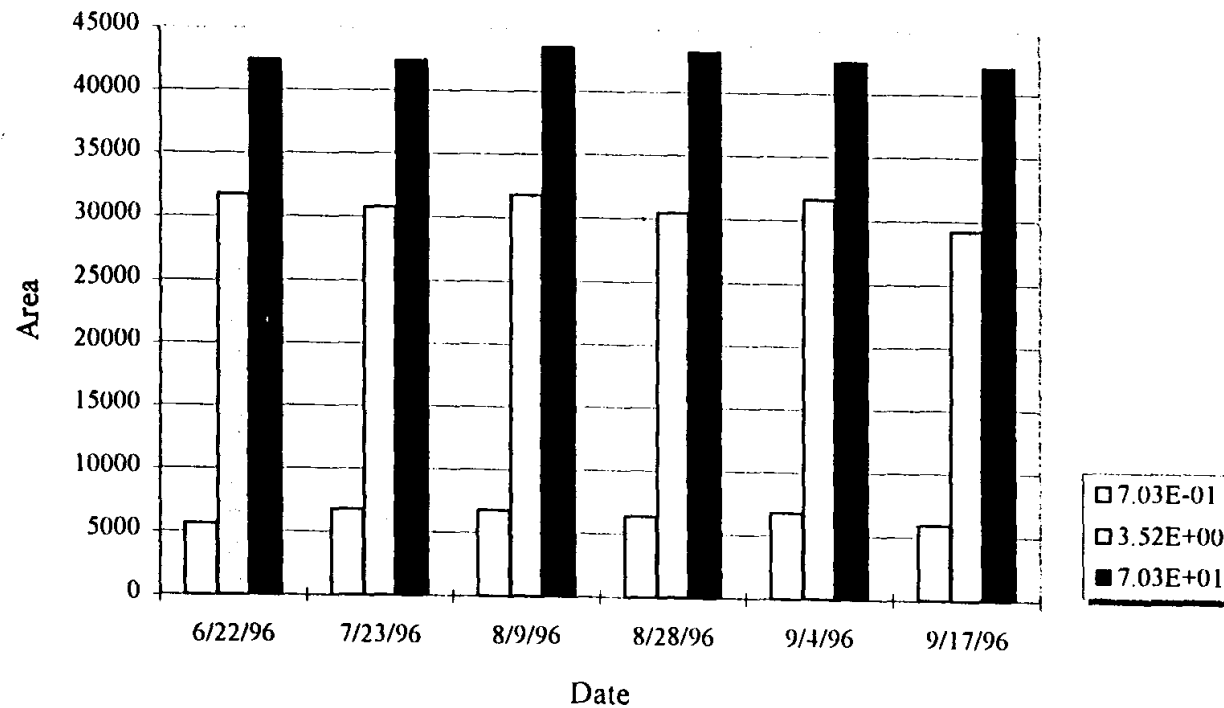
Figure 3.3: Result of standard run for octane on different dates. The sensitivity of the gas chromatograph was set at "high". Octane concentration for standard run were 7.03E-01, 3.52E+00 & 7.03E+01 mg/L-air.
