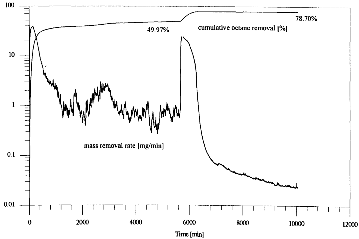
Figure 5.9: Mass removal rate and cumulative octane removal vs. time for Q_{air} = 1.25 L/min steady injection and M^f = 35.14 g., final wet medium experiment. Draining of the physical model occurred at 5656 min.
