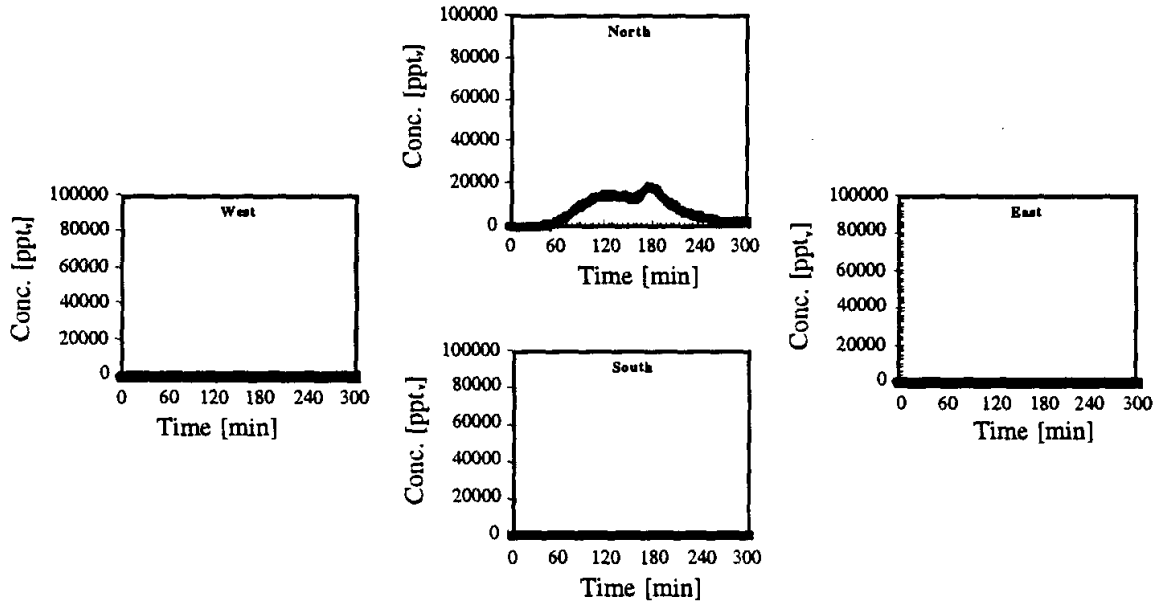
Figure SF-7. Directional soil vapor extraction well response to 0.5 mL injection of SF 6 into MP-6 (8-ft below ground surface); vapor extraction system only; flow per well 8 - 10 ft 3 /min (9/8/96).
