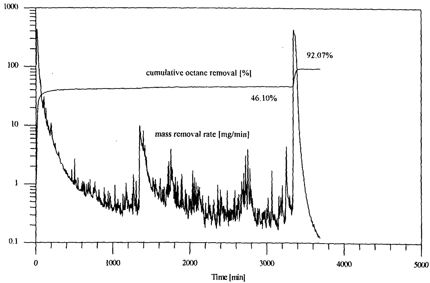
Figure 5.12: Mass removal rate and cumulative octane removal vs. time for Q_{air} = 10 L/min steady injection and M^0 = 35.14 g., final wet medium experiment. Draining of the physical model occurred at 3335 min.
