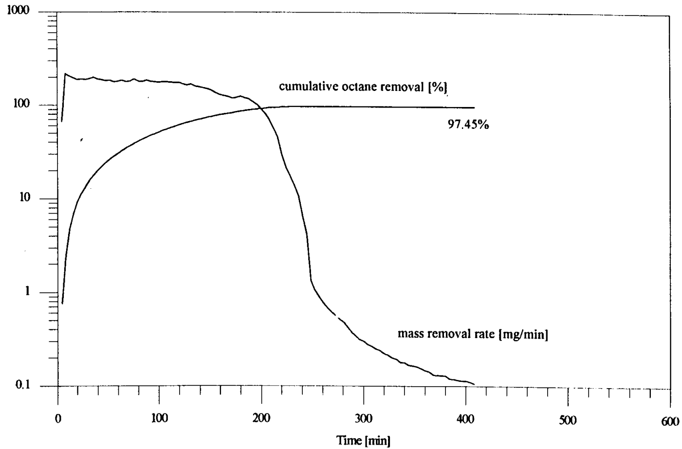
Figure 5.4: Mass removal rate and cumulative octane removal vs. time for Q_{air} = 10 L/min steady injection and M^f = 35.14 g., intermediate dry medium experiment.
