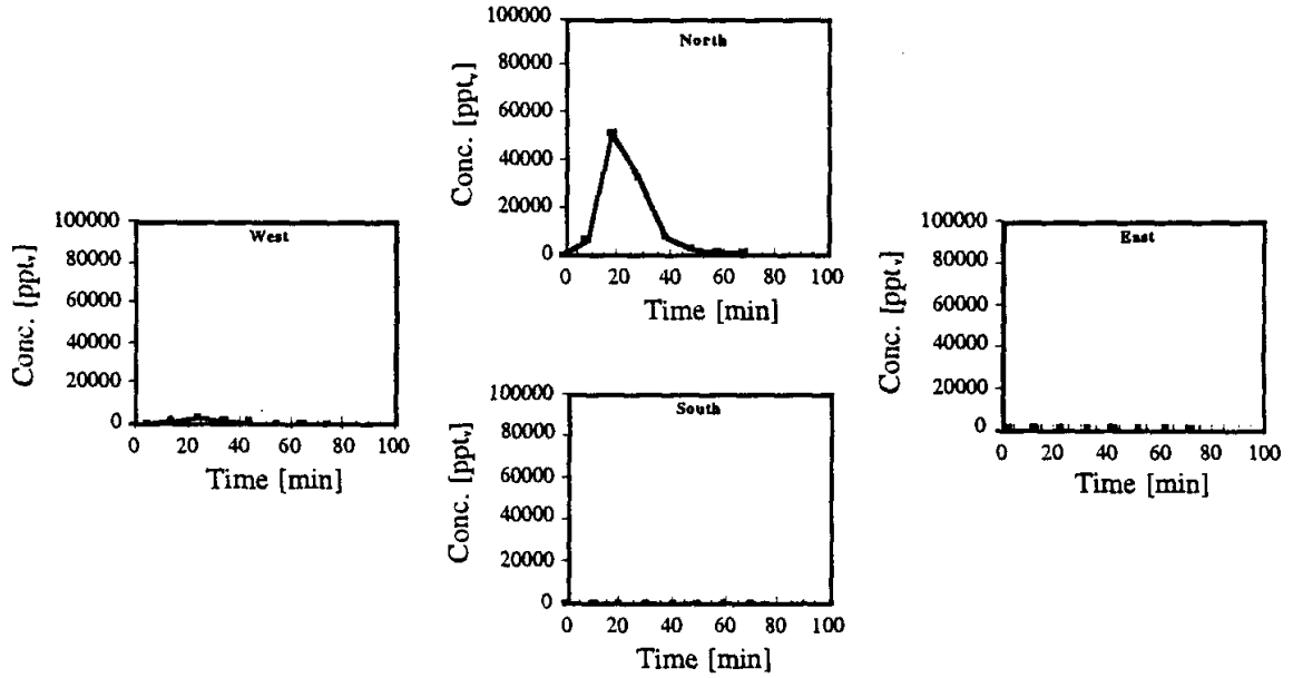
Figure SF-11. Directional soil vapor extraction well response to 0.5 mL injection of SF 6 into MP-6 (4-ft below ground surface); vapor extraction system with air injection; flow per extraction well ≈8 ft 3 /min; injection well flow 5 ft 3 /min (10/28/96).
