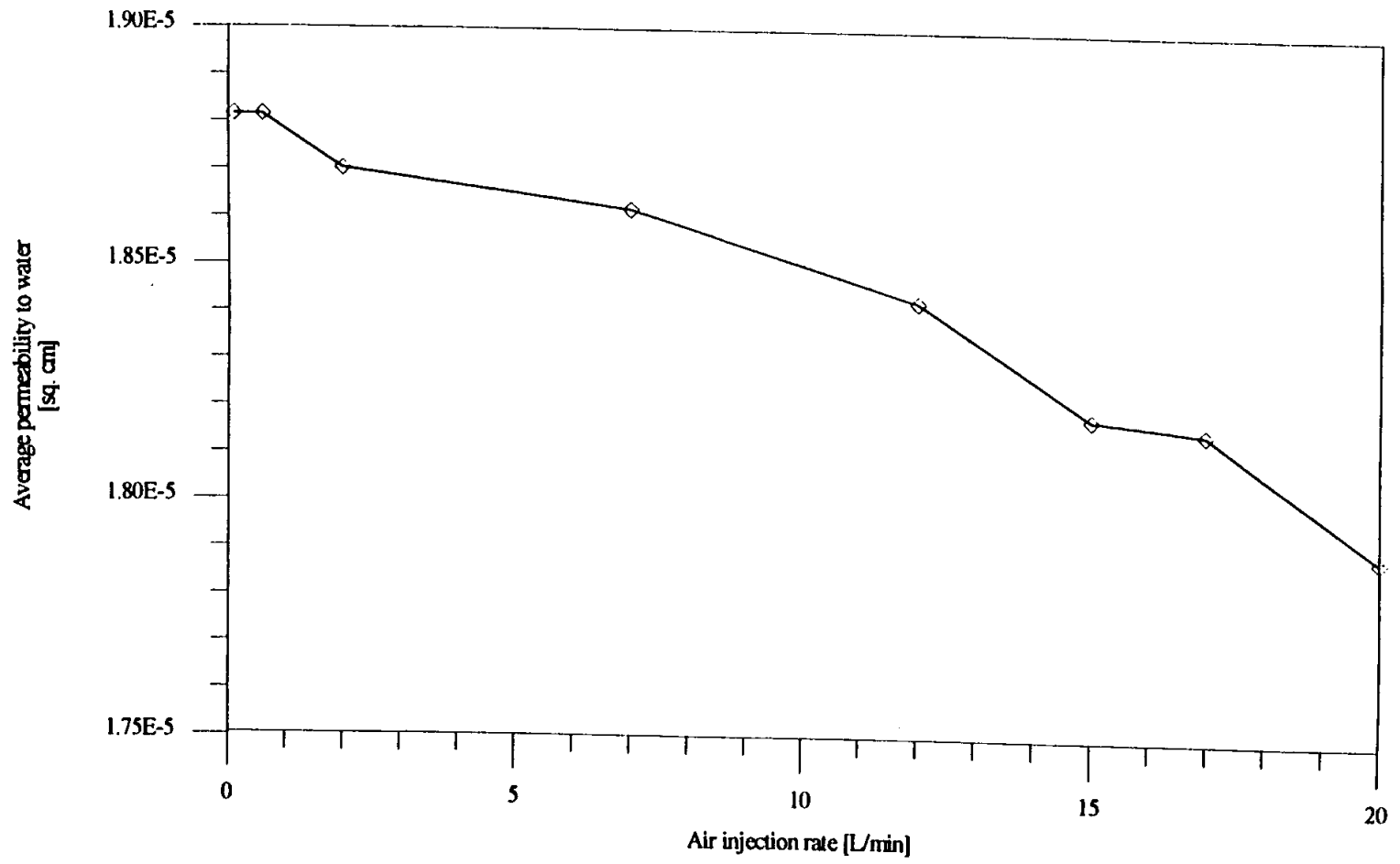
Figure A4: Average permeability vs. air injection rate for a layered system.
