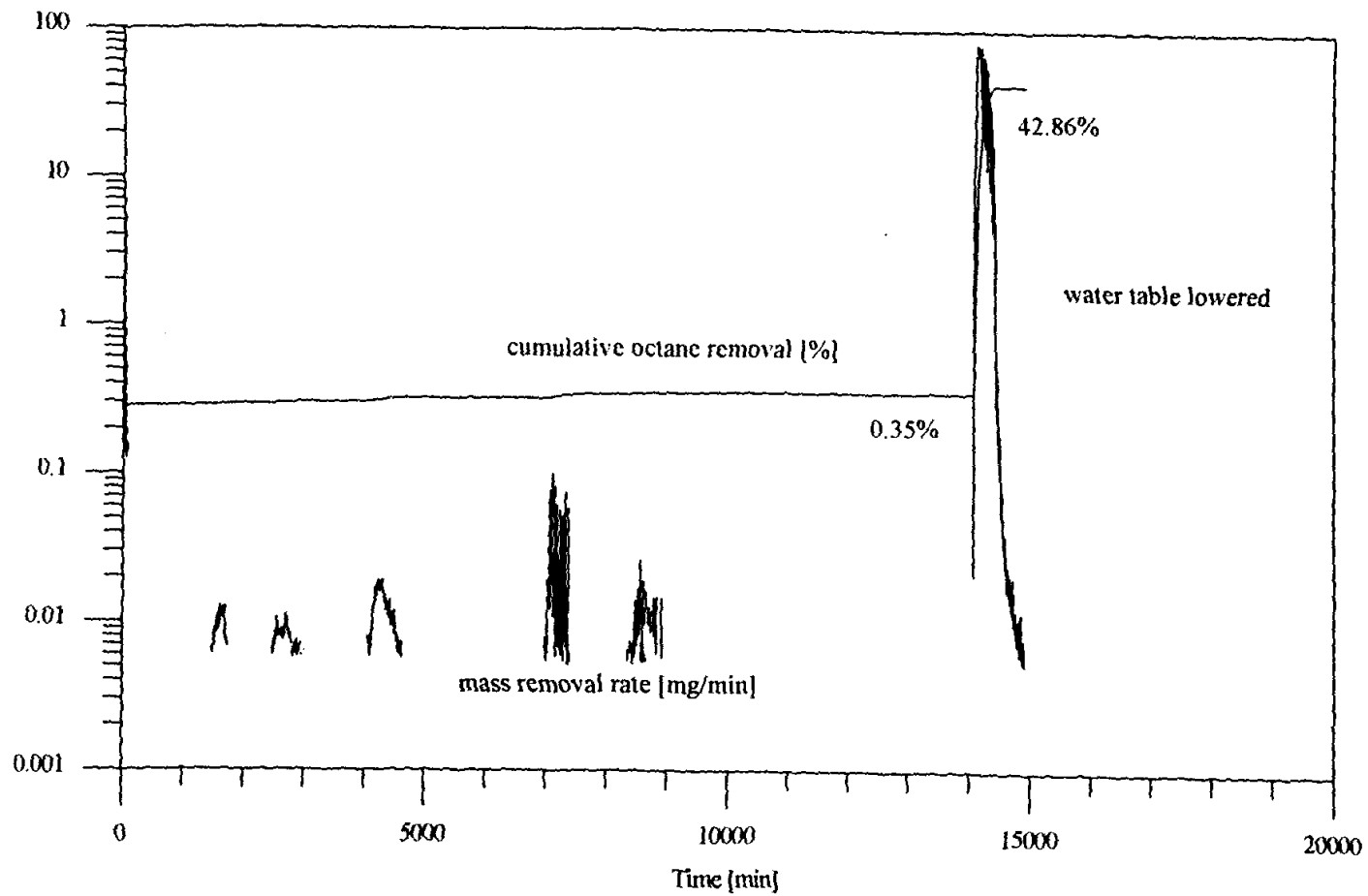
Figure 5.24: Mass removal rate and cumulative octane removal vs. time for Q_{air} = 10 L/min both steady pulsed injection and M = 35.14 g, final wet medium experiment. Draining of the physical model occurred at 14012 min.
