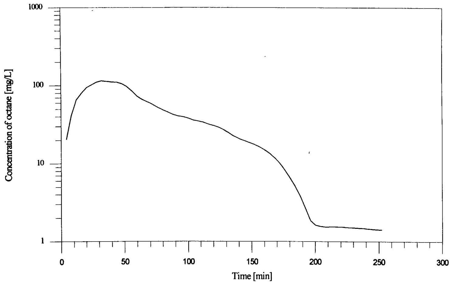
Figure 4.2: Octane concentration in the outlet air of the physical model vs. time for Q_{air} = 11 L/min steady injection and M = 7.03 g., preliminary dry medium experiment.
