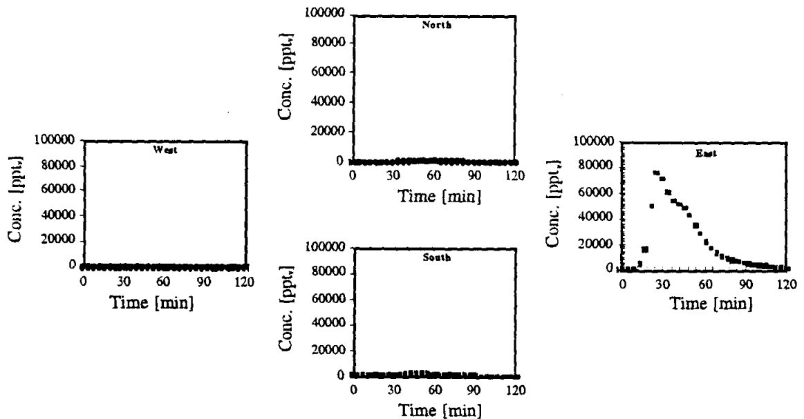
Figure SF-4. Directional soil vapor extraction well response to 0.5 mL injection of SF 6 into MP-4 (4-ft below ground surface); vapor extraction system only; flow per well 8 - 10 ft 3 /min (9/8/96).
