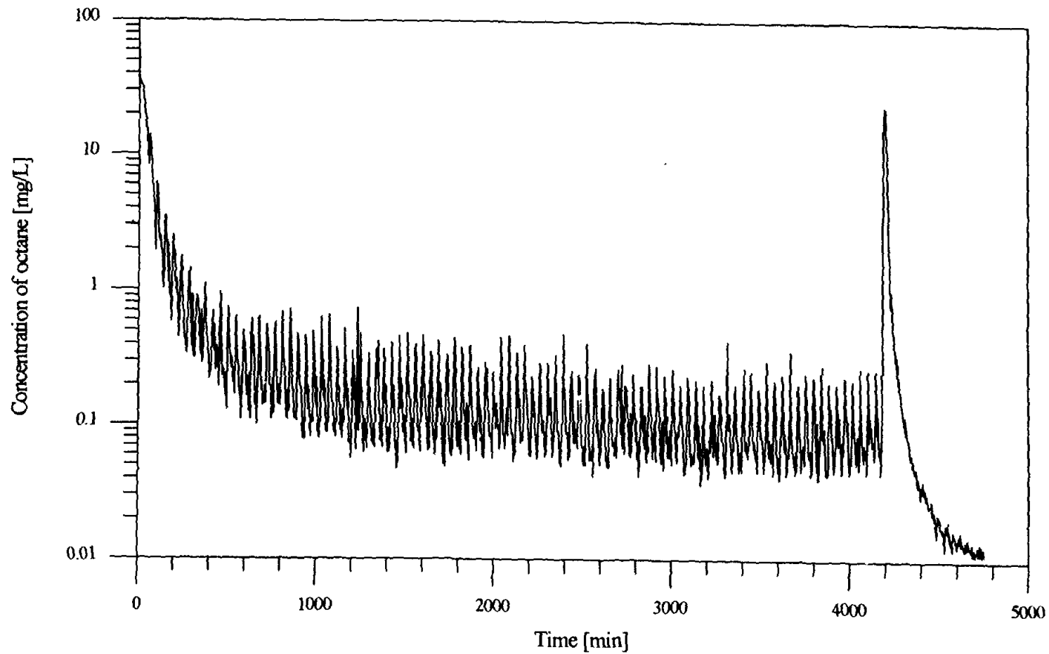
Figure 4.17: Octane concentration in the outlet air of the physical model vs. time for Q_{air} = 10 L/min pulsed injection and M^p = 35.14 g., final wet medium experiment. Draining of the physical model occurred at 4184 min
