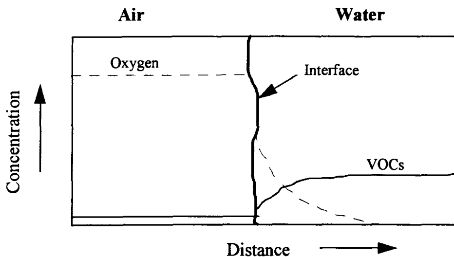
Figure 2.2: Conceptual model of oxygen and contaminant distributions in the vicinity of an air flow channel.
