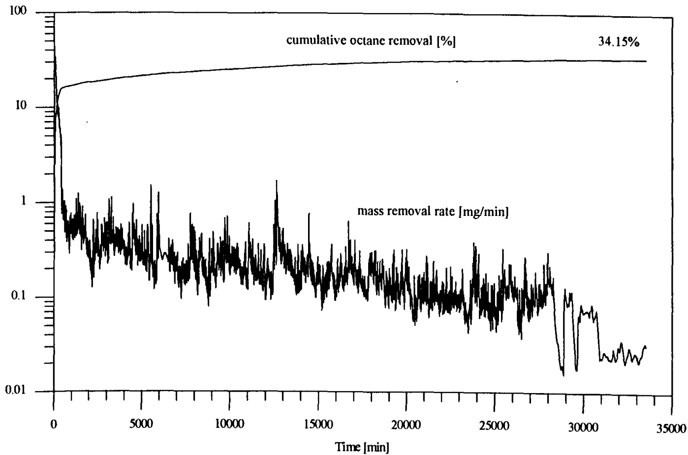
Figure 5.7: Mass removal rate and cumulative octane removal vs. time for Q_{air} = 1.25 L/min steady injection and M^P = 35.14 g., intermediate wet medium experiment.
