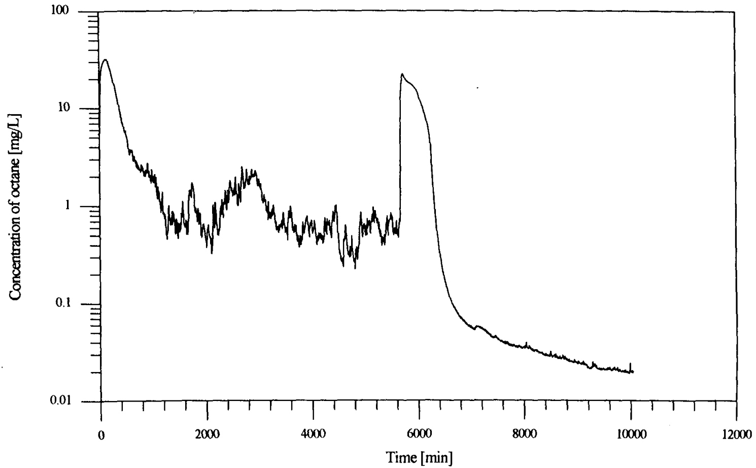
Figure 4.11: Octane concentration in the outlet air of the physical model vs. time for Q_{air} = 1.25 L/min steady injection and M^f = 35.14 g., final wet medium experiment. Draining of the physical model occurred at 5656 min
