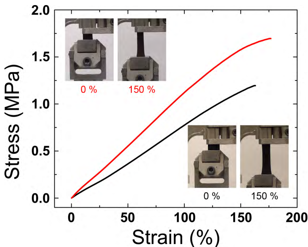
Figure 4. Stress/strain curves for small-grain (red) and large-grain (black) hollow iron oxide nanostructure polymer composites with 60 wt% nanoparticle loading. The images of elongated composites are shown as an inset.
