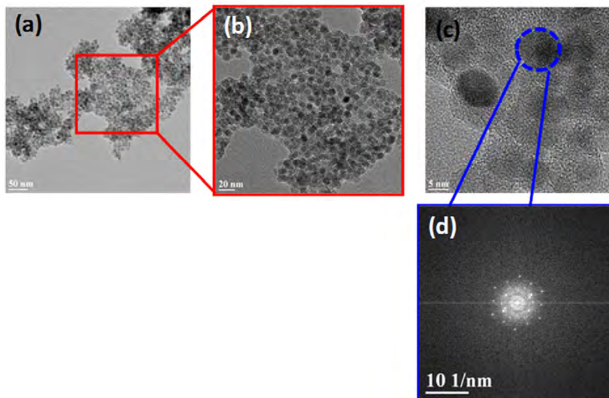
Figure 6. TEM images and FFT analysis from PyDop1- \gamma\text{-Fe}_2\text{O}_3 . (a)-(c) progressive magnification of nanoparticles immobilized on rGO platelet (d) FFT on nanoparticle in the composite showing crystalline character.
