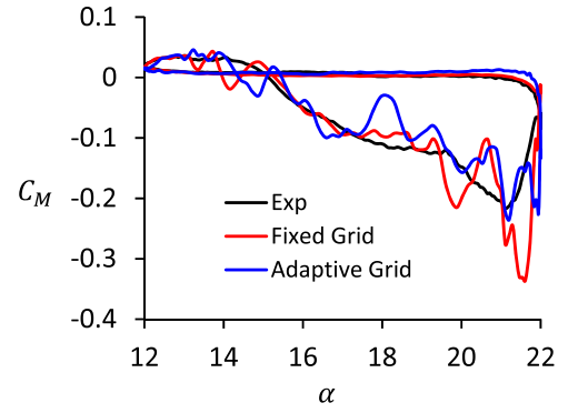
(a) r/R = 0.5
