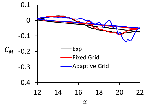
(c) r/R = 0.95
