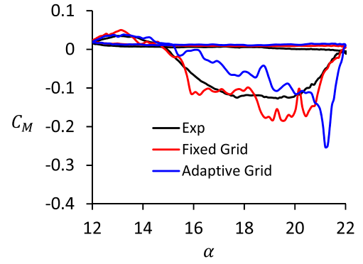
(b) r/R = 0.8
