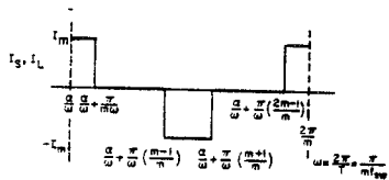
Fig. 5. Single Phase Current Source Waveform for an m-phase ICB Circuit.
