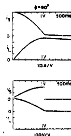
Fig. 10. Experimental Average Coil Voltage and Current Traces.
