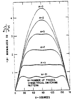
Fig. 6. Plot of <p> vs α.
