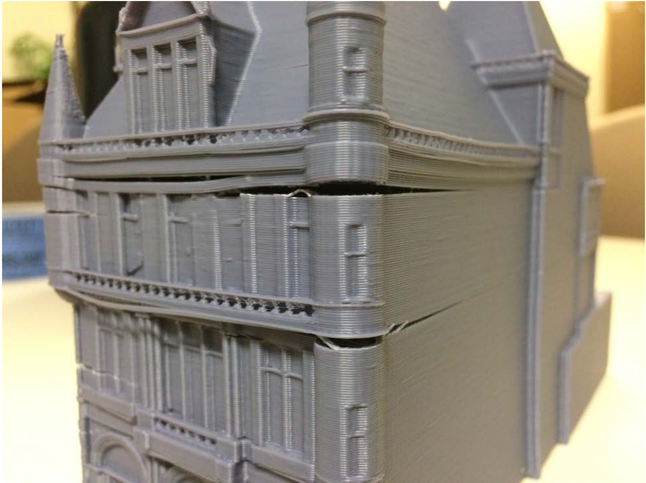
Figure 38: The surface detail of Vanderbilt mansion shows cracking and delamination, likely as a result of thermal stresses and poor layer adhesion at fast print speeds without optimized or adjusted temperature parameters.
