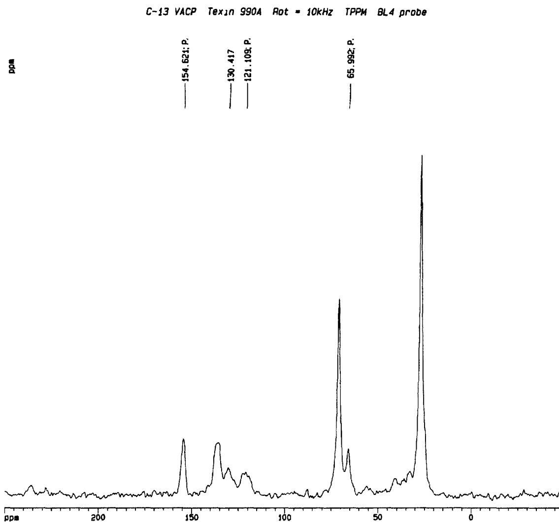
Figure 11. – Solid state ^{13}\text{C} NMR spectrum of Texin 990A. The spectrum was acquired using cross polarization with magic angle spinning and high power proton decoupling.
