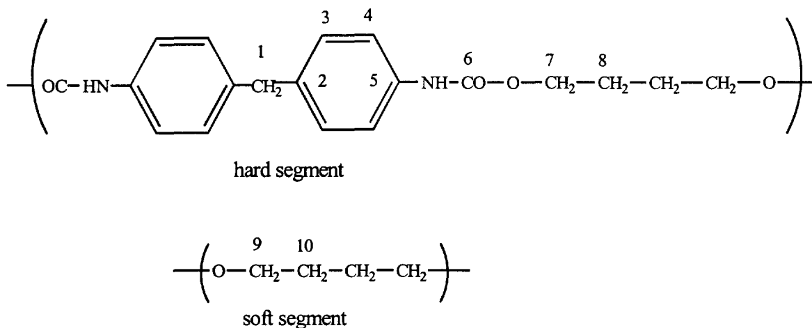
Figure 8. – Structures of the hard and soft segments of the MDI/butanediol/poly(tetramethylene ether glycol) poly(ether)urethanes. The numbers refer to carbons in unique chemical environments.
