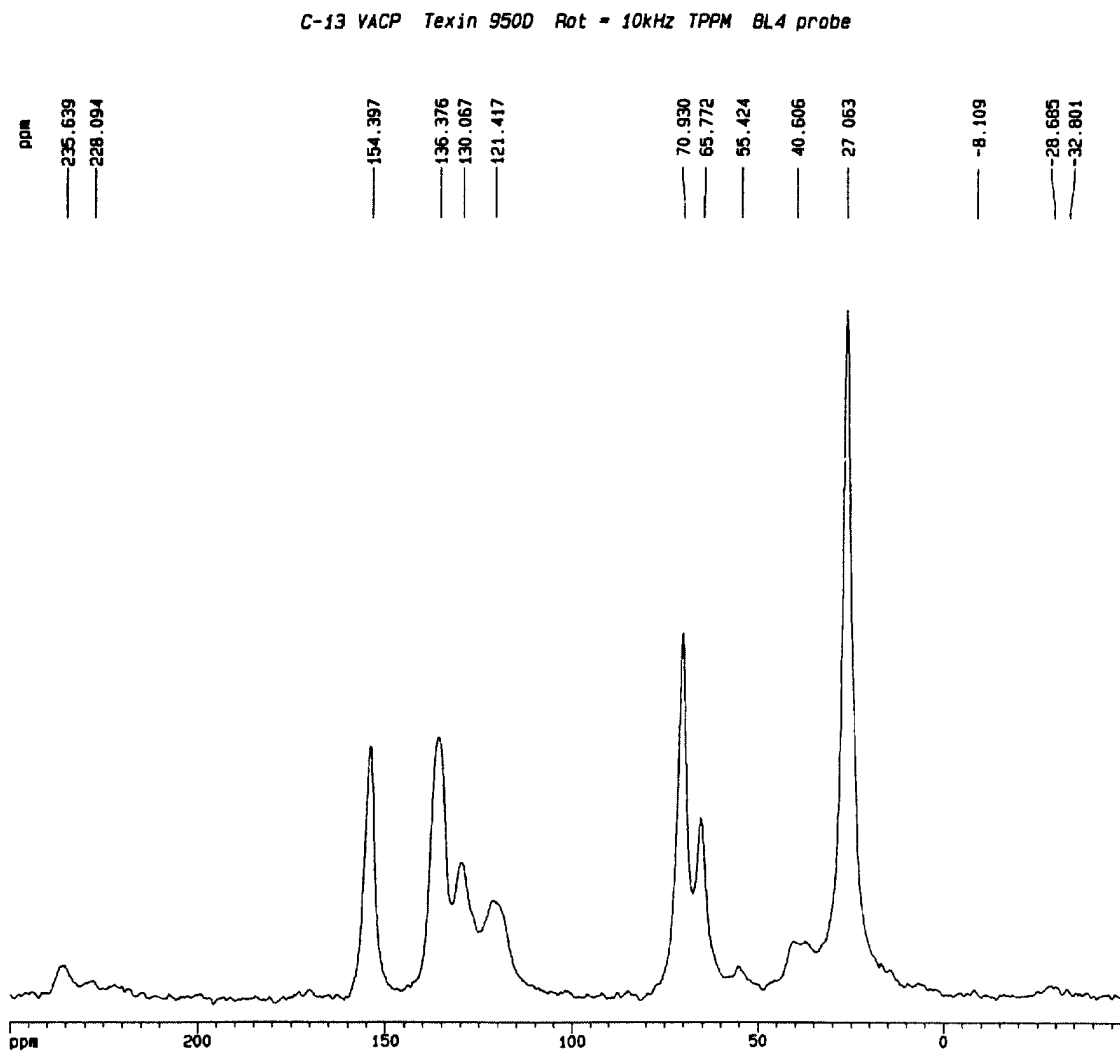
Figure 12. – Solid state ^{13}\text{C} NMR spectrum of Texin 950D. The spectrum was acquired using cross polarization with magic angle spinning and high power proton decoupling.
