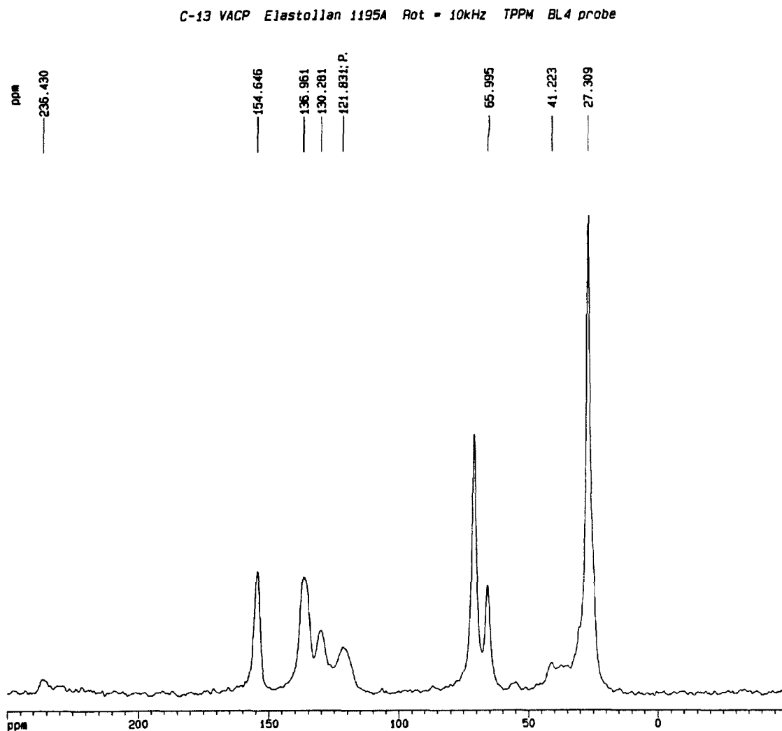
Figure 14. – Solid state ^{13}\text{C} NMR spectrum of Elastollan 1195A. The spectrum was acquired using cross polarization with magic angle spinning and high power proton decoupling.
