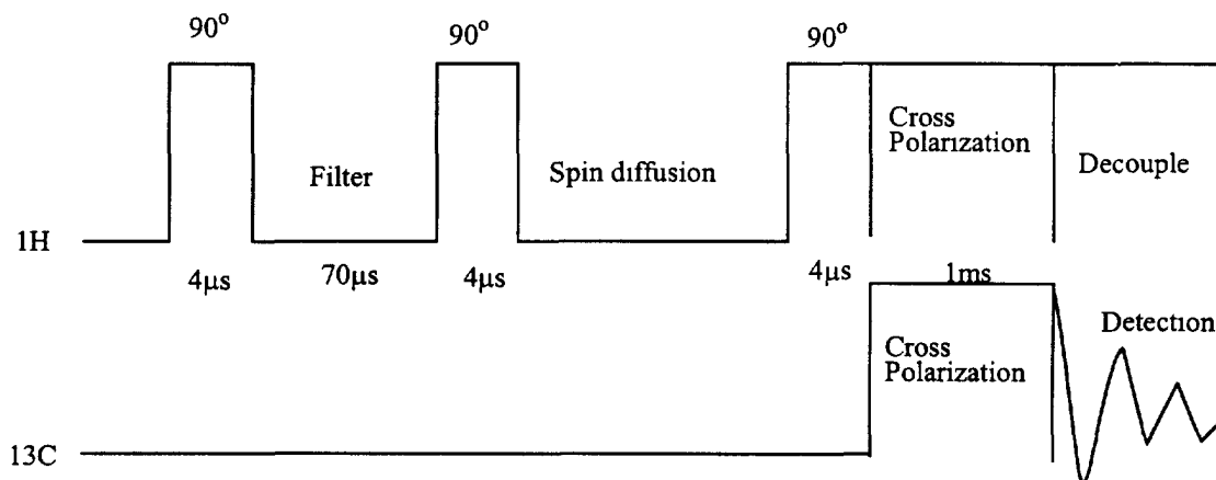
Figure 1. Goldman-Shen pulse sequence. The dephasing delay of 70 ms was followed by 12 cross-relaxation delays.
