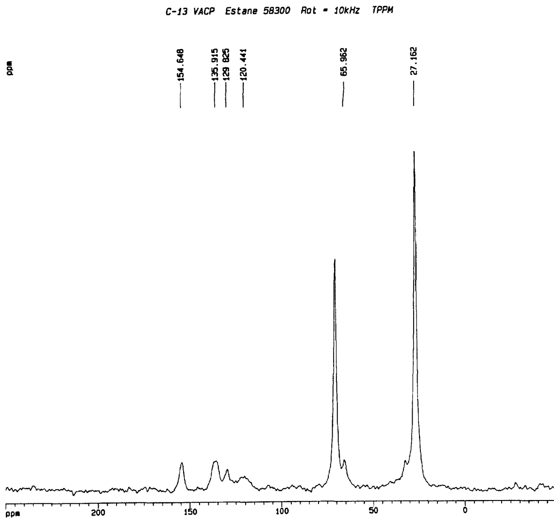
Figure 16. – Solid state ^{13}\text{C} NMR spectrum of Estane 58300. The spectrum was acquired using cross polarization with magic angle spinning and high power proton decoupling.
