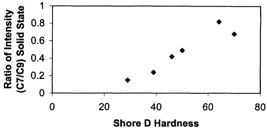
Figure 17. – Plot of the ratio of intensity of carbons C-7 and C-9 against Shore Type D Durometer hardness for the six TPEs.
