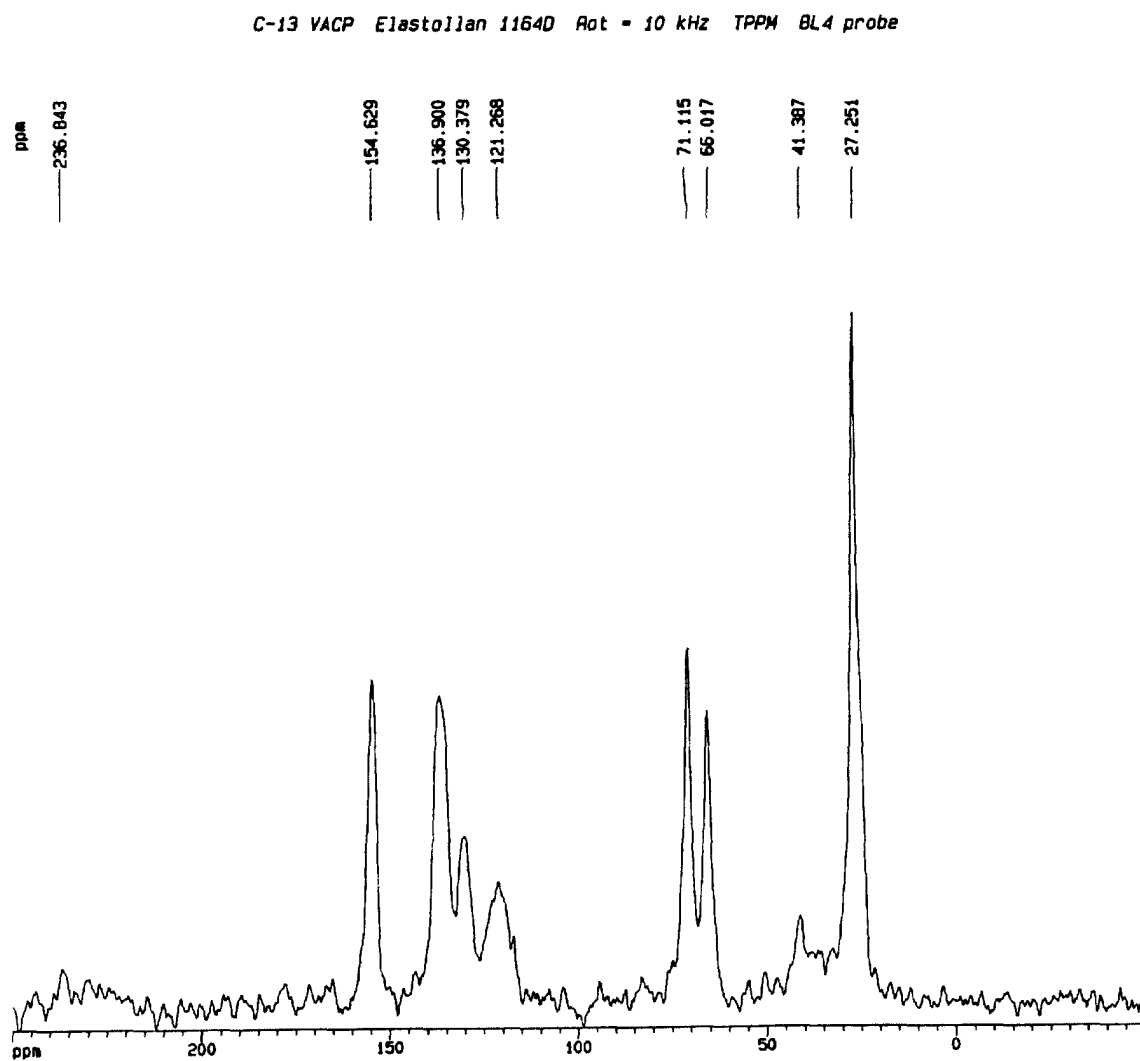
Figure 15. – Solid state ^{13}\text{C} NMR spectrum of Elastollan 1164D. The spectrum was acquired using cross polarization with magic angle spinning and high power proton decoupling.
