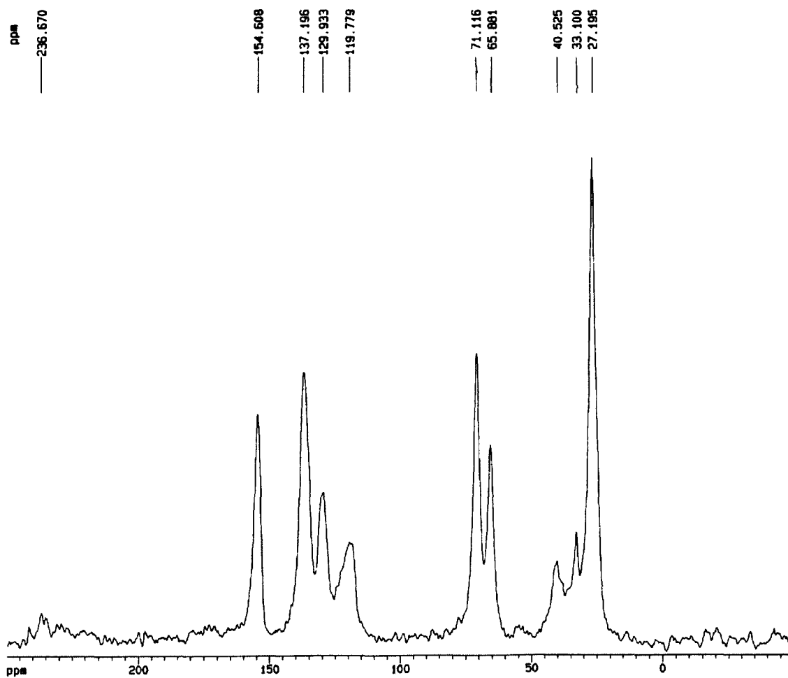
Figure 13. – Solid state ^{13}\text{C} NMR spectrum of Texin 970D. The spectrum was acquired using cross polarization with magic angle spinning and high power proton decoupling.
