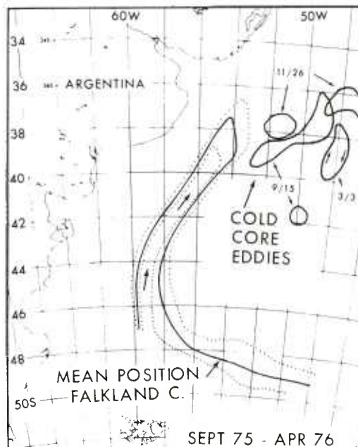
Fig. 5. The mean position of the boundaries of the cold water associated with the Falkland Current was determined from the sea surface temperature fronts apparent in the i.r. images from September 1975 to April 1976 (Table 1). The maximum deviation of the SST fronts from the mean is indicated by the dots. The shapes of the cold core eddies indicated in Table 1 are also illustrated.
