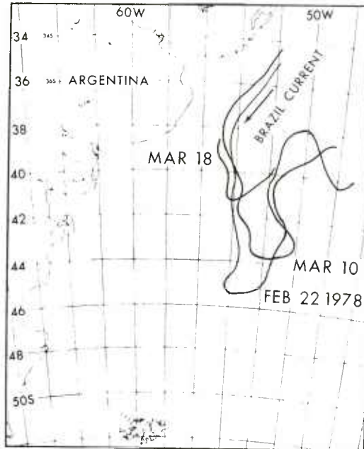
Fig. 7. The three positions of the boundaries of the warm water associated with the Brazil Current suggest an apparent northward displacement of the southern limit of the warm water between 22 February and 18 March 1978. During this interval two warm core eddies separated from the Brazil Current (Figs 10, 11).
