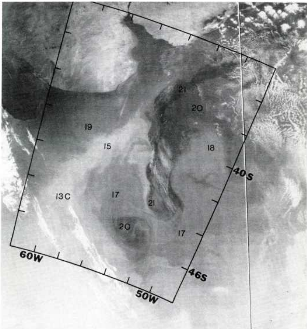
Fig. 4. The VHRR i.r. image was recorded on orbit 7283 by NOAA-5 on 10 March 1978. The darker shades of gray represent the warmer water. Selected temperatures recorded at the satellite are shown. The colder water associated with the Falkland Current warms northward from 13 to 15°C. Wave-like meanders are evident along the western SST boundary associated with the Brazil Current. A recently formed warm core eddy appears at 45° S and 53° W (Fig. 10).
