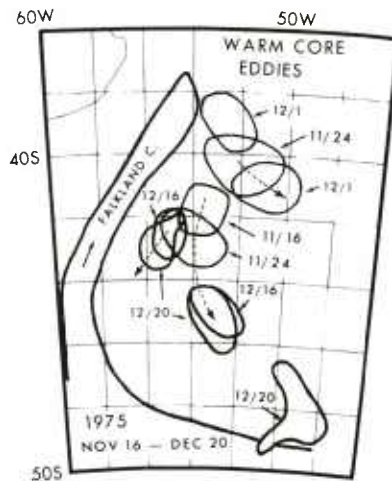
Fig. 15. The mean SST boundary associated with the Falkland Current and the position of the warm core eddies are shown between 16 November and 20 December 1975. Three of the eddies were displaced southward as indicated by the dashed lines. The eddies observed on 20 December also appear in the i.r. image in Fig. 2.
