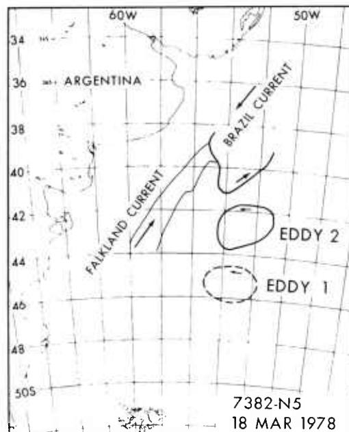
Fig. 11. The SST boundaries associated with the Falkland Current, the Brazil Current, and two warm core eddies are shown on 18 March 1978 based on VHRR i.r. image from orbit 7382 on NOAA-5. EDDY 1 was partially cloud covered and its position is approximate.
