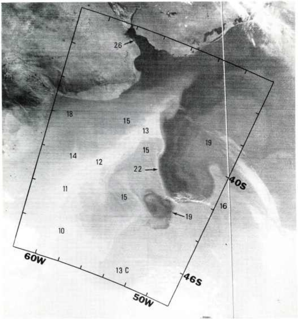
Fig. 3. The VHRR i.r. image was recorded on orbit 5339 by NOAA-4 on 16 January 1976. The darker shades of gray represent the warmer water. Selected temperatures recorded at the satellite are shown. The colder water associated with the Falkland Current increases northward in temperature from 10 to 13 °C. Wave-like meanders appear along the western SST boundary associated with the Brazil Current. A recently formed warm core eddy appears at 43° S and 52° W.
