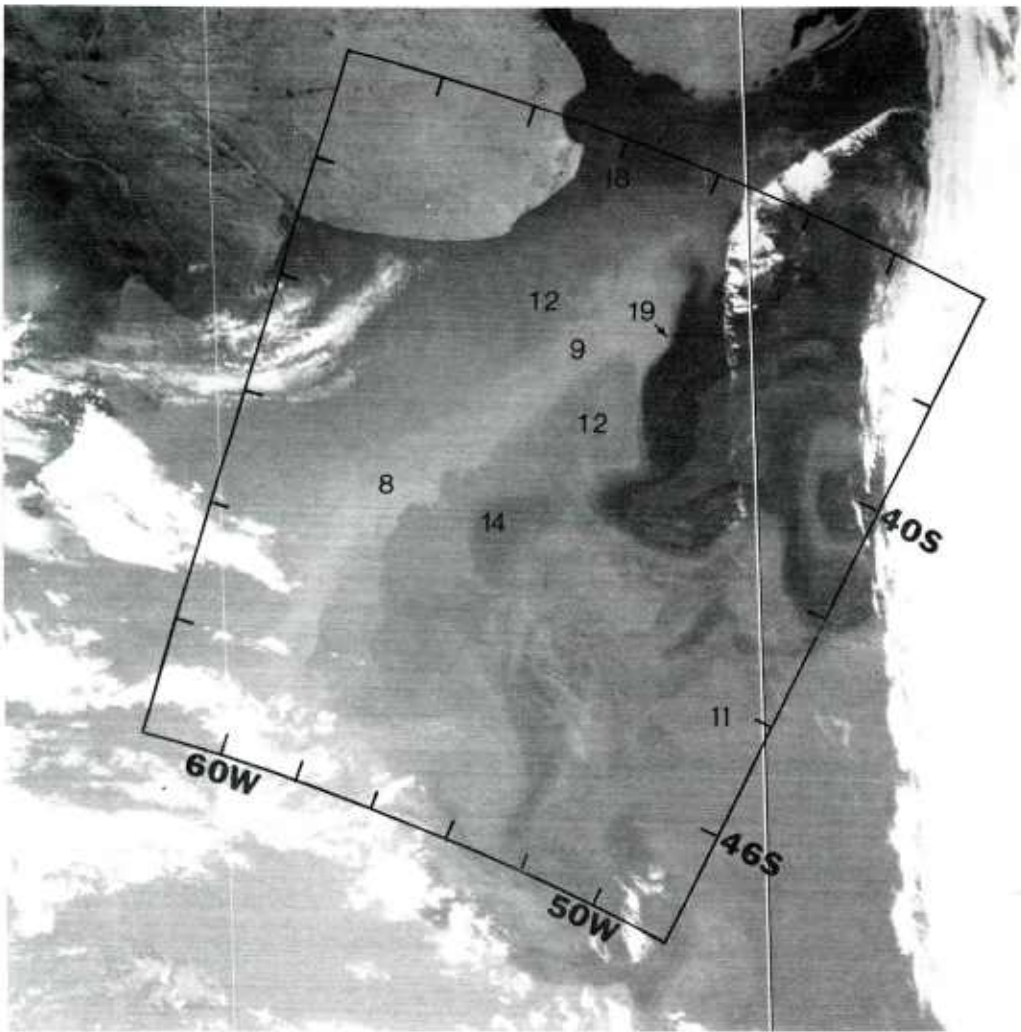
Fig. 2. The VHRR i.r. image was recorded on orbit 5001 by NOAA-4 on 20 December 1975. The darker shades of gray represent the warmer water. The warm water associated with the Brazil Current reaches 42 S before meandering eastward. At least three warm core eddies appear south of the Brazil Current (Fig. 15). Selected temperatures recorded at the satellite are shown. The temperature of the cold water associated with the Falkland Current increases northward from 8 to 9 C.
