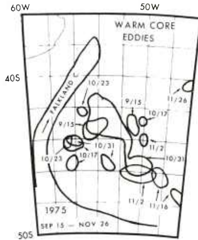
Fig. 14. The mean SST boundary associated with the Falkland Current and the position of the warm core eddies are shown between 15 September and 26 November 1975. Two eddies moved southward along 50°W from 17 October to 2 November and from 31 October to 2 November. Most of the other eddies are unique observations and their displacement was not established.
