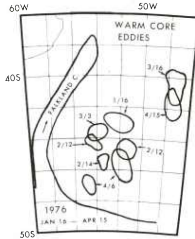
Fig. 16. The mean SST boundary associated with the Falkland Current and the position of the warm core eddies between 16 January and 15 April 1976 are shown. The eddy observed along 48°W on 16 March and 15 April may be the same eddy as well as the eddy observed on 16 January and 6 April along 52°W. The rest of the eddies appear to be unique.
