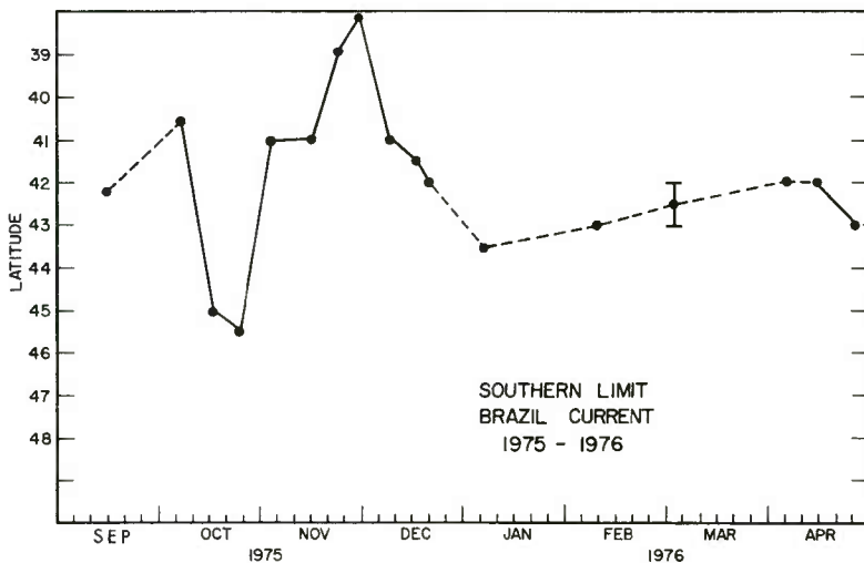
Fig. 17. The time series of the southern limit of the relatively warm water associated with the SST boundary of the Brazil Current from September 1975 to April 1976. At least six large warm core eddies formed south of the Brazil Current during October and November (Figs 14, 15). The measurement uncertainty in estimating the southern limit is indicated. The dashed line is used where sufficient observations were not available to resolve the fluctuations of the southern limit.
