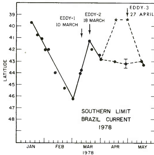
Fig. 8. A time series of the southern limit of the relatively warm water associated with the SST boundary of the Brazil Current from January to May 1978. The first two eddies formed after the southward displacement of the warm water during January and February. The dashed lines indicate the ambiguous interpretation of the southern limit due to cloud cover. EDDY 3 was observed only on 27 April. The measurement uncertainty in estimating the southern limit is indicated.
