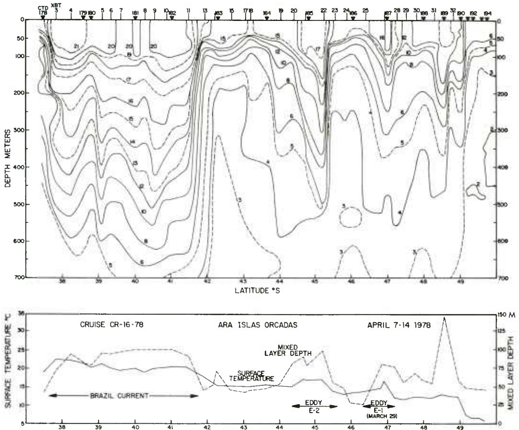
Fig. 18. Thermal structure of the upper 700 m along the track of the ARA Islas Orcadas cruise 16-78. The section is constructed from XBT observations 3 to 32 and CTD hydrographic Stas 178 to 194. The positions of EDDY 1 and EDDY 2 are taken from the last available satellite observation on 29 March 1978 (Fig. 12).
