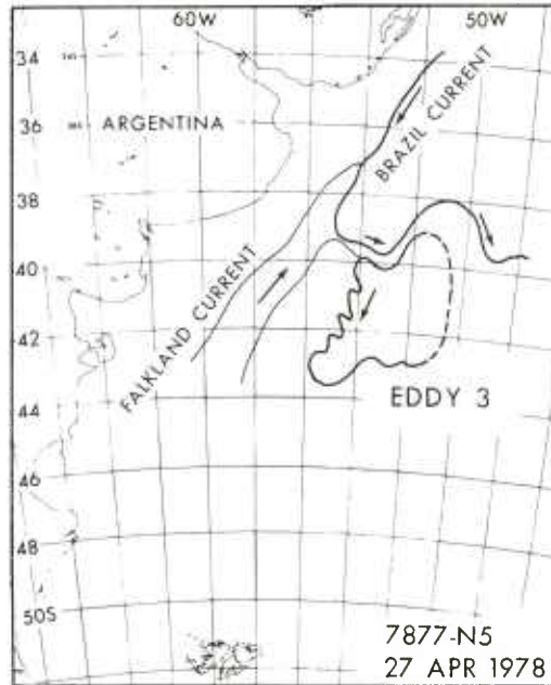
Fig. 13. The SST boundaries associated with the Falkland Current, the Brazil Current, and a large area of warm water, called EDDY 3, on 27 April 1978 are shown based on the VHRR i.r. image from orbit 7877 on NOAA-5. The eddy and the warm water associated with the Brazil Current appeared to be separated by a narrow filament of cold water associated with the Falkland Current.
