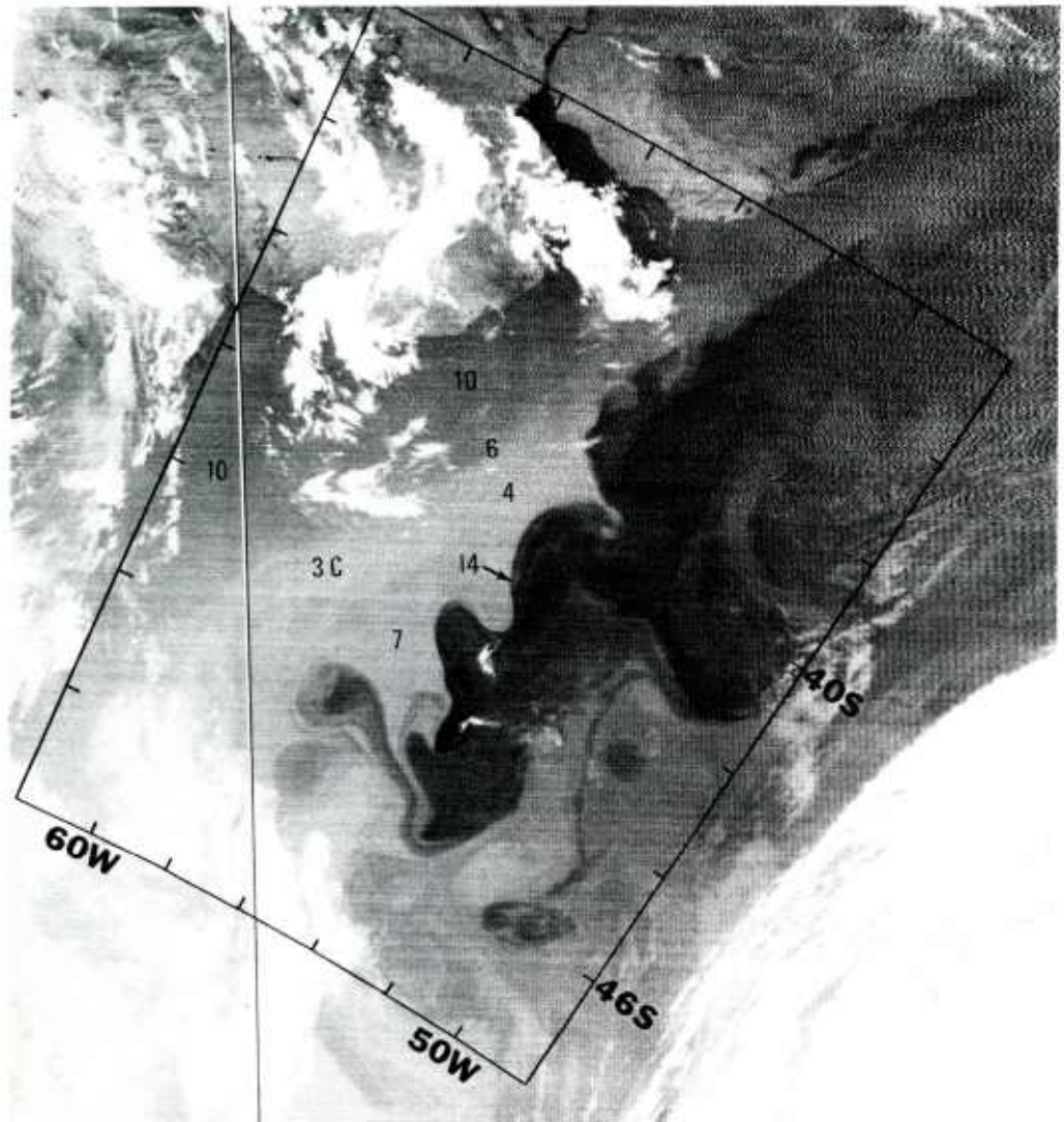
Fig. 1. The VHRR i.r. image was recorded on orbit 4200 by NOAA-4 on 17 October 1975. The darker shades of gray represent the warmer water. Wave-like meanders associated with the Brazil Current appear along the western SST boundary. Temperatures recorded at the satellite are shown. The temperature of the cold water associated with the Falkland Current increases northward from 3 to 4 C.
