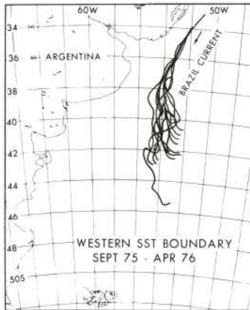
Fig. 6. The composite shows the positions of the western SST boundary associated with the Brazil Current from September 1975 to April 1976 as seen in the i.r. images tabulated in Table 1. The east-west displacement of the position of the boundary increases rapidly south of 36°S.
