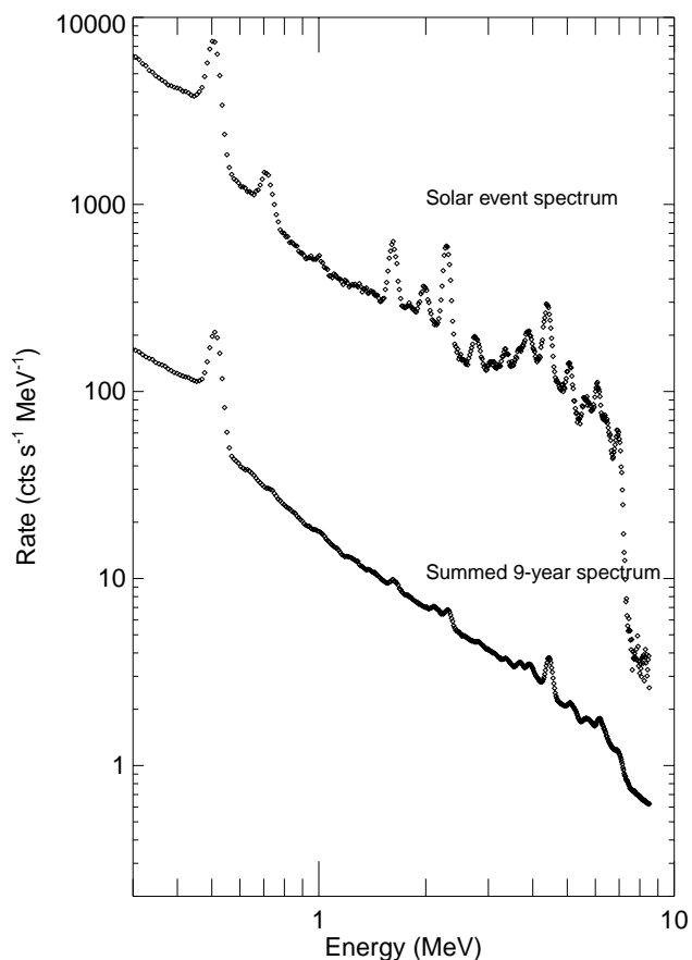
Figure 1: Comparison of the quiescent atmospheric spectrum, produced by cosmic rays observed over 9 years, with the spectrum excited by the 1989 October solar energetic particle event.
